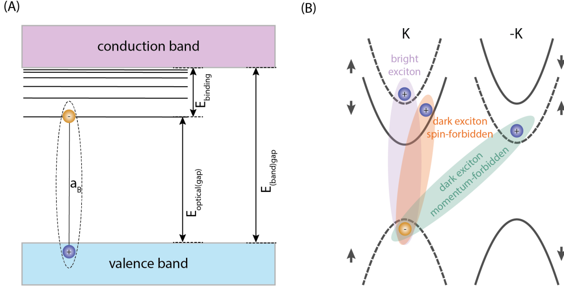
Figure 2.4: (A) An illustration of the general energy configuration for excitons as mid-gap states in semiconductors. (B) An illustration of the different kinds of exciton species possible within the TMDs. Here, we ignore the lower valence band due to the energy discrepancy between the two bands ( >100 meV). Excitations originating with a hole in the lower valence band make up the B series of excitons in TMDs. Panel (A) is adapted with modification from Ref. [132].
