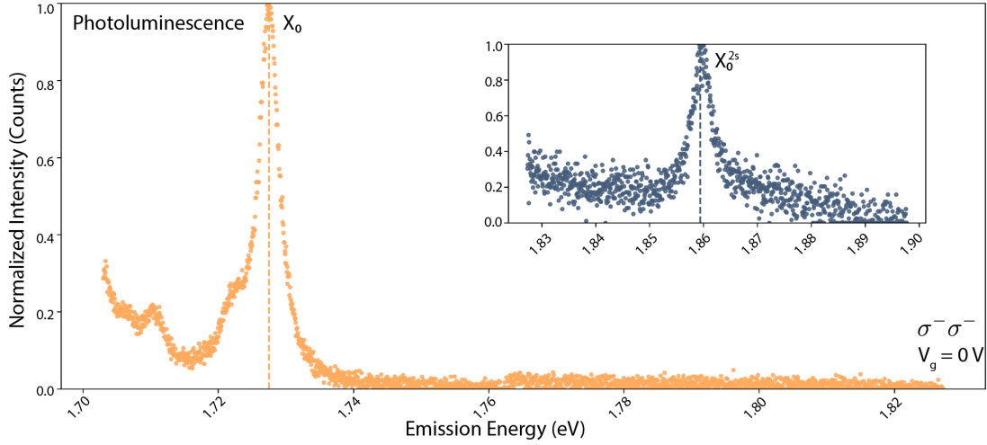
Figure 6.8: Comparison of the PL signal for X_0 and X_0^{2s} for PL measurements with E_{\text{ex}} = 2.33 eV. Both spectra are normalized to the emission maximum of their respective exciton lines and the spectral position of each is marked with a dashed line.
