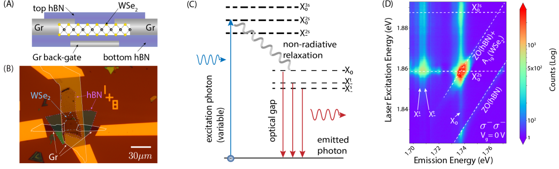
Figure 6.1: (A) Schematic of the hBN encapsulated WSe 2 with graphite (Gr) back gate and electrodes. (B) Optical image of device after full fabrication. The compressed area in the center indicates the region of the sample that underwent nanosqueezing. (C) Schematic of the PLE process highlighting the higher n states (e.g. X_0^{2s} ) and emission monitored channels (e.g. X_0 , X_-^t , or X_-^s ). (D) \sigma^-\sigma^- PLE spectra taken at V_g = 0 V and sample temperature of <300 mK. The monitored emission channels are marked with arrows ( X_0 , X_-^t , and X_-^s ) [16, 181]. Two Raman modes are identified as diagonal dashed lines (ZO(hBN) and ZO(hBN)+A 1g (WSe 2 )), see SM [119, 121]. The resonances of the excited states are marked with horizontal dashed lines ( X_0^{2s} , X_0^{3s} ) [292].
