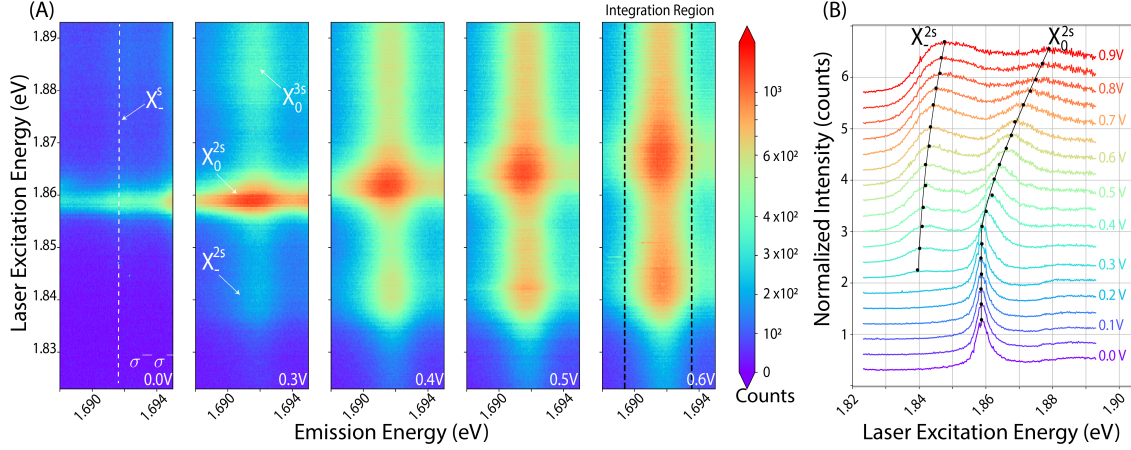
Figure 6.10: Comparison of the PL signal for X_0 , X_-^{2s} , and X_0^{2s} for PL measurements with gate dependence. All spectra have been normalized to the same color bar with the scale factor highlighted in the top left of each plot. (A) The 1s exciton species were collected while the sample was illuminated with an excitation energy of 1.95 eV (633 nm). (B/C) The 2s exciton species were collected while the sample was illuminated with an excitation energy of 2.33 eV. The sample was illuminated with linearly polarized light and the collection was polarization resolved for \sigma^- .
