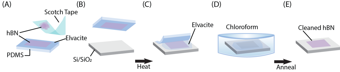
Figure 3.4: Panels (A)-(E) illustrate, in order, the process for producing one layer of an encapsulated stack using the “drop-down” method. The method must be repeated with each layer of the stack.
