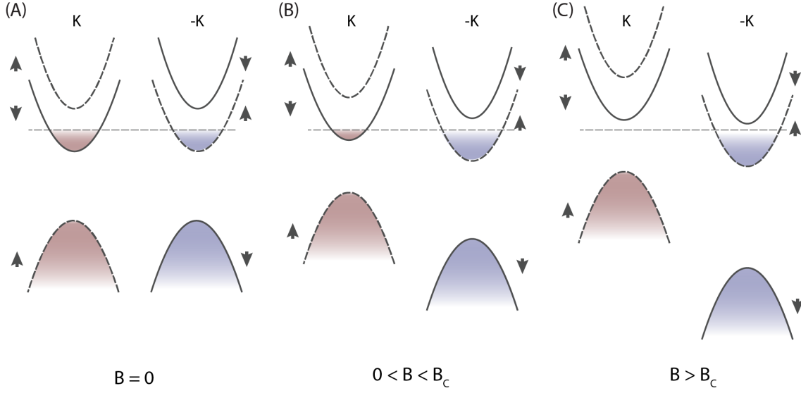
Figure 5.4: Stages of carrier polarization under applied magnetic field (A) B = 0\text{T} and there are an equal number of carriers in each valley, (B) 0 < B < B_C and there is a carrier population imbalance between the two valleys, but both valleys have excess carriers, (C) B > B_C and all of the excess carriers now resides in just one of the two valleys. If we reversed the field, the occupation sequence would flip valleys as |B| increased. In all panels, the dashed horizontal line indicates where the Fermi energy E_F is in the sample.
