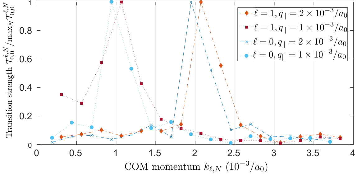
Figure 8.2: For the 1s transition, we plot the transition strength \mathcal{T}_{0,0}^{\ell,N} into the different COM modes k_{\ell,N} , normalized by the peak value \max_N(\mathcal{T}_{0,0}^{\ell,N}) , for illumination with \ell = 0 and \ell = 1 Bessel beams. The peak is obtained for the best match between COM momentum k_{\ell,N} and in-plane photon momentum, q_{\parallel} = 10^{-3}a_0^{-1} .
