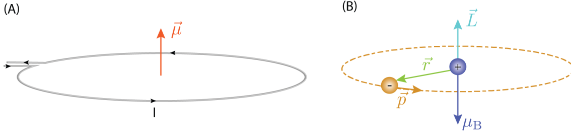
Figure B.1: (A) Current carrying loop with magnetic moment \vec{\mu} and (B) the Bohr magneton ( \mu_B ) arising from the Bohr model of the hydrogen atom.
