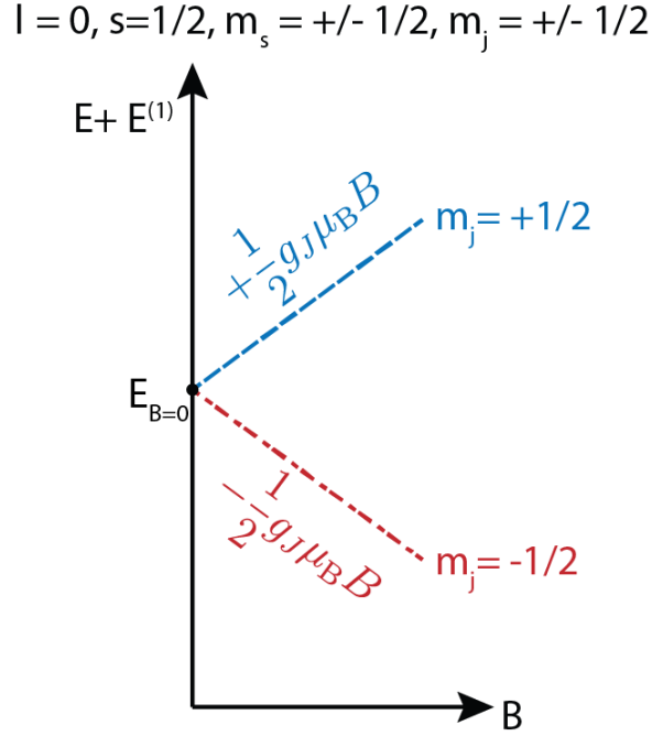
Figure 5.1: Detailed illustration of the Zeeman effect in hydrogen for the ground state.
