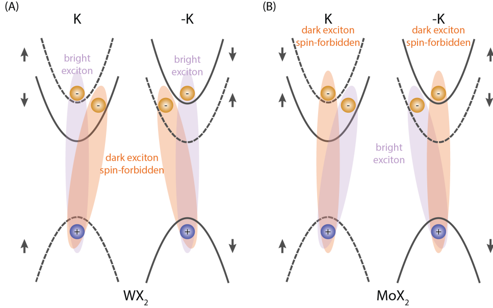
Figure 2.6: Comparison of the bright/dark states in (A) W-based TMDs and (B) Mo-based TMDs. Due to d-orbital chemistry in the W-based TMDs the conduction band orbitals are inverted compared with the conduction band in Mo-based TMDs.
