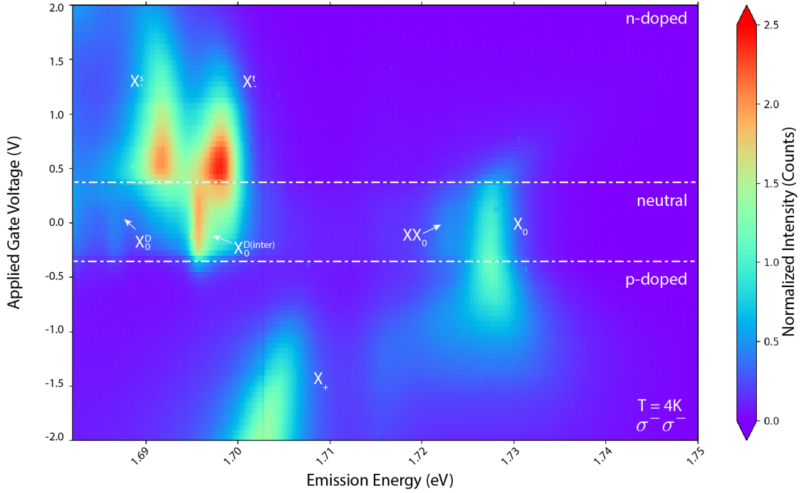
Figure 4.3: PL measurement of the gate response in a representative sample of WSe 2 .
