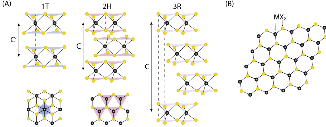
Figure 2.1: (A) An illustration of stacking periodicity and coordination of the different TMD polytypes. C is the unit repeat in the \hat{z} direction. In this labeling scheme, the number denotes the monolayers in the unit cell and T, H, and R correspond to trigonal, hexagonal, and rhombohedral respectively [145]. (B) An illustration of a monolayer TMD lattice extracted from a 2H crystal from a top-down view. In both panels, the black atoms correspond to the transition metal atoms and the yellow atoms correspond to the chalcogen atoms. This figure is adapted with some modification from Ref. [137]
