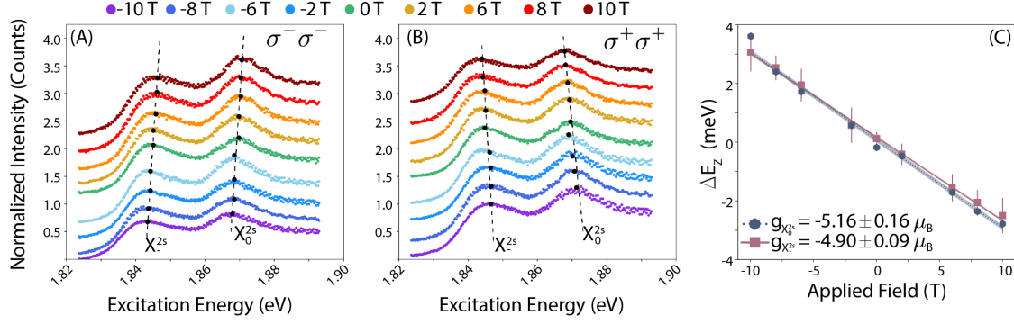
Figure 6.11: Vertical cross-sections in excitation energy as a function of field through the X_s^- emission channel for (A) (\sigma^- \sigma^-) and (B) (\sigma^+ \sigma^+) marked with the corresponding peak positions for the X_0^{2s} and X_-^{2s} excitons from fitting. (C) Extracted g -factor for X_0^{2s} and X_-^{2s} . The shaded regions in panel (C) on the fit line include the error in the extracted slope.
