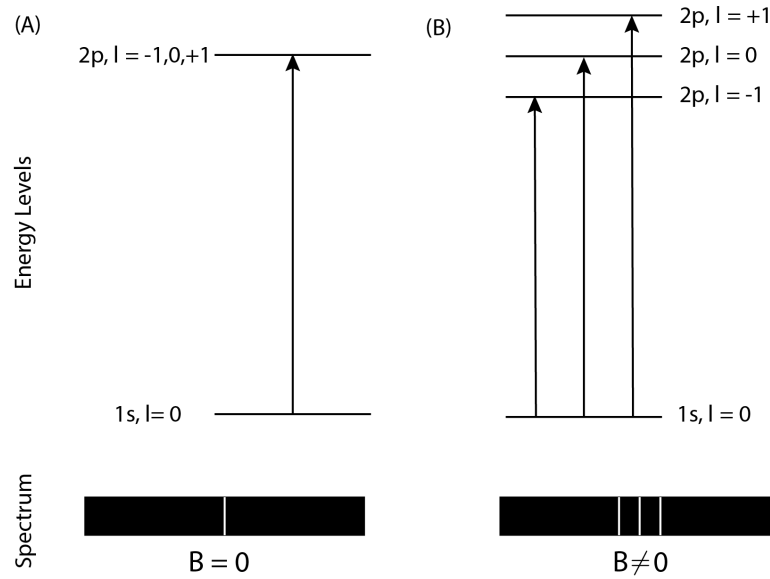
Figure 4.4: Visual representation of the effect of applying a magnetic field and observing the splitting of different angular momentum states (the Zeeman effect).
