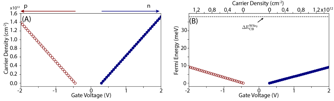
Figure 6.7: (A) Extracted carrier density as a function of applied gate voltage in a capacitive model (B) Calculated Fermi energy from carrier dependence with gate voltage. The energy corresponding to the conduction band spin-splitting is noted.
