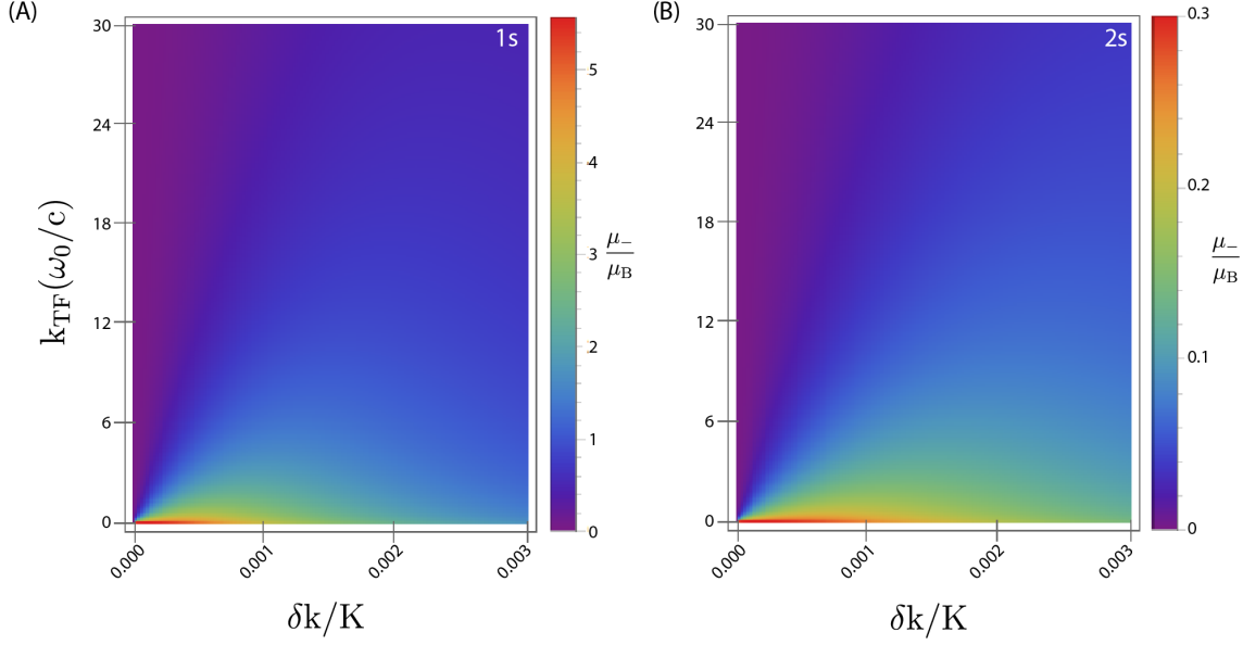
Figure 6.14: Valley orbital magnetic moment for a charged exciton as a function of the center of mass k from the valley center K for different carrier concentrations (expressed in k_{\text{TF}} ) for (A) 1s charged exciton and (B) 2s charged exciton. Note the difference in scale for the resulting magnetic moment in each panel.
