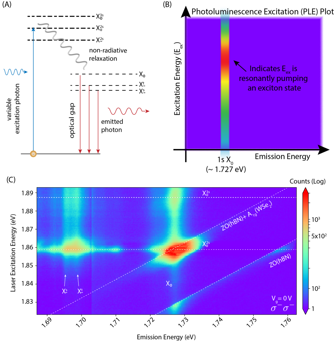
Figure 4.2: Panel (A) shows the diagram representing the energetics of the photoluminescence excitation (PLE) process. It is similar to PL, but the excitation wavelength is varied in this case. Panel (B) shows a diagram of the expected PLE plot, indicating emission to the lowest state from a resonantly excited state, and panel (C) shows a typical PLE emission spectra for WSe_2 in the 2s energy region.
