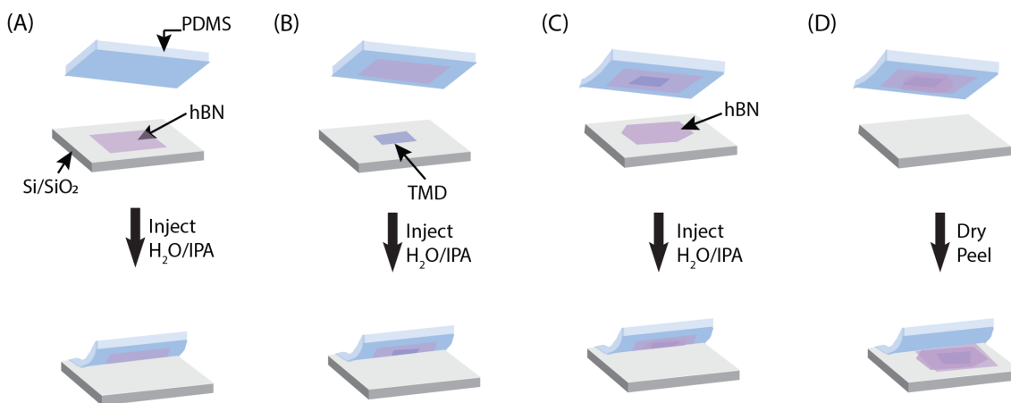
Figure 3.6: Capillary-action assisted pickup of a TMD stack using a combination of liquid injection and dry transfer.
