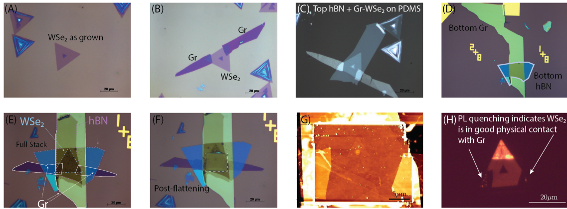
Figure 6.5: More detailed images from the fabrication process showing (A) the as-grown \text{WSe}_2 , (B)/(C)/(D) graphite leads/gate, (E) full hBN encapsulation, (F) fully encapsulated stack after nano-squeegee process (highlighted with dashed box), (G) an AFM image of the nano-squeegee region highlighting the removal of interlayer impurities from the stacking process, and (H) a PL image of the \text{WSe}_2 monolayer and graphite leads, with the quenching of emission at the contact points indicating good physical contact.
