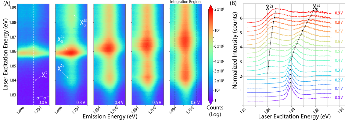
Figure 6.3: (A) PLE data with increasing n_e -doping while monitoring the X_t^- recombination channel ( \sigma^- \sigma^- ). (B) As in Fig. 6.2, the waterfall plot corresponds to vertical cross-sections from V_g = 0 - 0.9\text{ V} .
