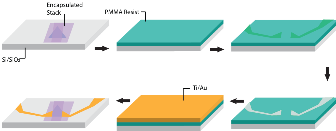
Figure 3.8: EBL process for defining electrical contacts on a sample.
