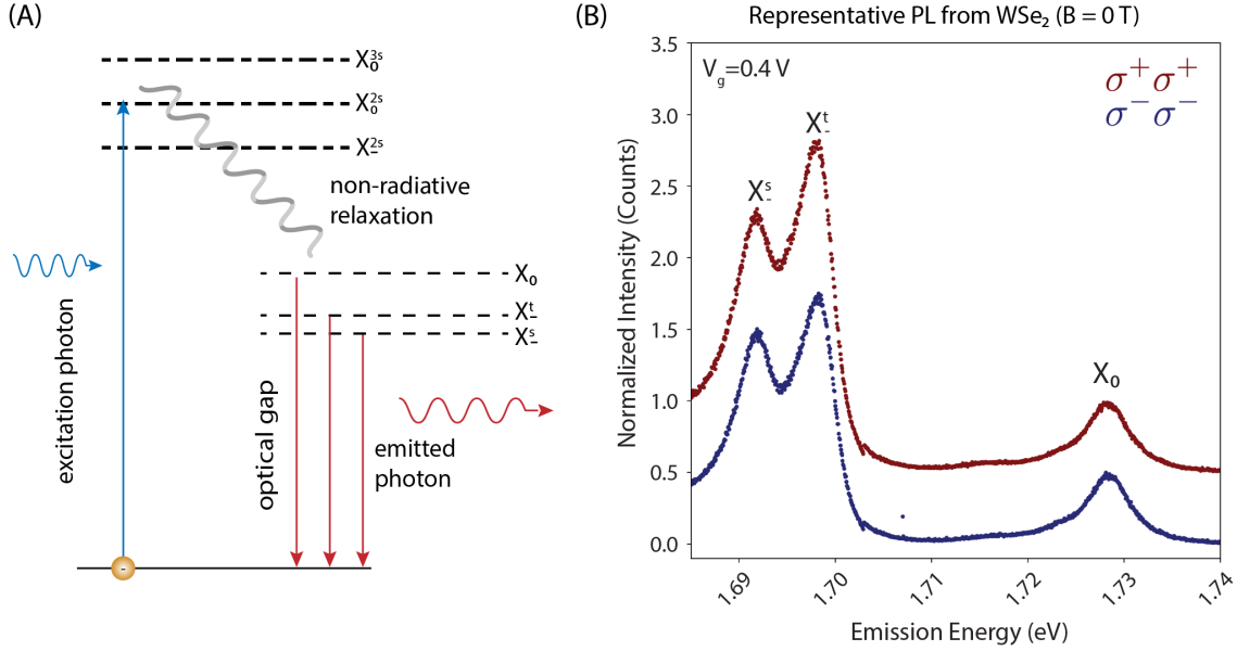
Figure 4.1: Panel (A) shows a diagram representing the energetics of the photoluminescence (PL) process and panel (B) shows a typical PL emission spectra for WSe 2 with labels denoting the different exciton species emission origins.
