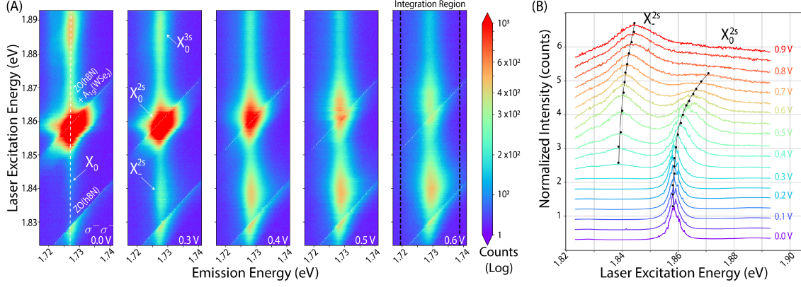
Figure 6.2: (A) PLE data with increasing n_e -doping while monitoring the X_0 recombination channel in the -K-valley ( \sigma^- \sigma^- ). (B) Waterfall plot of vertical cross-sections from V_g = 0 - 0.9 V. The integration region is annotated in panel (A). The counts were summed over the emission width for each excitation energy.
