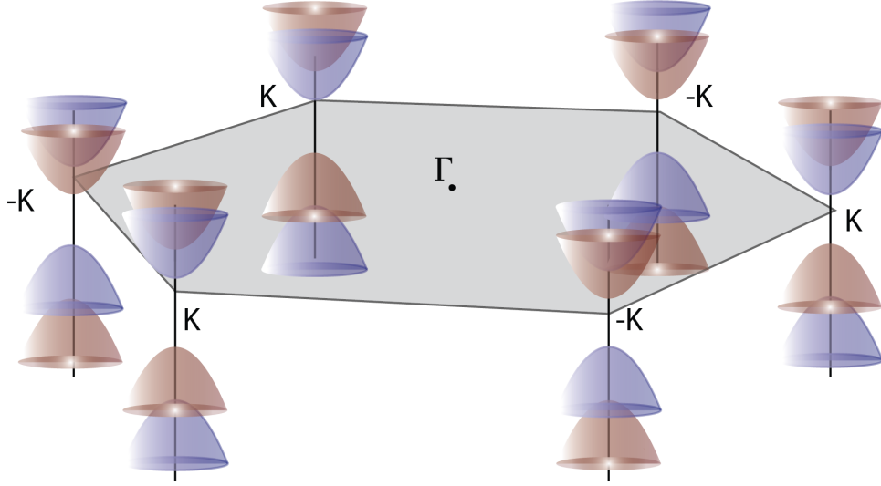
Figure 2.2: Transition metal dichalcogenide band structure schematic of the band edges showing the spin splitting of the valence band/conduction band at the \pm K valleys. The schematic is not to scale. The figure is derived from Reference [327].
