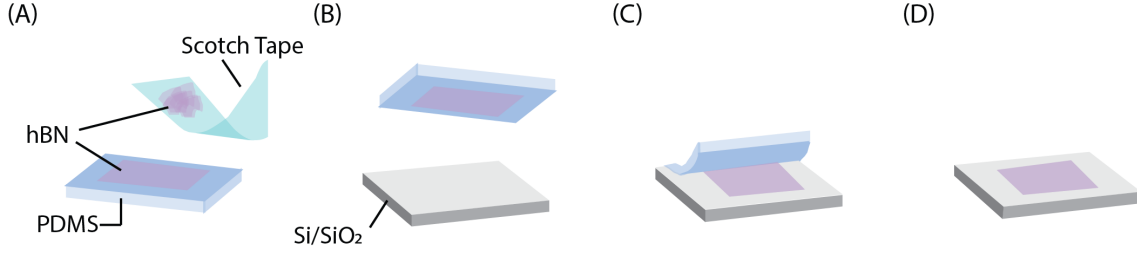
Figure 3.3: Panels (A)-(D) show chronologically the steps for creating one layer of a stack using viscoelastic stamping.
