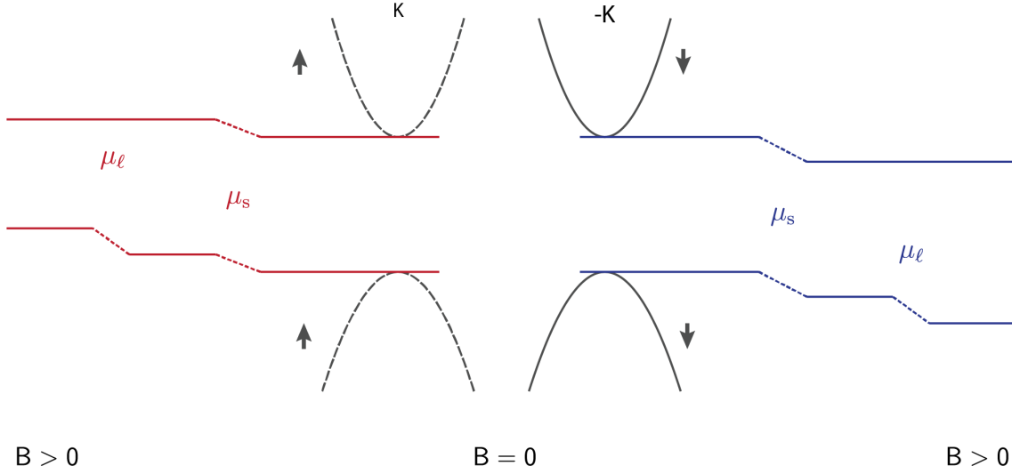
Figure 5.2: Zeeman splitting for excitons in TMDs in the single-particle model. Here, only the bands for the A series bright exciton are shown. Note that if the applied field was negative, we would expect the K-valley to blue shift and the -K-valley to red shift instead.
