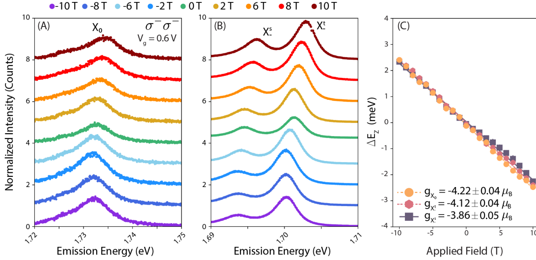
Figure 6.13: 1s PL spectra at V_g=0.6\text{V} for the (A) X_0 , (B) X_-^t/X_-^s . (C) Extracted g -factors from fitting PL as a function of field for X_0 , X_-^t , and X_-^s . For all measurements E_{\text{ex}}=1.92 eV
