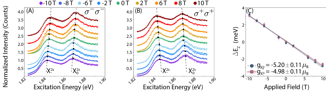
Figure 6.4: Vertical cross-sections from the X_t^ emission channel as a function of field for (A) (\sigma^- \sigma^-) and (B) (\sigma^+ \sigma^+) marked with the corresponding peak positions (black dots) for the X_0^{2s} and X_-^{2s} states from fitting with the dashed line serving as a guide to the eye. (C) Extracted g -factors for X_0^{2s} and X_-^{2s} states. The thickness of the fit line in panel (C) corresponds to the error in the fit.
