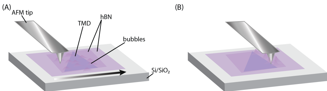
Figure 3.7: Panels (A) and (B) show the nano-squeegee process whereby the bubbles that can appear during encapsulation can be flattened out using the force of the AFM tip. Figure is adapted with some modification from Ref. [255].
