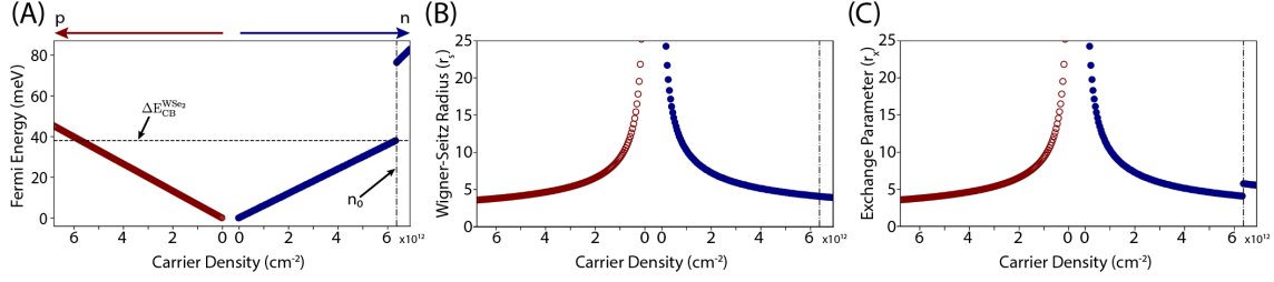
Figure 5.3: Illustration of the relationship between carrier density, Fermi energy, Wigner-Seitz radius, and exchange interaction strength in TMDs. (A) Calculated Fermi energy from carrier dependence with gate voltage. The Fermi energy needed to cross from the lower to upper conduction band is marked, as is the associated density for that transition. (B) Extracted Wigner-Seitz radius for the sample as a function of carrier density. The threshold for crossing into the upper conduction band is marked. (C) The calculated exchange parameter, highlighting the effect of doubling the spin-valley degeneracy upon crossing into the upper conduction band.
