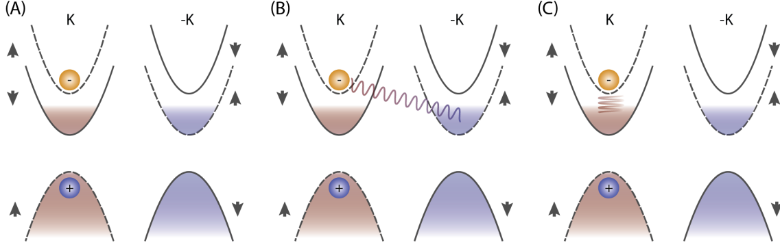
Figure 2.12: (A) Repulsive polaron, (B) intervalley attractive polaron, and (C) intravalley attractive polaron in WSe 2 . Figure is adapted with some modification from Ref. [91].
