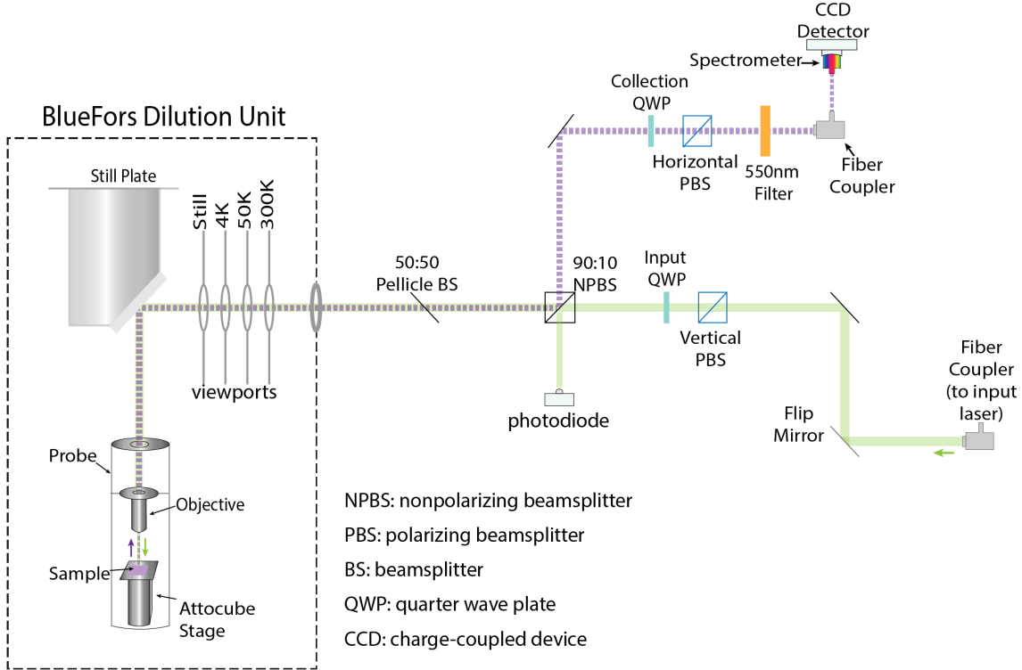
Figure 4.5: Optical diagram depicting the excitation and emission collection scheme used for photoluminescence and photoluminescence excitation measurements. Figure is taken from our own work [266].
