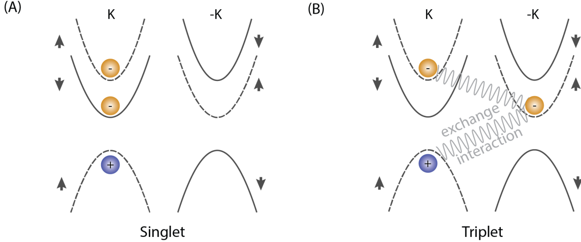
Figure 2.9: Focusing just on K-valley trions (A) shows the intravalley singlet trion and (B) shows the intervalley triplet trion and its associated exchange interaction. It should also be noted the bands are structured in this diagram for WX_2 systems. All trions here are negative and a similar configuration to both (A) and (B) can be produced in the -K valley.
