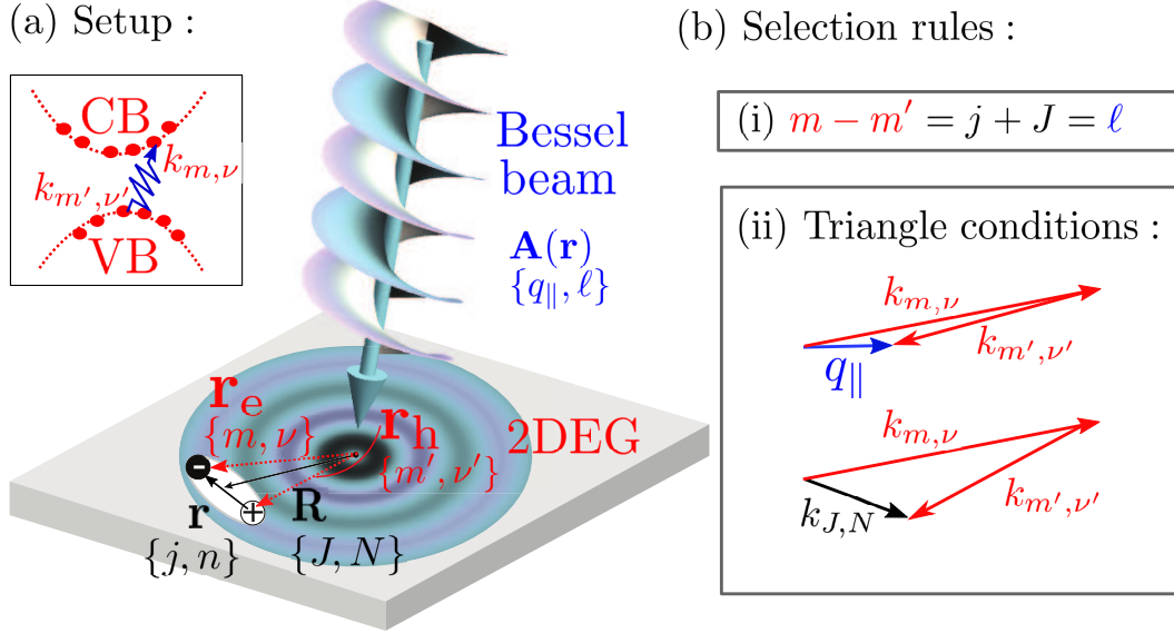
Figure 8.1: (a) A Bessel light beam \mathbf{A} with photon momentum/angular momentum (q_{||}, \ell) creates an electron-hole pair in a 2D electron gas (2DEG). The electron [hole] is characterized by quantum numbers (m, \nu) [ (m', \nu') ] for angular momentum/ momentum. The pair can form a bound state, and the degrees of freedom of such an exciton are the center-of-mass motion, characterized by angular momentum/ momentum quantum numbers (J, N) , and the relative motion, characterized by quantum numbers (j, n) for angular momentum and energy. (b) The selection rules for optical transitions and exciton formation reflect (i) conservation of angular momentum, and (ii) conservation of linear momentum, reflected by the illustrated triangle conditions.
