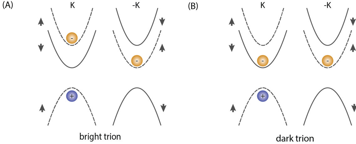
Figure 2.10: (A) the formation of a bright trion in a TMD, denoting the positions in the bands of the carriers. (B) the formation of a dark trion in a TMD, denoting the positions in the bands of the carriers. It should also be noted the bands are structured in this diagram for WX_2 systems.
