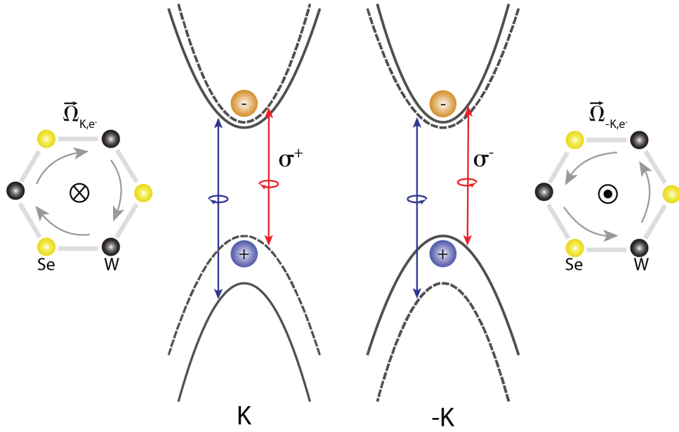
Figure 2.3: Valley- and spin-selection rules in TMDs the polarization to excite each valley is denoted ( \sigma^{\pm} ) and the dipole allowed transitions are denoted with blue (higher energy, “B” excitons) and red (lower energy, “A” excitons) transitions. Spin up is denoted with the dashed line and spin down is denoted with the solid line. On the outside the Berry curvature in each valley is depicted. This figure is derived with modification from Ref. [198]
