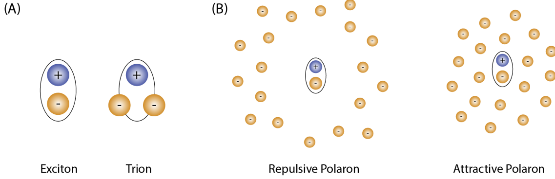
Figure 2.11: (A) Neutral (exciton) and charged (trion) single-particle species and their (B) many-body interpretations, the repulsive and attractive polarons.
