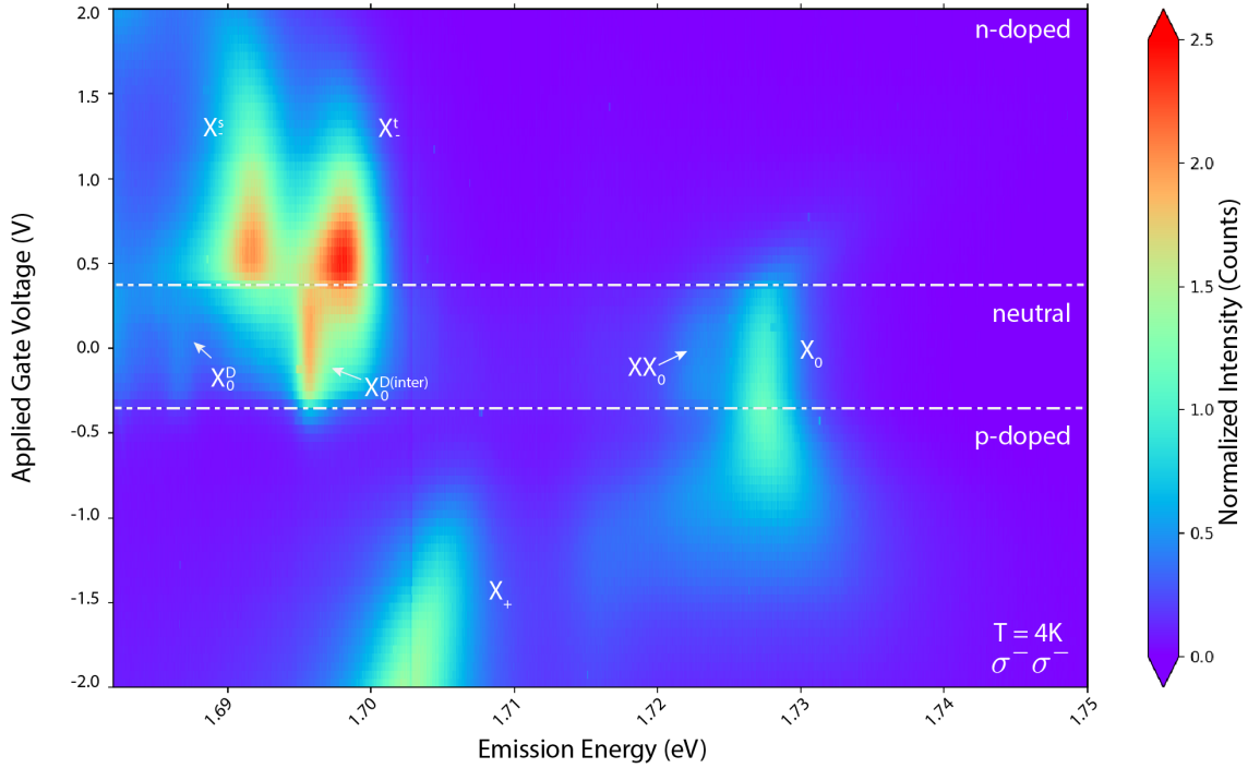
Figure 6.6: PL of the 1s exciton species as a function of gate voltage. Here, there are three regions marked based on their charge character: n -doped, neutral, and p -doped. Exciton species are noted. Data collected while the sample was illuminated with an excitation energy of 1.95 eV.
