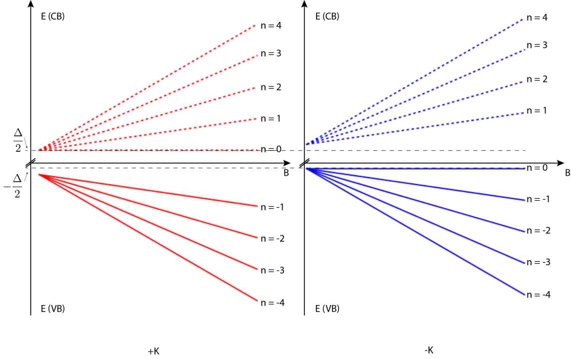
Figure B.2: Valley-resolved LLs in TMDs resulting from a real magnetic field. Note that the energy axis is split so as to showcase both the valence and conduction bands at the same time.
