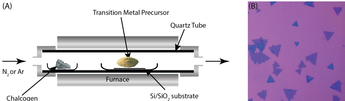
Figure 3.2: (A) Setup of the tube furnace for depositing monolayers of TMDs using the chemical vapor deposition (CVD) process. The examples materials here are raw selenium (Se) for the chalcogen and tungsten trioxide ( \text{WO}_3 ) for the transition metal precursor, since our experiments focus on \text{WSe}_2 . (B) CVD grown \text{WSe}_2 monolayers on \text{SiO}_2 . The natural termination of the monolayer into a triangle is due to the underlying crystal structure and a typical size is \sim 30\text{-}40\ \mu\text{m} per side of the triangle.
