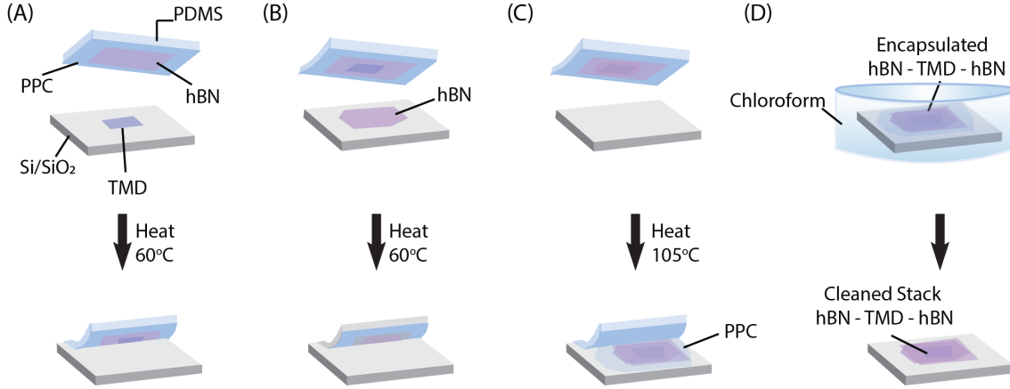
Figure 3.5: Dry pickup method for sequentially picking up 2D materials to form heterostructures with PPC.
