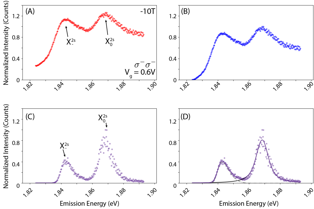
Figure 6.12: (A) Raw Vertical cross-sections of the X^-_{2s} emission channel at -10T and 0.6V. The data has been normalized to the maxima of the extracted spectra. (B) The same data after the lowest value in the spectra has been subtracted from all points and data has been renormalized to the maxima. (C) Power sharpening of the spectra in panel (B). (D) Peak fitting of the X^0_{2s} and X^-_{2s} . The denoted input/output polarizations, magnetic field, and gate voltage in panel (A) are the same for all panels.
