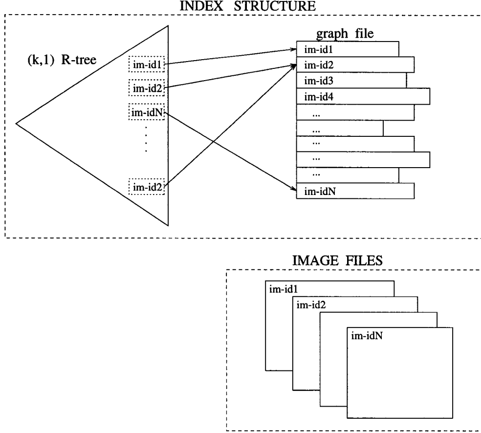
Figure 7: Proposed file structure.
