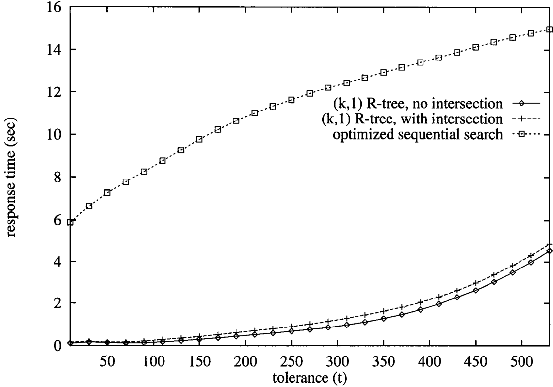
Figure 10: Average retrieval response time as a function of the tolerance ( t ) for (k,2) queries corresponding to (a) search on a (k,1) R-tree utilizing one (k,1) sub-query, (b) search on a (k,1) R-tree utilizing both (k,1) sub-queries and (c) optimized sequential scan of the database.
