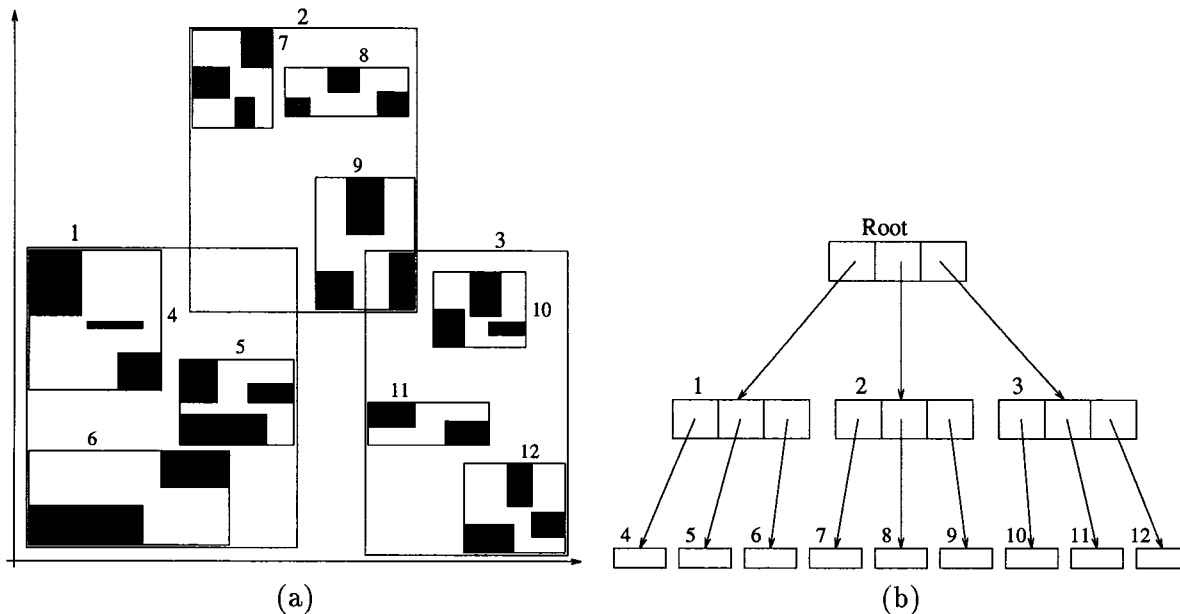
Figure 4: Data (dark rectangles) organized in an R-tree (a), and the resulting tree on disk (b).
