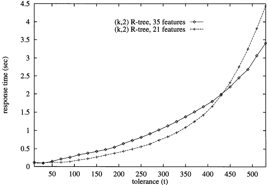
Figure 14: Average retrieval response time as a function of the tolerance ( t ) for (k,2) queries corresponding to search on a (k,2) R-tree utilizing (a) all 35 attributes and (b) 21 attributes.
