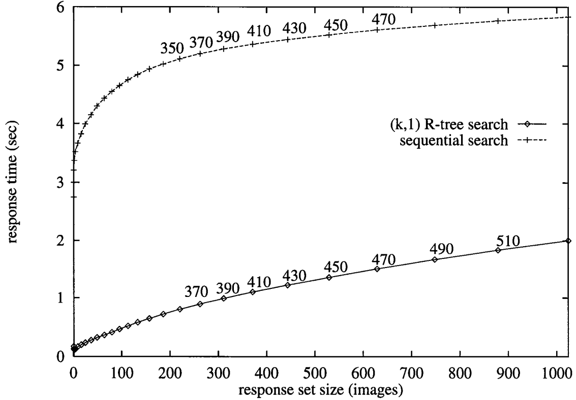
Figure 9: Average retrieval response time as a function of the average retrieval response set size for (k,1) queries. The labels denote the corresponding values of the tolerance ( t ).
