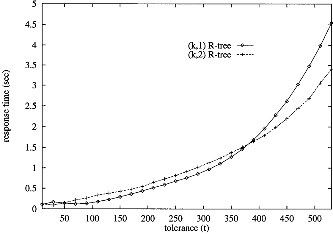
Figure 13: Average retrieval response time as a function of the tolerance ( t ) for (k,2) queries corresponding to search on (a) a (k,1) R-tree and (b) a (k,2) R-tree.
