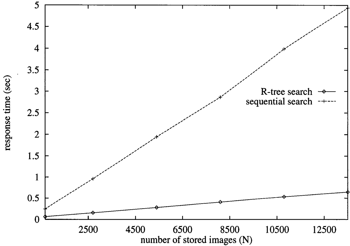
Figure 11: Average retrieval response time corresponding to a fixed value of the tolerance ( t = 310 ) as a function of the number of images ( N ) stored in the database.
