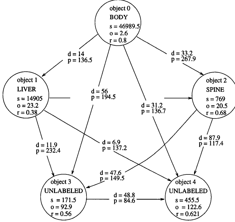
Figure 6: Attributed graph representing the content of the example image of Figure 5.
