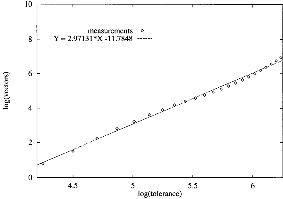
Figure 15: Logarithm of the number of qualifying vectors as a function of the logarithm of the tolerance t for (k,1) queries.
