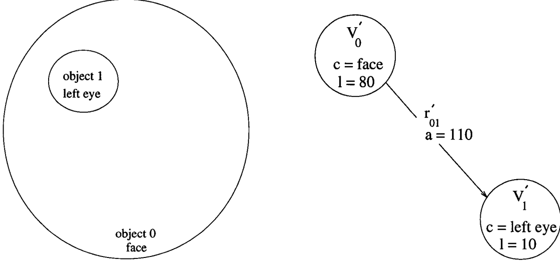
Figure 2: Example query image (left) and its corresponding ARG (right).
