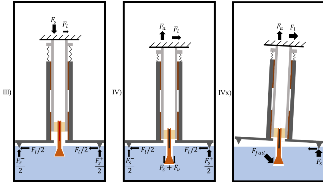
Figure 62: Illustrated concept of operation states III, IV, and IVx of the long thermal pick end effector.
