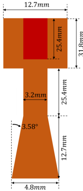
Figure 17: Illustration of thermal pick (A) showing relevant dimensions. Not to scale.
