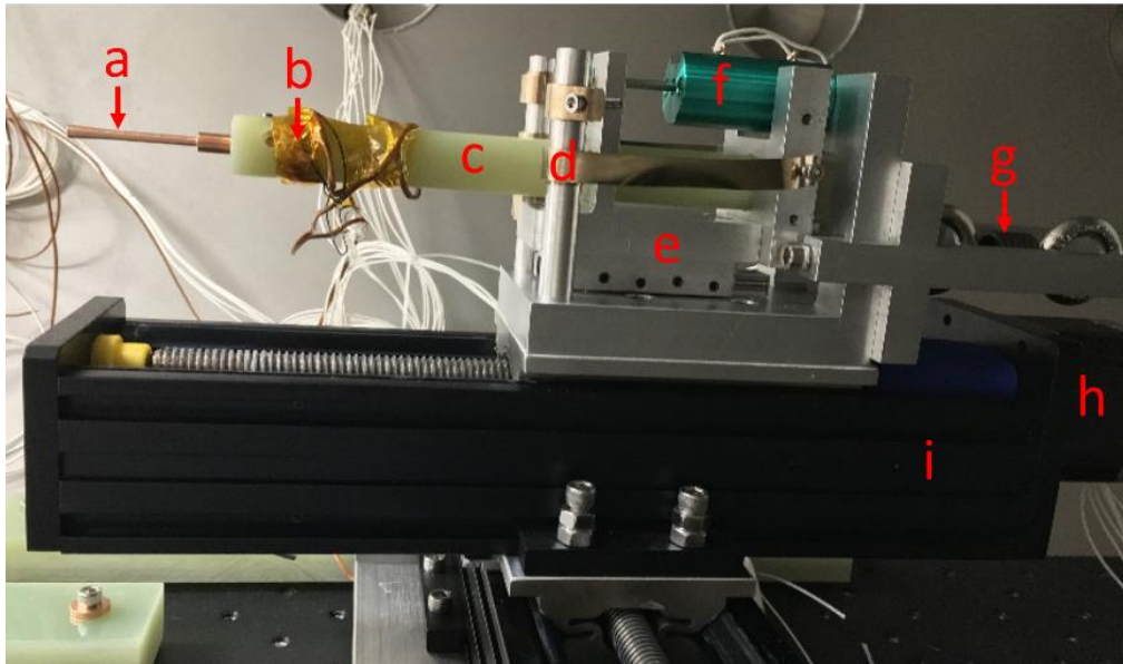
Figure 22: Water ice test rig side view. Shown are the thermal pick (a), thermocouple location (b), G-10 thermal insulation (c), constant force springs (d), crossed roller bearing (e), linear potentiometer (f), extension spring (g), stepper motors (h), and positioning slides (i).
