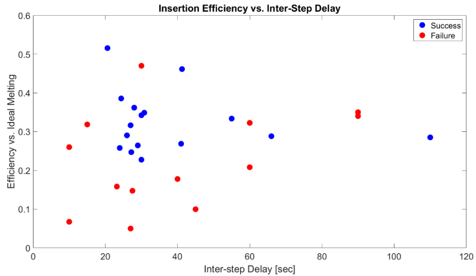
Figure 33: Efficiency relative to ideal melting vs. inter-step delay for all water ice insertion tests.
