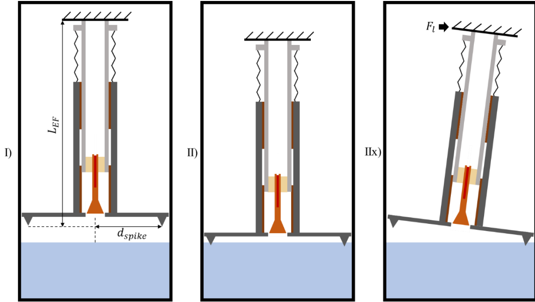
Figure 61: Illustrated concept of operation states I, II, and IIx of the long thermal pick end effector.
