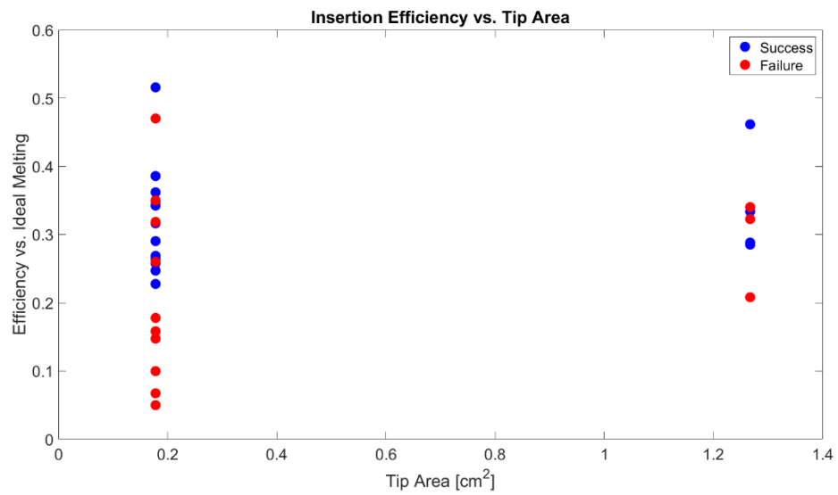
Figure 35: Efficiency relative to ideal melting vs. tip area for all water ice insertion tests.
