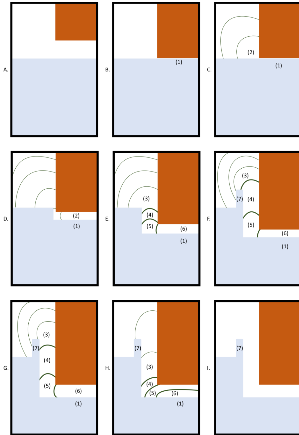
Figure 28: Illustration of the insertion process showing (1) conduction into the ice, (2) gaseous water, (3) ice and gaseous water, (4) triple phase water, (5) liquid water and gaseous water, (6) liquid water, and (7) the formation lip. Lines of constant pressure shown with thickened lines indicating phase change boundaries, ice is shown in light blue, and thermal pick shown in brown.
