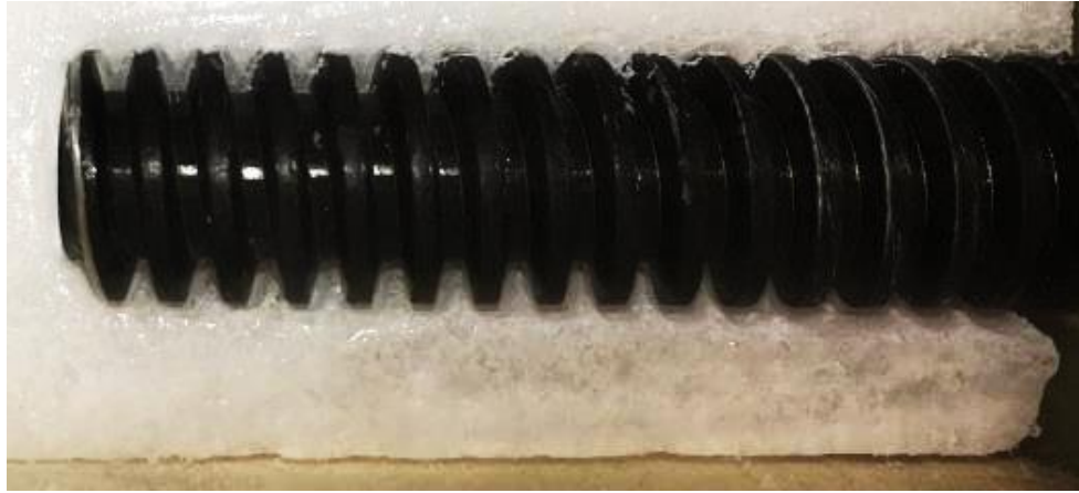
Figure 6: Cross cut of threaded ice borehole and thermal pick (f). Thread quality degrades towards the surface of the ice due to thermal erosion.
