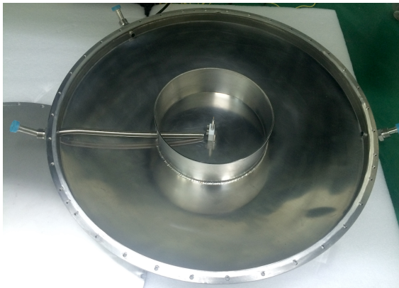
Figure 3.10: The internal structure of the overflow chamber. A level meter in the middle of the chamber. The tube on the left is for liquid xenon out. The other two are for pressure equalizing and overflow-in.
