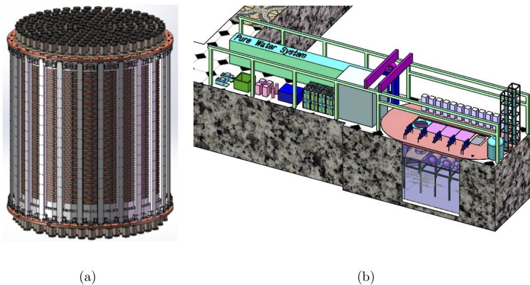
Figure 5.1: A diagram for PandaX-4T TPC (a) and preliminary layout of the PandaX-4T experiment in Hall-B (b).
