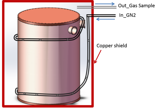
Pipes for flushing N2 between the OV and copper shield
