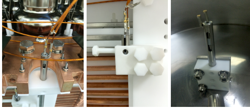
Figure 3.16: The long level meter (left), one of the three short ones (middle), and the overflow chamber one (right) in the PandaX-II detector. A PTFE filler can be seen in the middle of the one in the overflow chamber.
