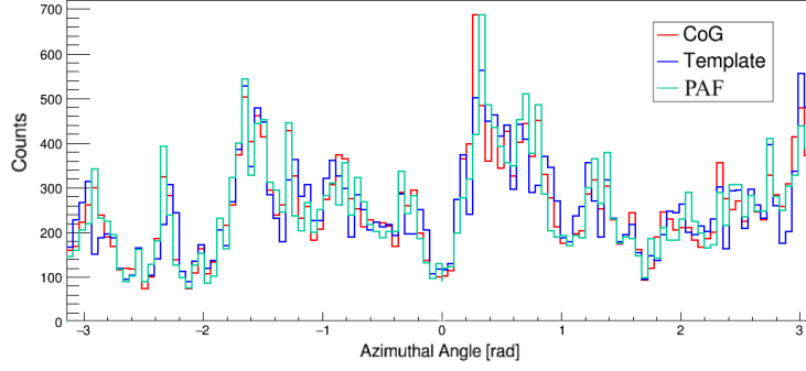
Figure 4.17: The azimuthal distribution of ^{210}\text{Po} \alpha events using different reconstruction algorithms.
