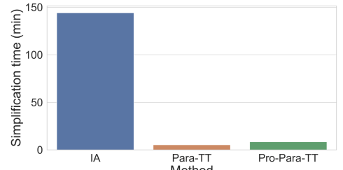
(b) Simplification time
