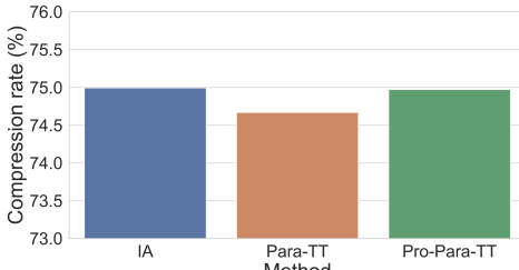
(a) Compression rate
