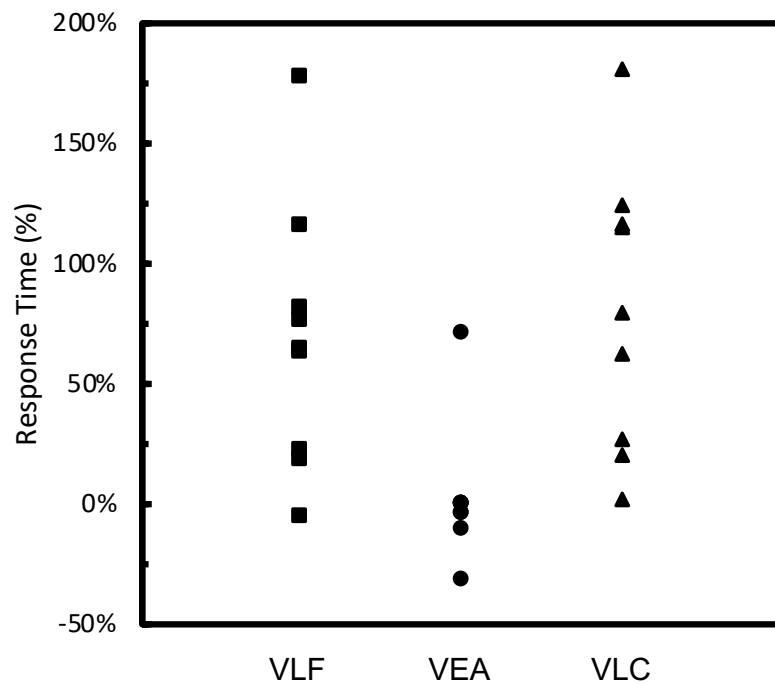
Figure 4.3: Total comparison of response times between ASDs and Whittaker photoelectric detector. Comparison in response time is presented as a percent difference to the Whittaker detector. Positive percentages indicate the VESDA system alarmed before the Whittaker while negative percentages indicate the VESDA system alarmed after the Whittaker.
