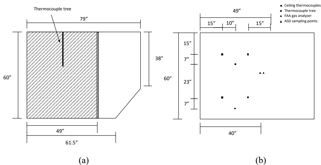
Figure 3.3: (a) Front view of ULD with shaded Plexiglas door. (b) Top view of ULD.
