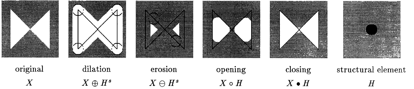
Figure 3: Original image (left column) and dilation, erosion, opening, closing, and structural element.
