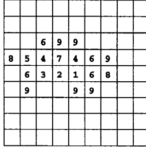
Figure 1: Lattice at t = 9 . The infection time of each infected cell is marked.
