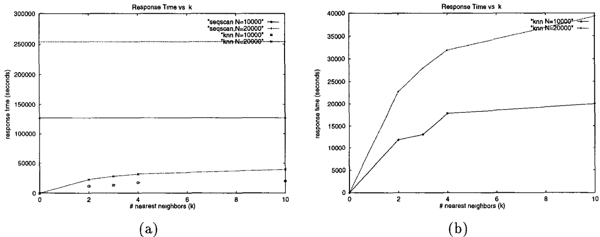
Figure 9: Response time vs. k for N = 10,000 and N = 20,000 (a) with seq. scanning (b) without seq. scanning
