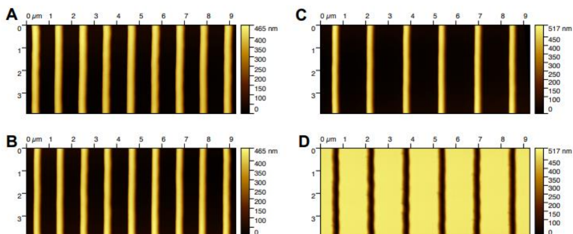
Figure 2.3 AFMs of 1- \mu m-spaced master (A) and replica (B) ridges, and 1.5- \mu m-spaced replica ridges (C) and grooves (D). Reprinted with permission from reference 142.
