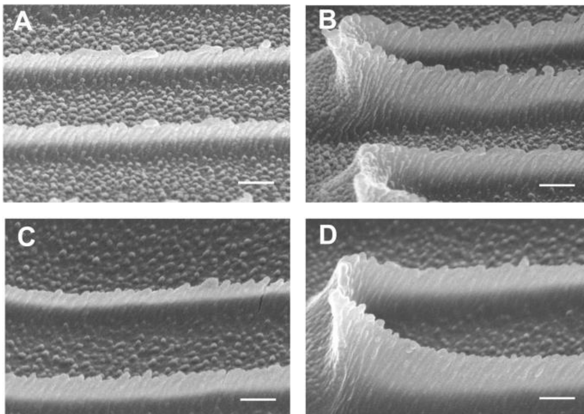
Figure 2.4. Replication of nanoglass. SEM images of the master (A,B) and replica (C,D) nanoglass. Scale bars, 200 nm. Reprinted with permission from reference 142.
