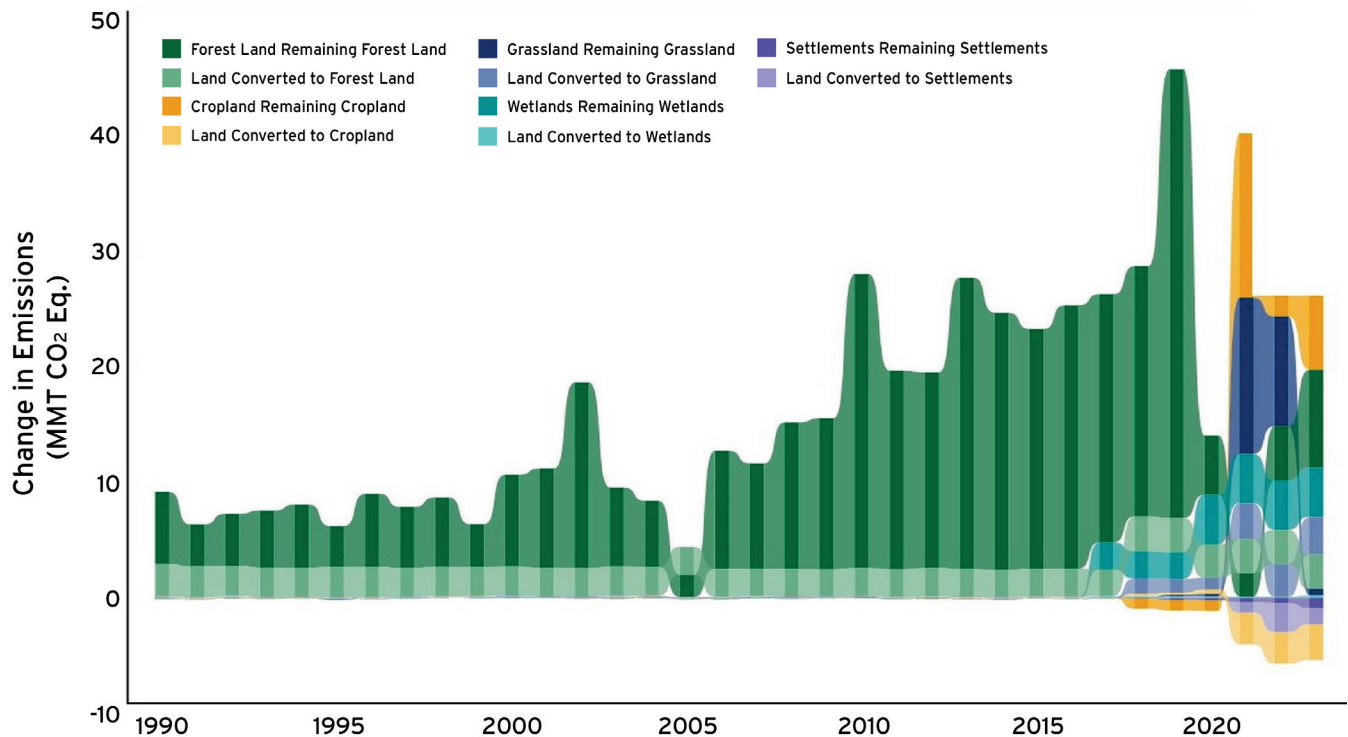
Figure 9-7: Impacts from Recalculations in the LULUCF Sector
