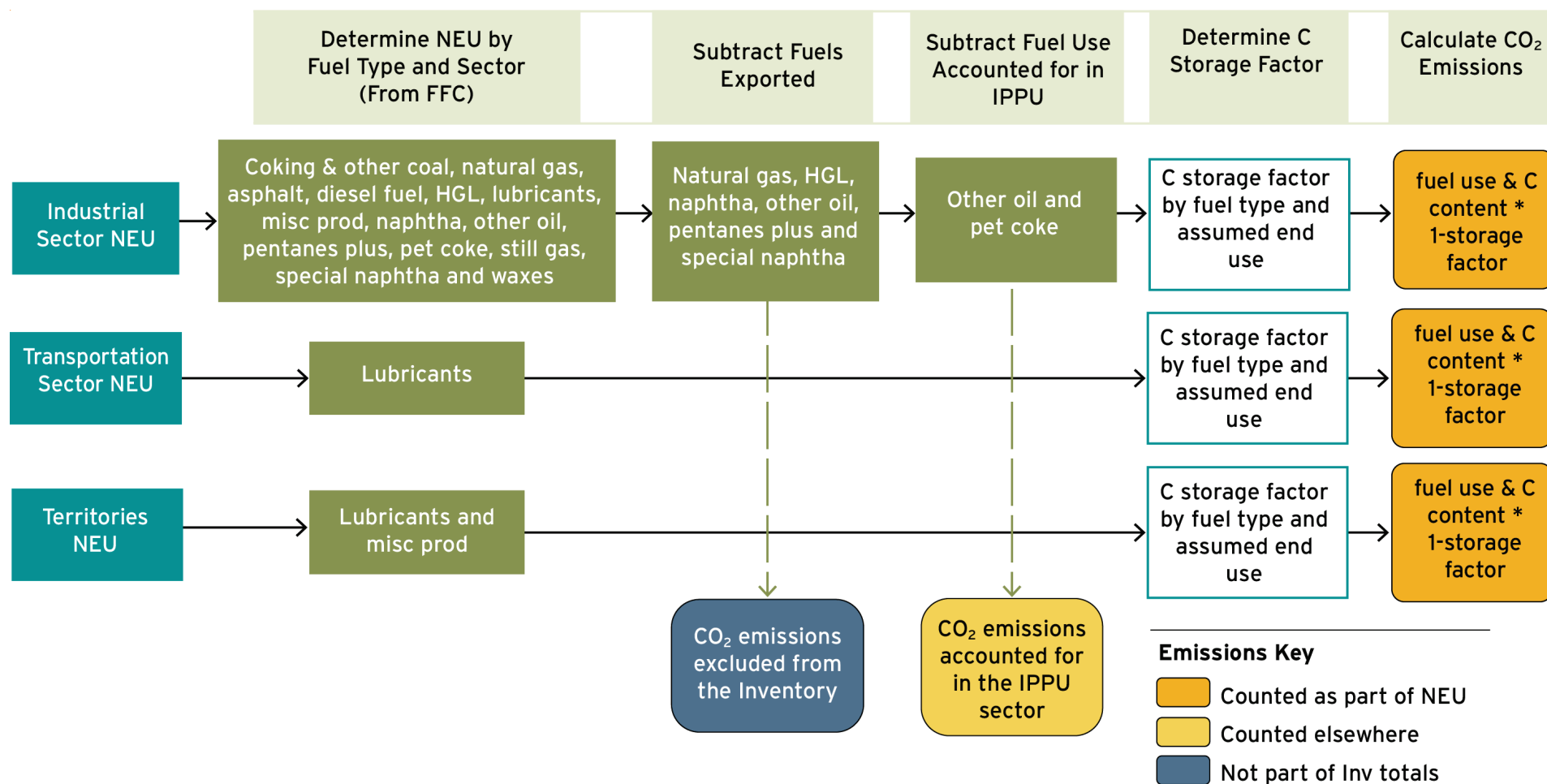
Figure 3-15: Approach for Calculating NEU Emission Estimates
