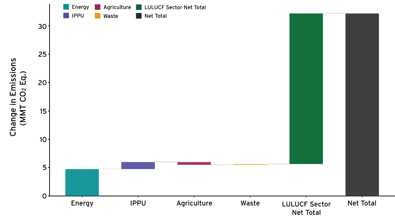
Figure 9-3: Impacts from Recalculation by Sector on 2023 Net Emissions (Absolute Change)
