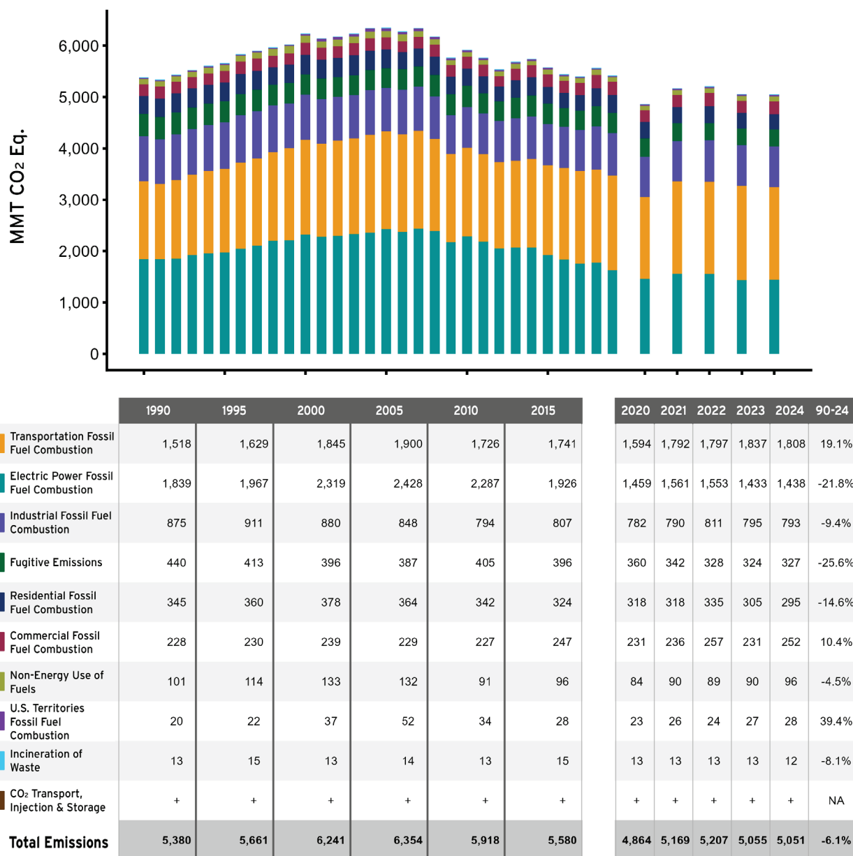
Figure 2-5: Trends in Energy Sector Greenhouse Gas Sources
