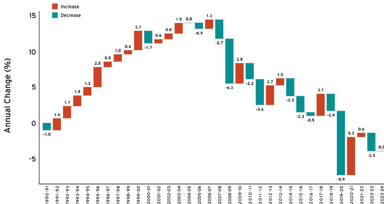
Figure 2-2: Annual Percent Change in U.S. Gross Emissions
