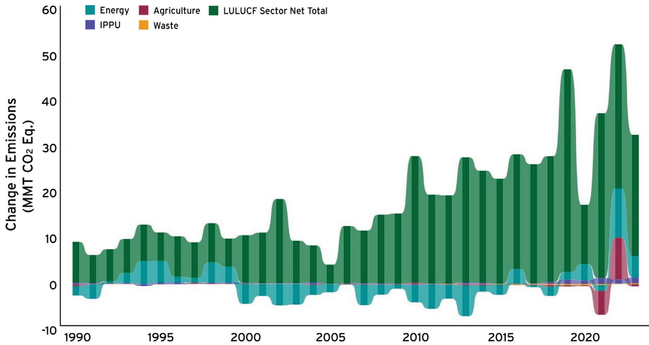
Figure 9-5: Impacts from Recalculation by Sector on Net Emissions Over Time
