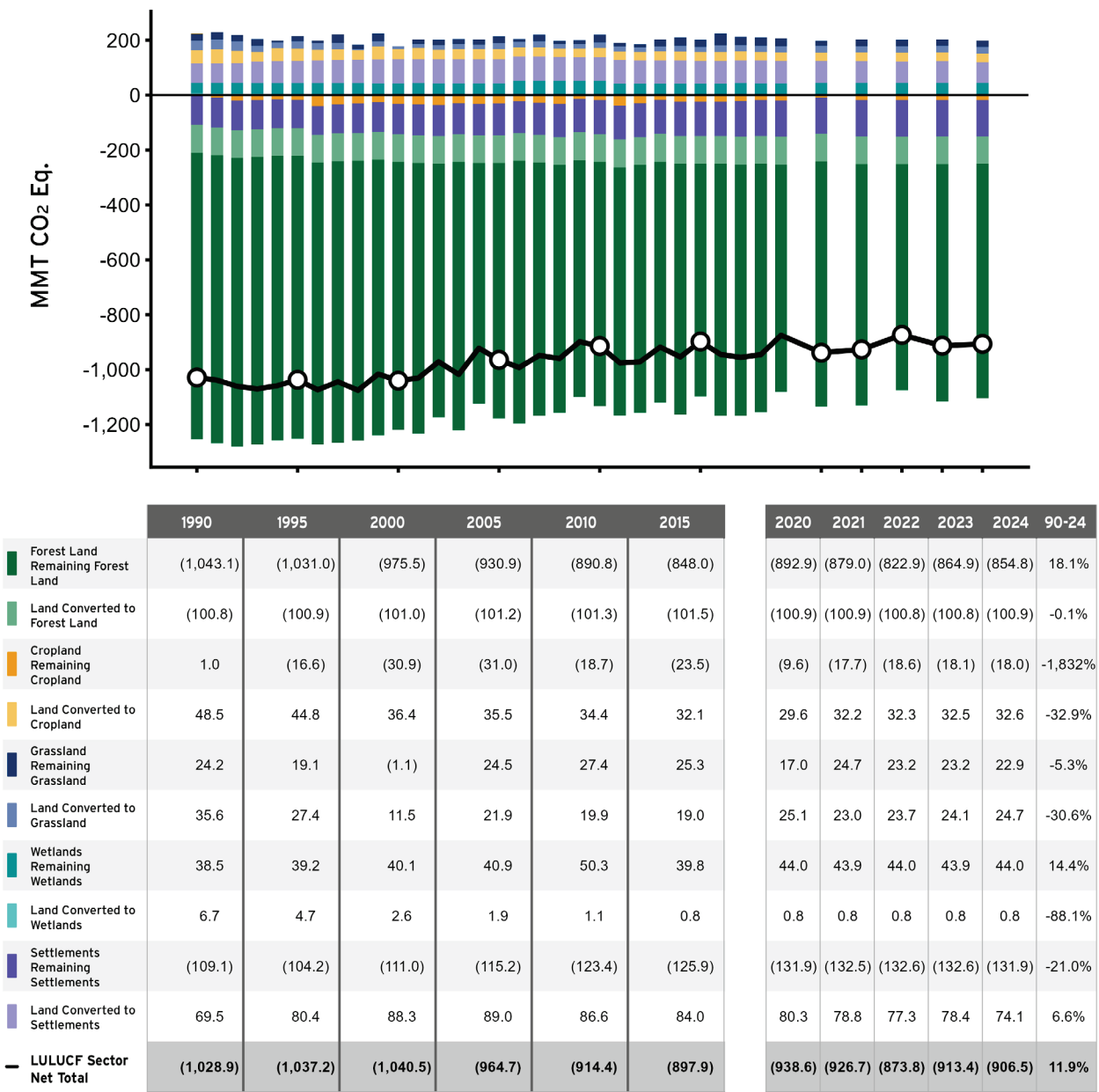
Figure 2-8: Trends in LULUCF Sector Emissions and Removals
