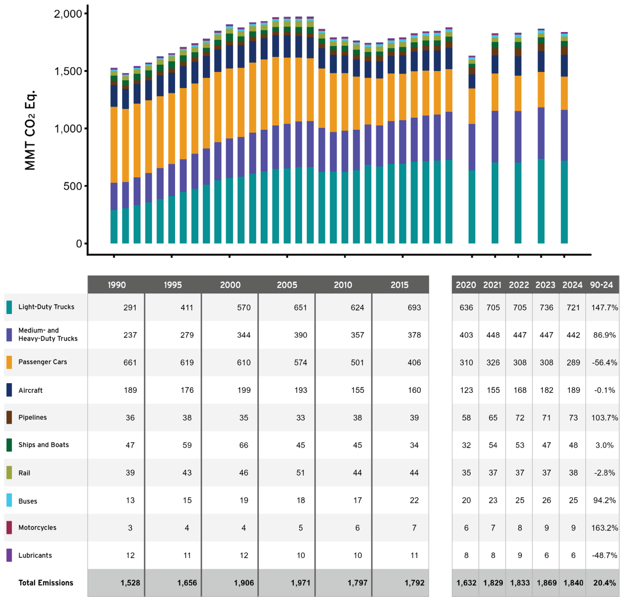
Figure 2-12: Trends in Transportation Sector by Mode
