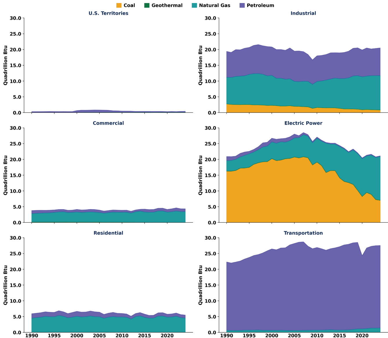
Figure 3-5: Fuel Use by End-Use Sector
