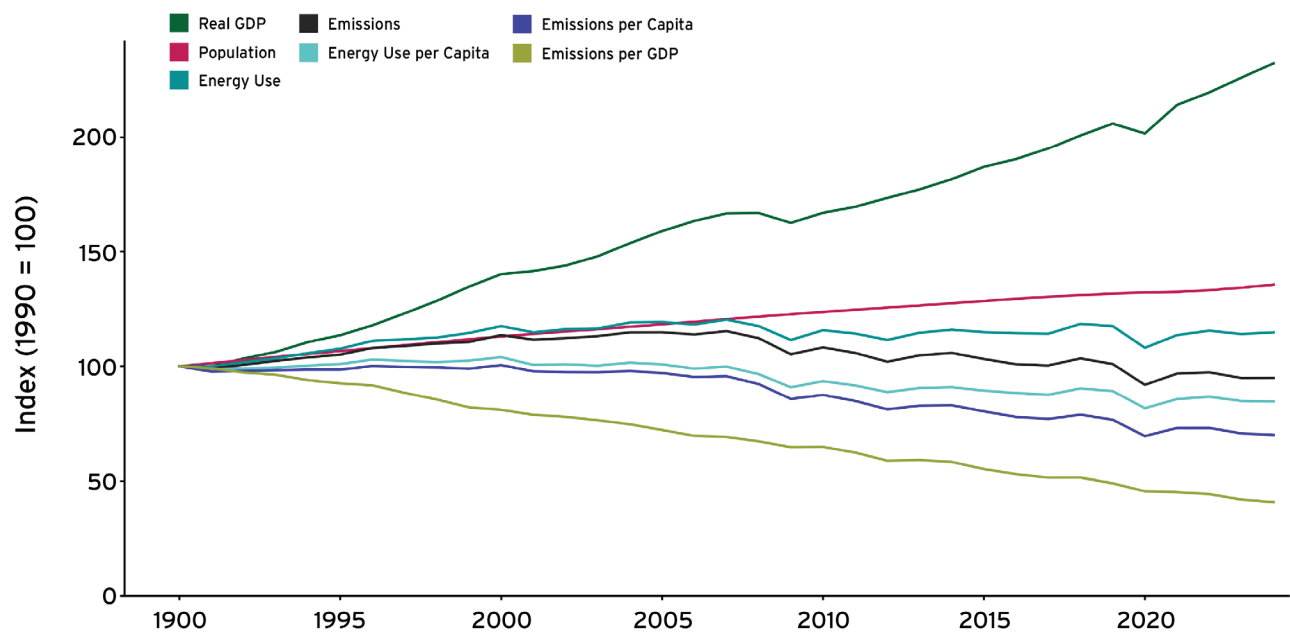
Figure 2-14: Key Economic and Demographic Indicator Trends
