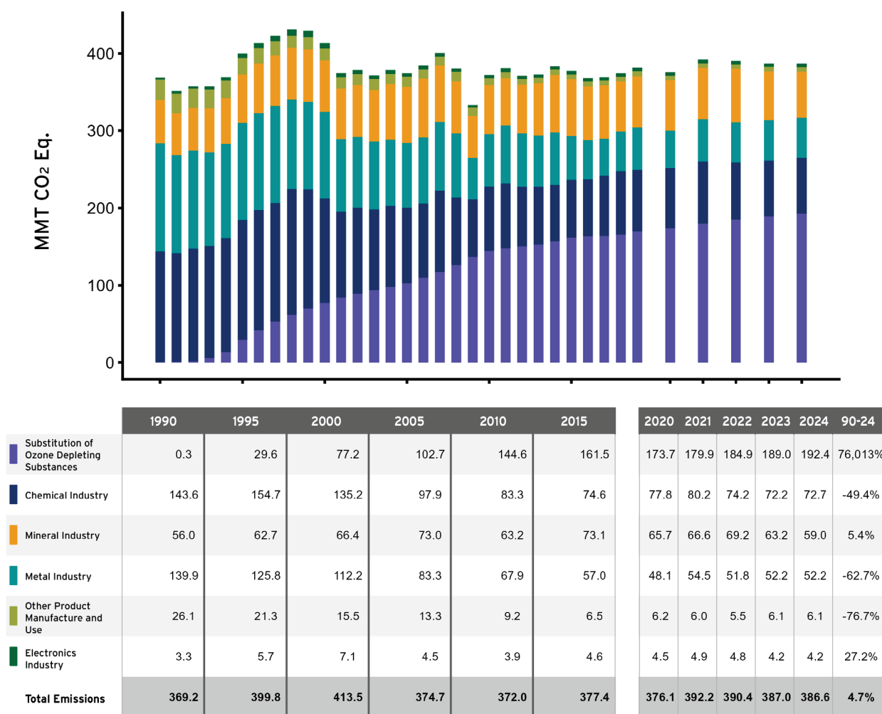
Figure 2-6: Trends in Industrial Processes and Product Use Sector Greenhouse Gas Sources (MMT CO 2 Eq.)
