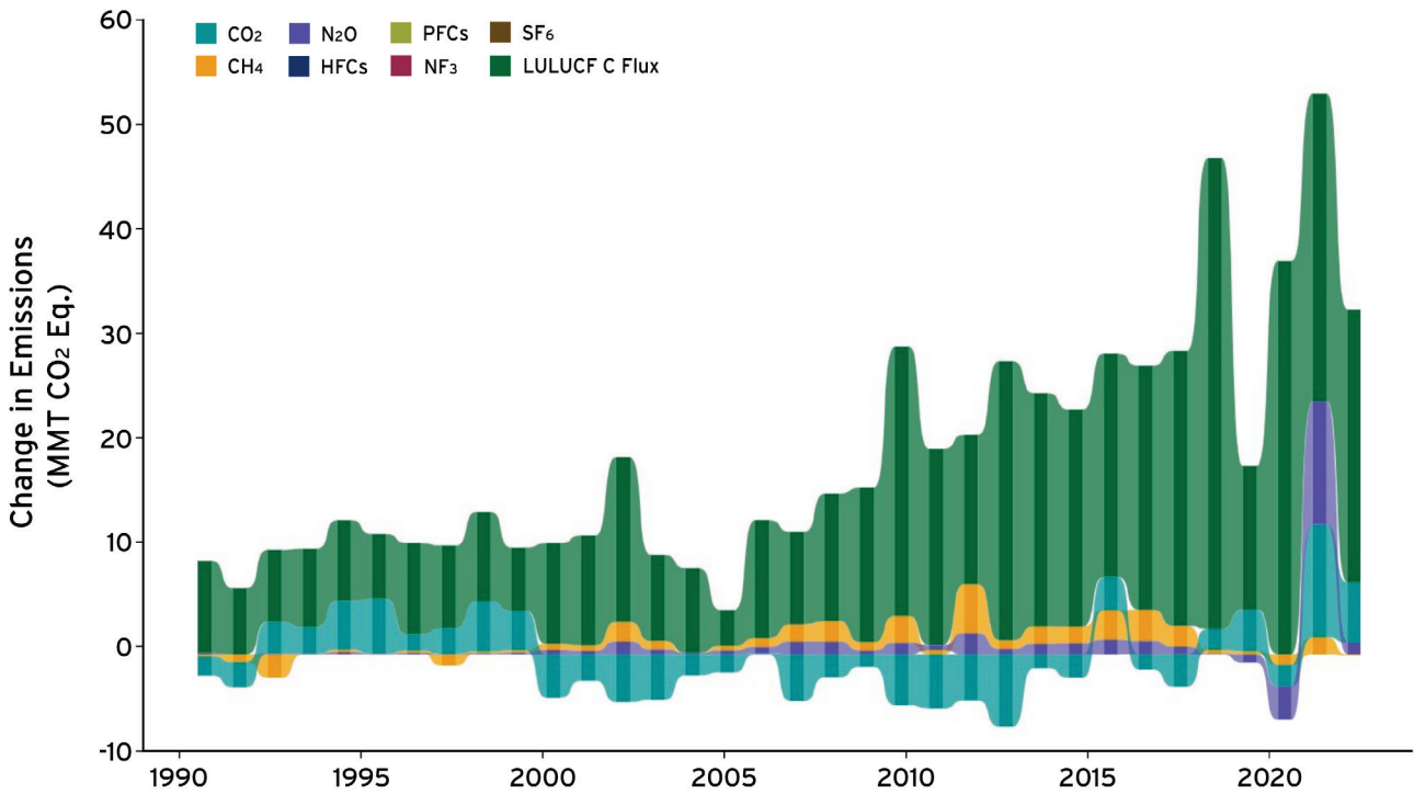
Figure 9-4: Impacts from Recalculations by Gas on Net Emissions Over Time
