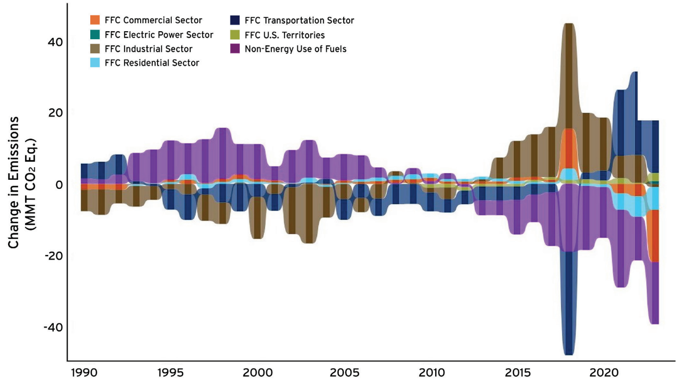
Figure 9-6: Impacts from Recalculations in Energy Subsectors
