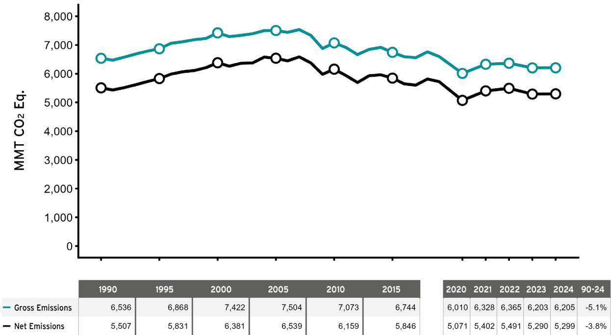
Figure 2-1: U.S. Gross and Net Emissions
