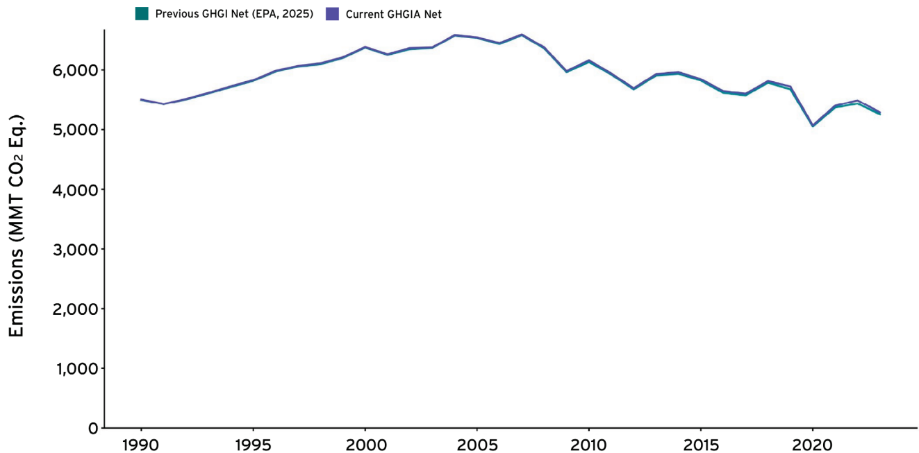
Figure 9-1: Impacts from Recalculations on Net Emissions
