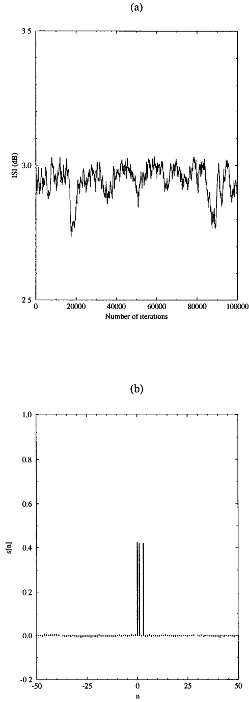
Figure 6: The ISI (a) and the impulse response (b) of the equalized system when the initial values of g_0 is unit, and the rest of g_n are zero.
