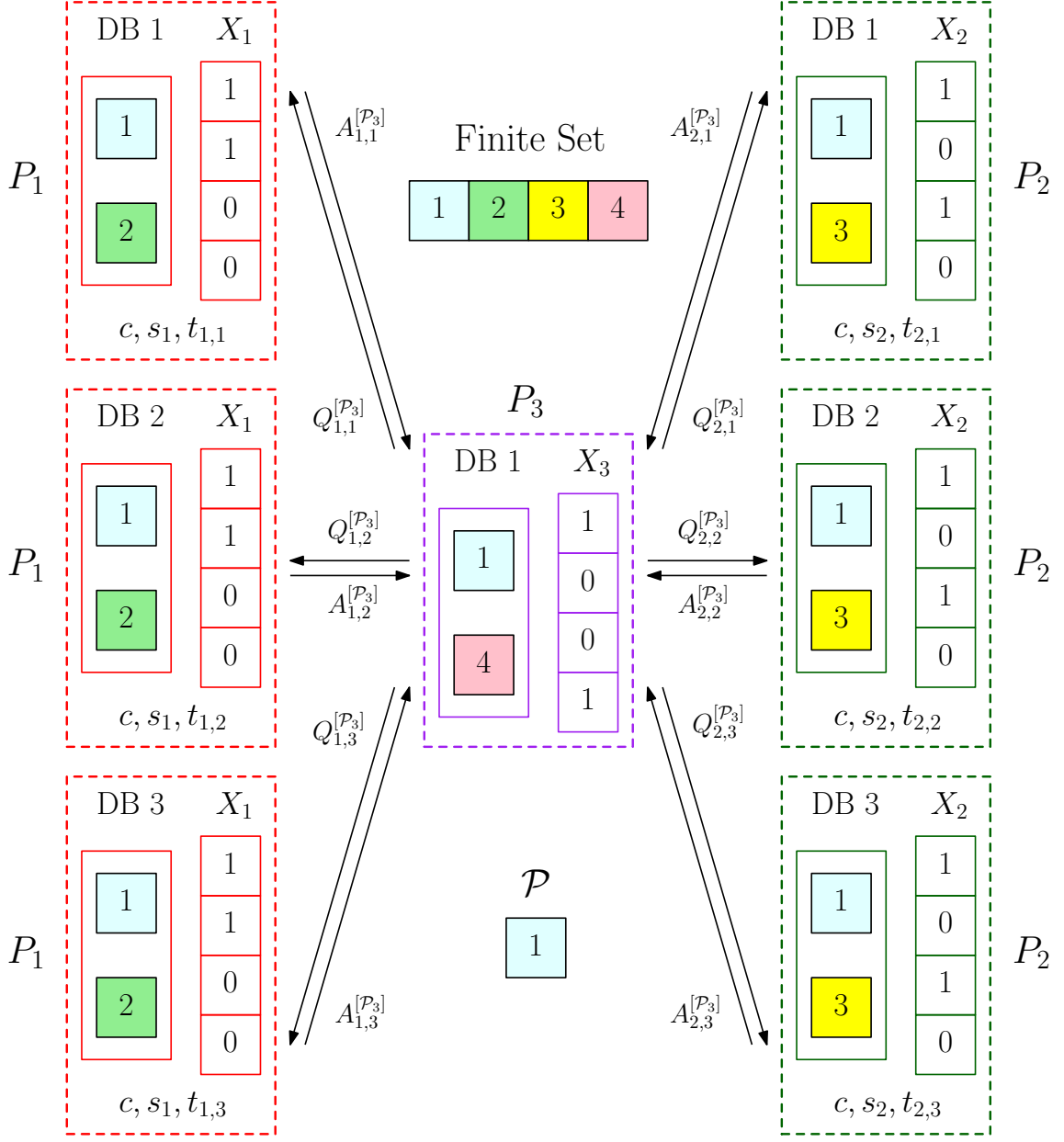
Figure 4.1: MP-PSI for the motivating example.
