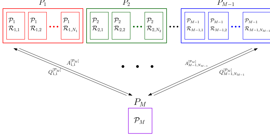
Figure 1.1: Multi-party private set intersection (MP-PSI) system model.
