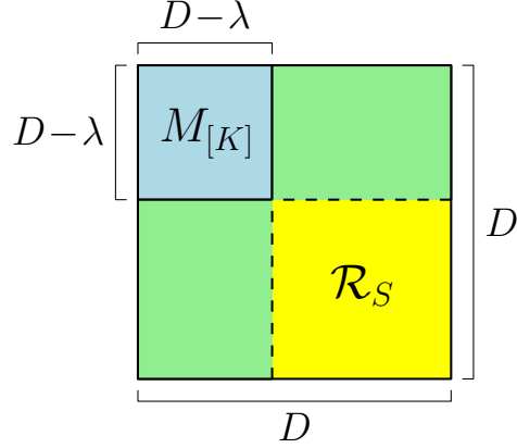
Figure 8.2: Structure of the D \times D message matrix \Omega .
