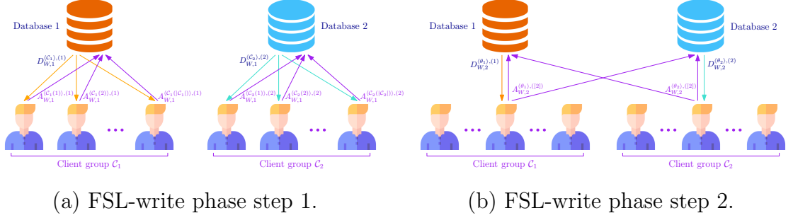
Figure 7.3: Data flow in the FSL-write phase of our FSL system model.
