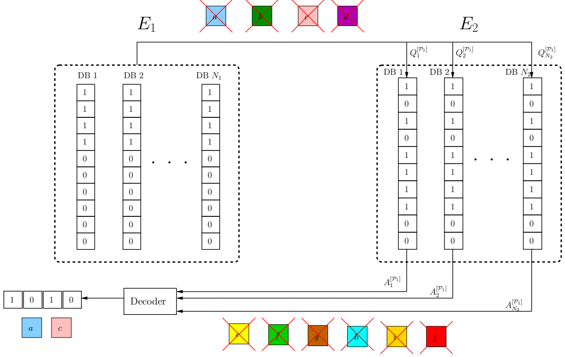
Figure 2.3: Example for the transformation from the PSI problem to an MM-SPIR problem. E_1 needs to retrieve the elements corresponding to \mathcal{P}_1 from the incidence vector X_2 without revealing \mathcal{P}_1 , while E_2 responds with answer strings that do not leak \bar{\mathcal{P}}_1 .
