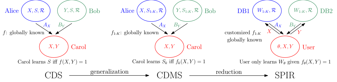
Figure 5.1: Relationship among CDS, CDMS and SPIR.
