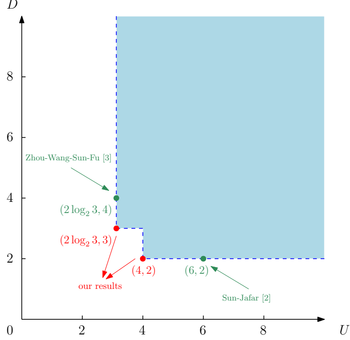
Figure 5.6: Achievable (U, D) region for two-database SPIR with K = 3 , L = 1 .
