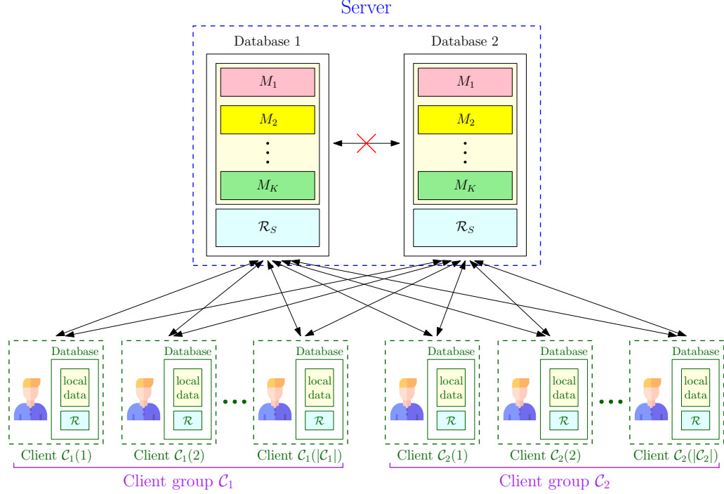
Figure 7.1: Distributed federated submodel learning (FSL) system model.
