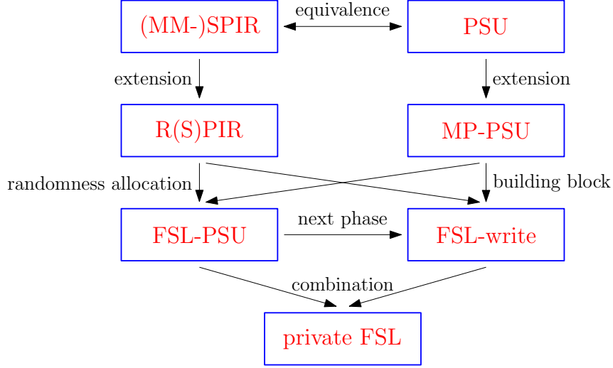
Figure 1.2: Techniques used, their relationships, and the roadmap of the development of the private FSL in Chapter 7.
