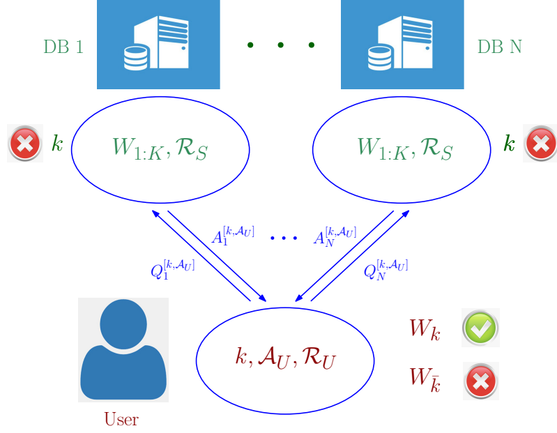
Figure 3.1: System model for SPIR with user-side common randomness.
