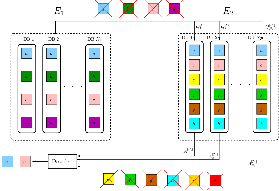
Figure 2.1: Example for the private set intersection (PSI) problem. E_1 has the set \mathcal{P}_1 = \{a, b, c, d\} and E_2 has the set \mathcal{P}_2 = \{a, c, e, f, g, h\} . E_1 submits queries to E_2 that do not leak information about \mathcal{P}_1 , while E_2 responds with answers that do not leak information about e, f, g, h (or non-existence of i, j ). By decoding the answers, E_1 learns that \mathcal{P}_1 \cap \mathcal{P}_2 = \{a, c\} .
