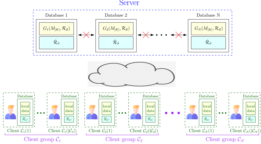
Figure 8.1: Federated submodel learning (FSL) problem in distributed storage system.
