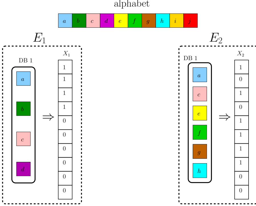
Figure 2.2: Example for the transformation from sets to incidence vectors. E_1 has the set \mathcal{P}_1 = \{a, b, c, d\} and E_2 has the set \mathcal{P}_2 = \{a, c, e, f, g, h\} . The alphabet is \mathcal{P}_{alph} = \{a, b, c, d, e, f, g, h, i, j\} . Entity E_i constructs an incidence vector X_i to facilitate MM-SPR.
