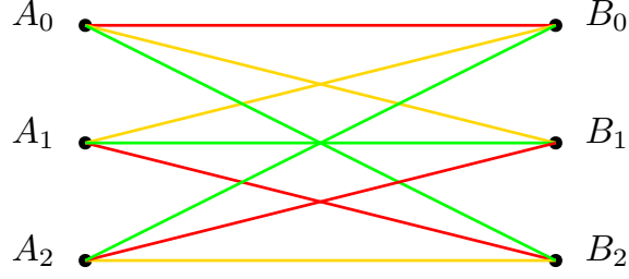
Figure 5.2: Bipartite graph for K = 3 messages and U = 2 \log_2 3 upload cost.
