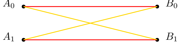
Figure 5.4: Bipartite graph for K = 2 messages and U = 2 upload cost.
