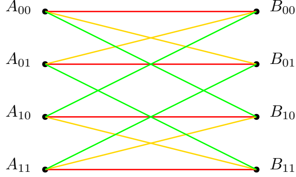
Figure 5.3: Bipartite graph for K = 3 messages and U = 4 upload cost.
