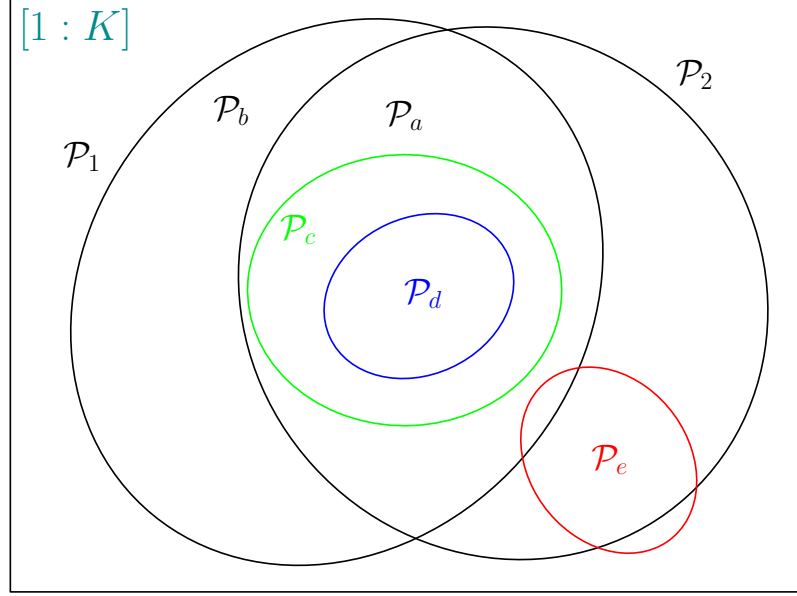
Figure 2.4: The relation of the index sets presented in Lemma 2.3 and used in Lemmas 2.4 and 2.5.
