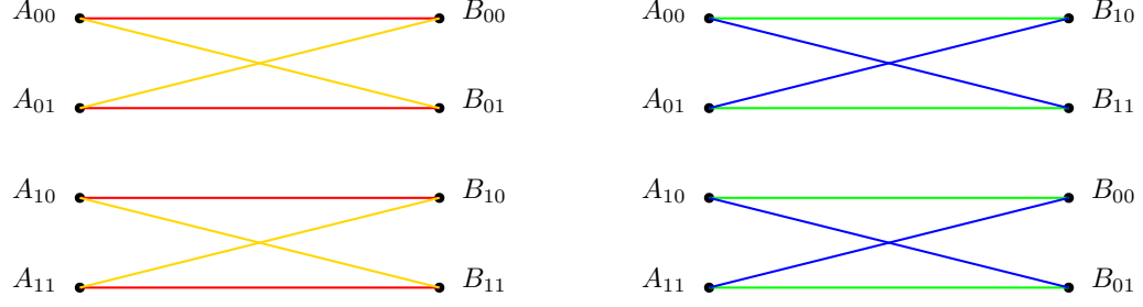
Figure 5.5: Bipartite graph for K = 4 messages and U = 4 upload cost.
