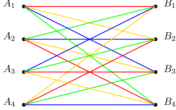
Figure 6.1: A two-database RSPIR bipartite graph for K = 4 messages.
