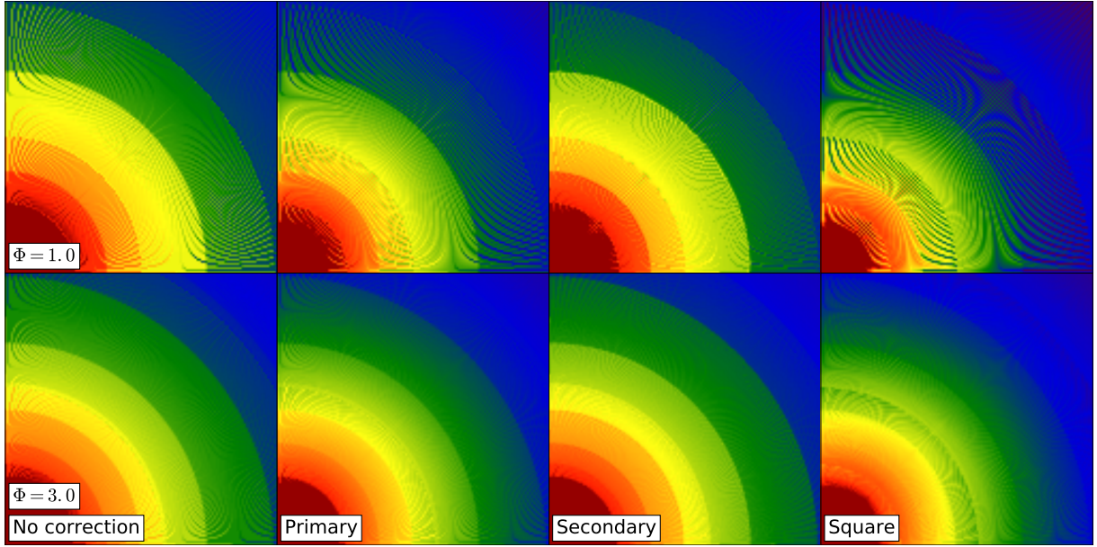
Figure 3.10: This figure shows a selection of correction methods for two different ray splitting rates. The parameter \Phi represents the number of rays per cell area, so that the bottom row have three times the splitting rate of those in the top row. The first column represents the method without correction factors. The second column illustrates the case with a primary correction, or the application of Equation 3.2 to the rate of ionization in every cell. The third column represents the case with primary and secondary correction, or the application of Equation 3.3 to the cell which is closest to the cell face has the greatest overlap. The fourth column represents the case with only the primary correction with f_c squared, as presented in Wise & Abel (2011). The low \Phi = 1 plots were included to emphasize the difference between these configurations; clearly a higher value of \Phi improves the accuracy for any configuration, but also increases the computational work for the simulation.
