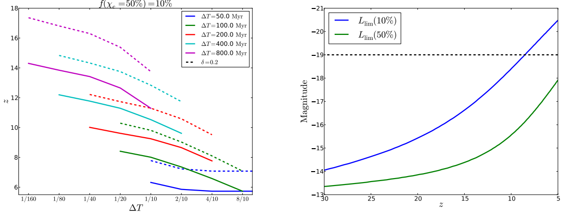
Figure 2.10: ( Left. ) Redshift at which the volume filling fraction of gas with x_e \leq 50\% reaches Q = 10\% for the same models as in Fig. 2.5. We interpret this as the redshift at which overlap of H II regions begins to be relevant and star formation transitions to a more continuous mode. We see that for all but the most bursty scenarios, the time between the beginning of general overlap and the domination of the ionizing background is relatively short. The dashed lines represent the same results in a region with an overdensity 1 + \delta = 1.2 . ( Right. ) Limiting UV magnitude above which 10% (blue line) and 50% (green line) of the total ionizing photon budget is emitted. If we take M_{UV} = -19 (dashed line) as the luminosity above which a halo will always produce stars continuously, we see that such large halos do not dominate the total luminosity until very late.
