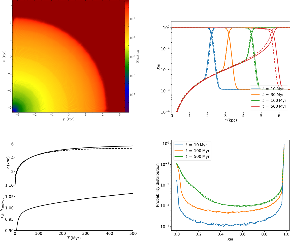
Figure 3.4: Test 1 - Expansion of an isothermal H II region in a gas of pure hydrogen. ( Top-left. ) Slice plots of the neutral fraction at 500 Myr into the simulation. The size and shape of the H II region are in good agreement with the results in RT06. ( Top-right. ) Radially averaged neutral fraction as a function of distance from the source, in kpc. The dashed lines are the same plots reproduced from RT06 using C^2 -Ray. ( Bottom-left. ) Ionization front plotted along with the analytical model (top) and the ratio of these models (bottom). We note that the simulation deviates from the analytic solution at the beginning and end of the simulation. This is a result of the soft 13.6 eV spectrum being the worst case scenario for our optically thin approximation for non-equilibrium chemistry calculation. ( Bottom-right. ) Histogram of neutral fractions at t = 10, 100, 500 Myr. The dashed lines are the same plots reproduced from RT06 using C^2 -Ray. We see that our model matches C^2 -Ray very well.
