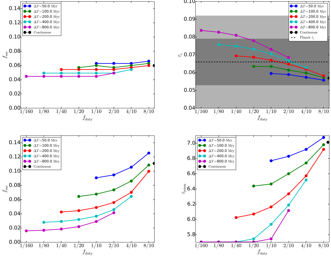
Figure 2.6: Same plots as in Fig. 2.5 but assuming a spectrum of the sources absorbed by a fixed column density of neutral hydrogen N_{\text{HI}} = 3.8 \times 10^{19} \text{ cm}^{-2} . Neutral hydrogen preferentially absorbs softer photons, thus resulting in a harder final spectrum. The overall result is a lower optical depth (for fixed z_{\text{re}} ), earlier completion of reionization (for fixed \tau_e ), and a lower escape fraction (for fixed \tau_e, z_{\text{re}} ).
