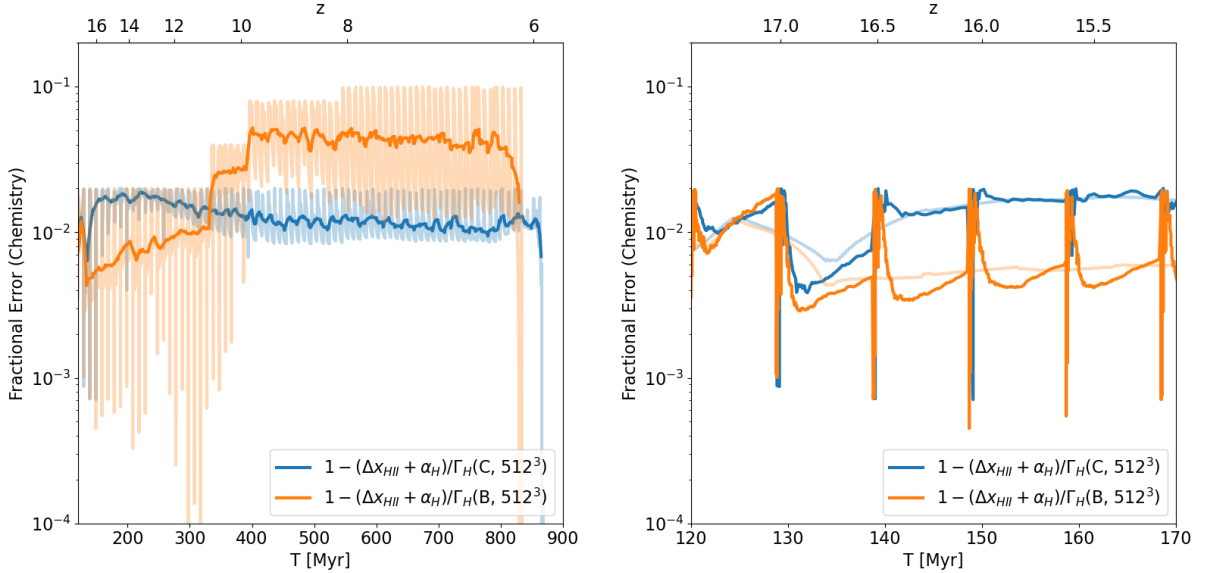
Figure 4.13: ( Left ). The error in H II associated with the time steps taken in both simulations (which are shown in Figure 4.12). At late times we relax the constraint on the bursty model. ( Right ). A smaller slice of the left plot. In both plots, we also show the moving averages over a 10 Myr interval to smooth out the noise.
