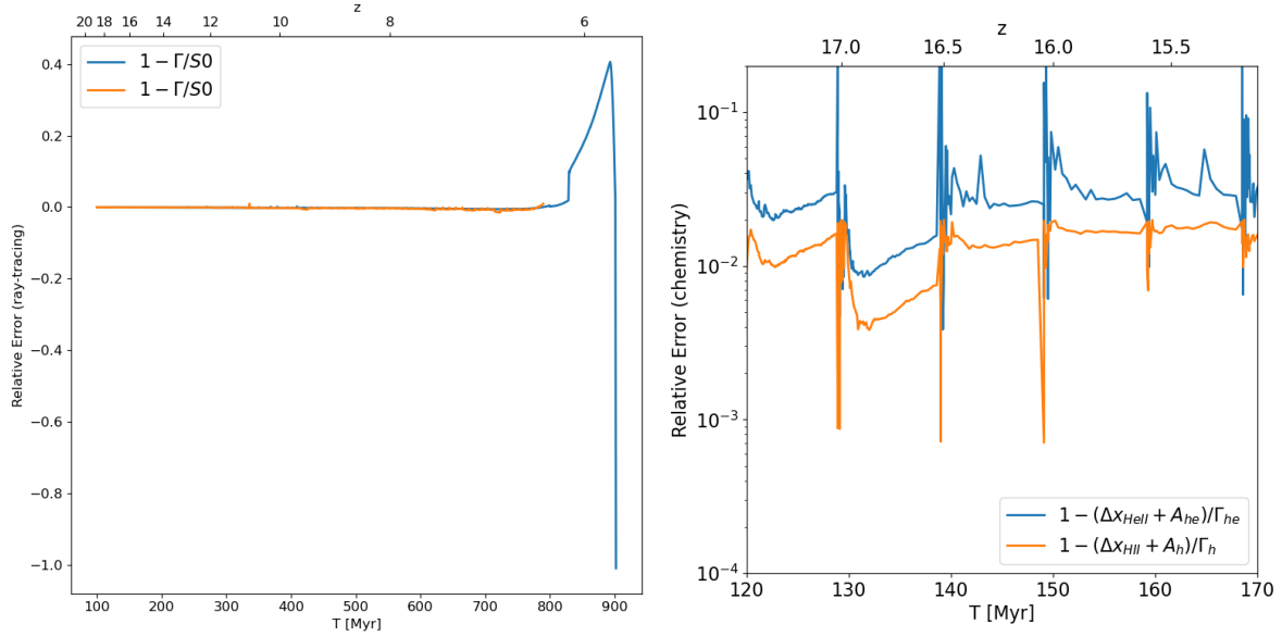
Figure 4.2: An example of the errors taken from a 50 Myr segment from on of our simulations ( Left ). The S_0 and \Gamma error plotted as the deviation of S_0/\Gamma from 1. A positive error indicates that photons are not being absorbed. ( Right ). The \Gamma_i - A_i and \Delta x_i/\Delta t error shown for hydrogen and helium separately.
