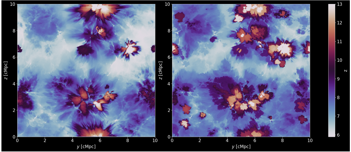
Figure 4.14: A visualization of the redshift of reionization (specifically x_{\text{H II}} > 0.9 ) for a slice through the continuous ( left ) and bursty ( right ) models, respectively. In the continuous model, gas generally reionizes radially outwards from the brightest sources, while in the bursty model there smaller and more spread out regions of ionization.
