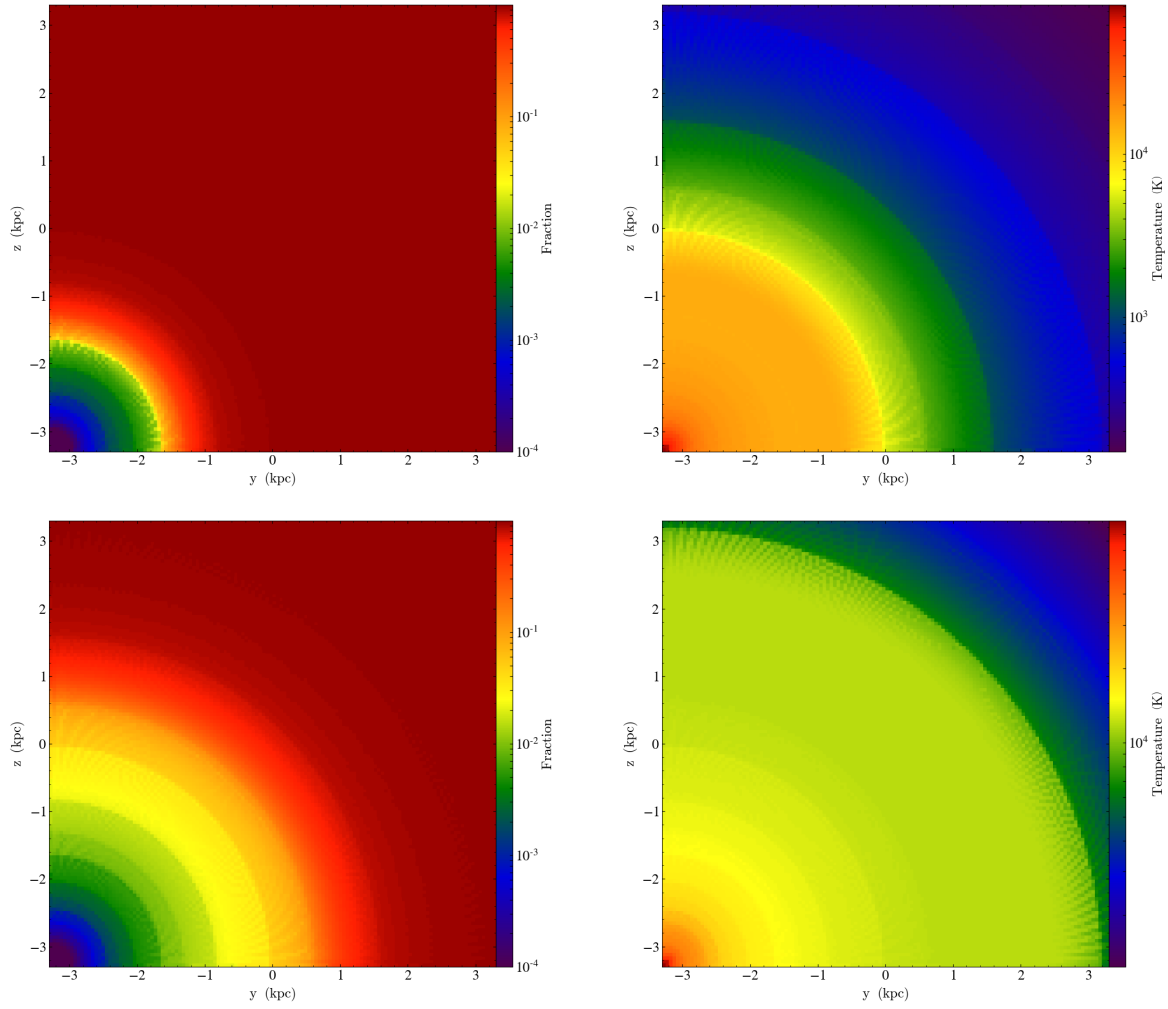
Figure 3.5: Test 2 - Expansion of H II region in a gas of pure hydrogen with evolving temperature. ( Top and bottom left. ) Slice plots of the neutral fraction at 10 Myr and 500 Myr into the simulation, respectively. ( Top and bottom right. ) Slice plots of the temperature at 10 Myr and 500 Myr into the simulation. The adopted 10^5 K blackbody spectrum introduces harder photons which heat the gas to a much larger radius than the size of the Strömgren sphere, in agreement with the results presented in RT06.
