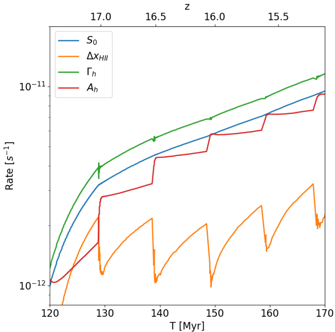
Figure 4.1: Example rates of photon production, hydrogen ionization, hydrogen recombination, and ionization change taken from a 50 Myr segment of one of our simulations.
