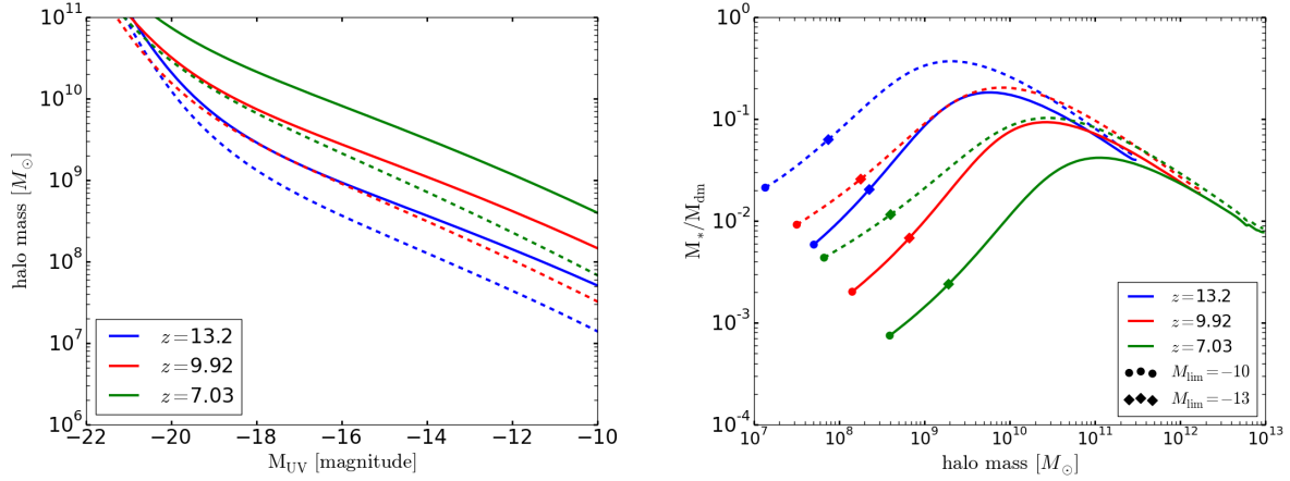
Figure 2.2: ( Left ). Typical halo mass hosting a galaxy of UV magnitude M_{UV} produced by the halo matching method in equation (2.4). The solid lines represent the continuous star formation, and the dashed lines represents bursty star formation with f_{\text{duty}} = 5\% . ( Right ). Star formation efficiency f_* \equiv M_*/M_{\text{dm}} as a function of halo mass derived by our halo matching procedure. Halo matching in the bursty star formation models places brighter stellar populations in less massive halos.
