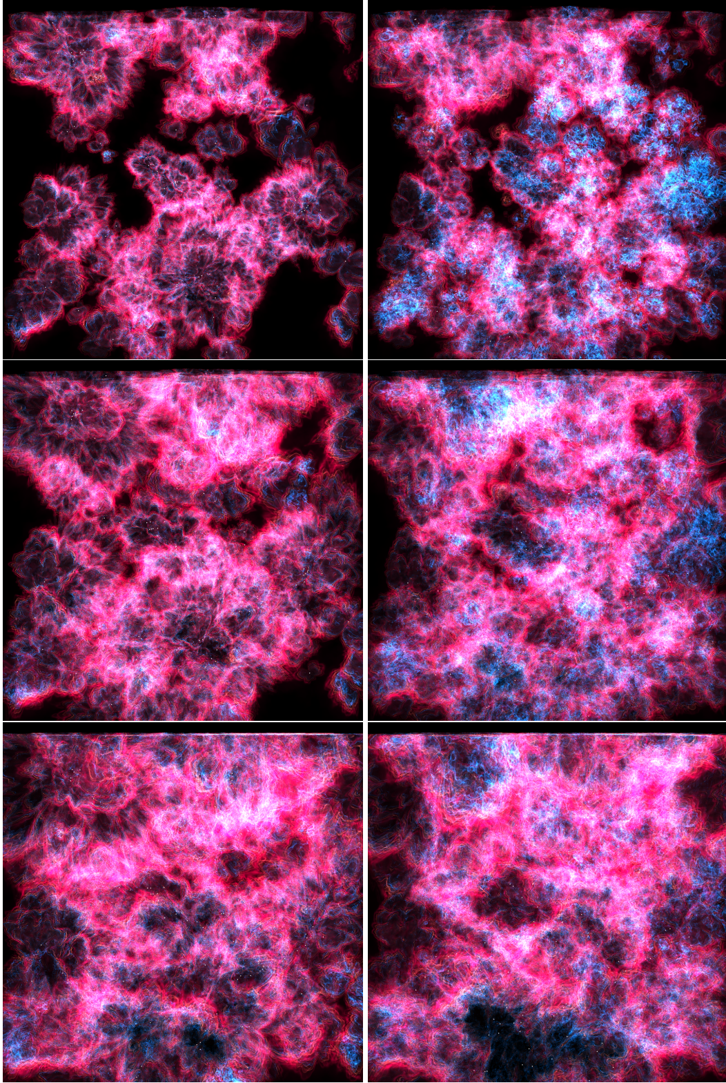
Figure 4.8: 3D visualizations from the high resolution Set 1 simulations at various times. The left and right columns correspond to the continuous and bursty models, respectively. The rows correspond to times of 450 Myr, 550 Myr, and 650 Myr into the simulations.
