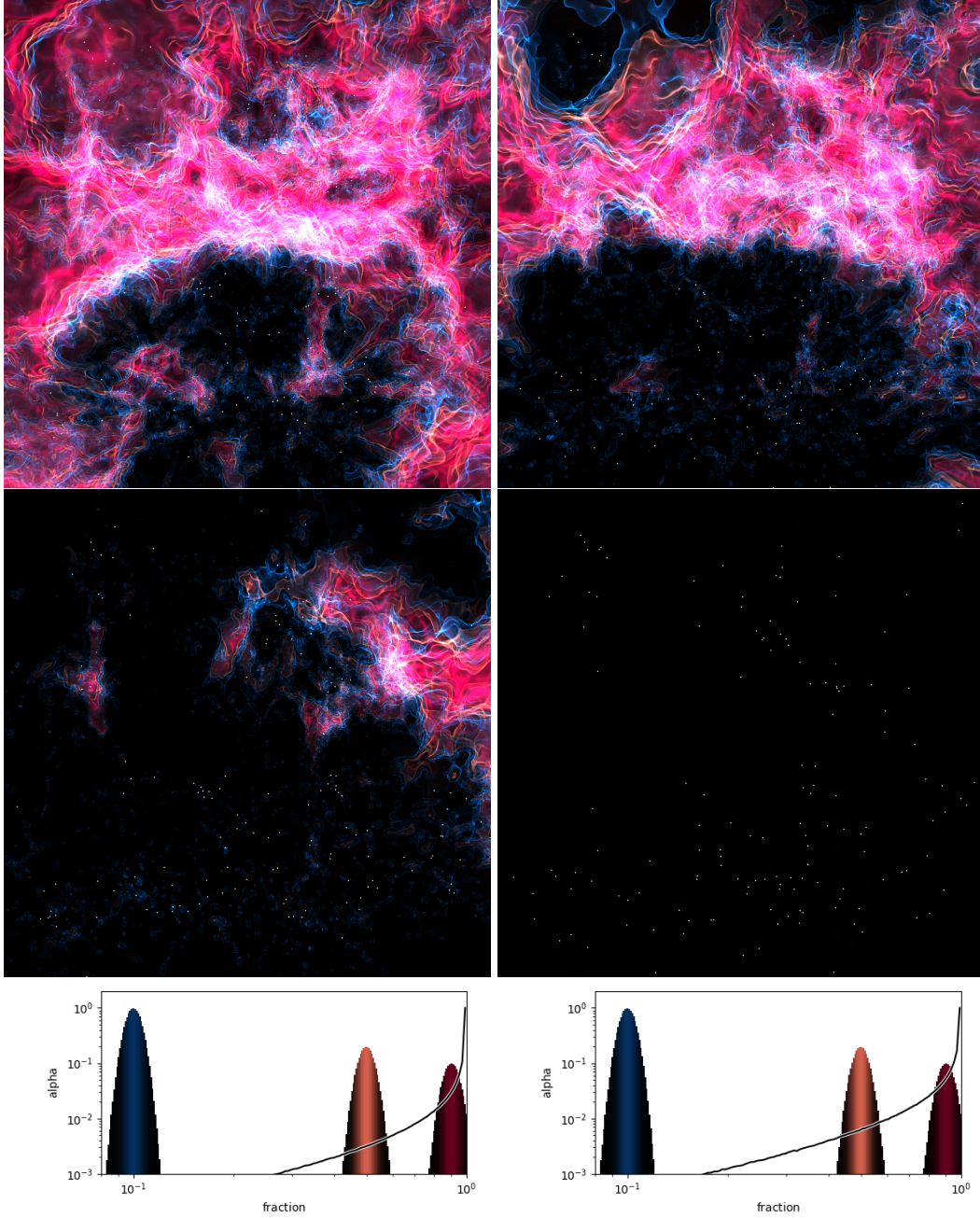
Figure 4.9: 3D visualizations from the high resolution Set 1 simulations at various times. The left and right columns correspond to the continuous and bursty models, respectively. The rows correspond to times of 750 Myr and 850 Myr into the simulations. The bottom row represents the color map transfer functions and associated histograms of neutral fraction for the 750 Myr plots.
