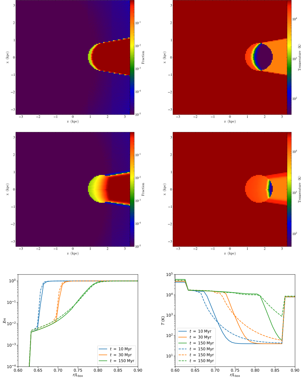
Figure 3.7: Test 3 - I-front trapping and formation of a shadow. ( Top and middle left. ) Slice plots of the neutral fraction at 1 Myr and 15 Myr into the simulation, respectively. ( Top and middle right. ) Slice plots of the temperature at 1 Myr and 15 Myr into the simulation. The shape of our shadow region expands with distance, a result of the point-like nature of the source of ionizing photons. Our results agree well with Wise & Abel (2011) , a simulation which uses the same point-like configuration. Neutral fraction ( bottom-left ) and temperature ( bottom-right ) along a ray going through the center of the dense clump. The dashed lines represent the same plots calculated using C^2 -Ray using data from RT06. We interpret the discrepancy in the right figure as the result of using a point source, as in our simulation, rather than a plan-parallel front. The diverging rays heat more effectively closer to the source (low r ) and less effectively further from the source (high r ).
