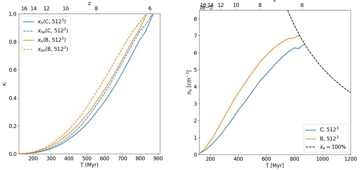
Figure 4.15: (Left) . Overall mass-weighted ionization rates of hydrogen and helium. (Right) . Physical density of free electrons.
