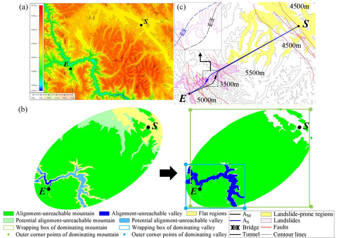
FIGURE 16 (a) Terrain map of the study area; (b) dominating landform determination; and (c) the horizontal alignments of A_M and A_S .
