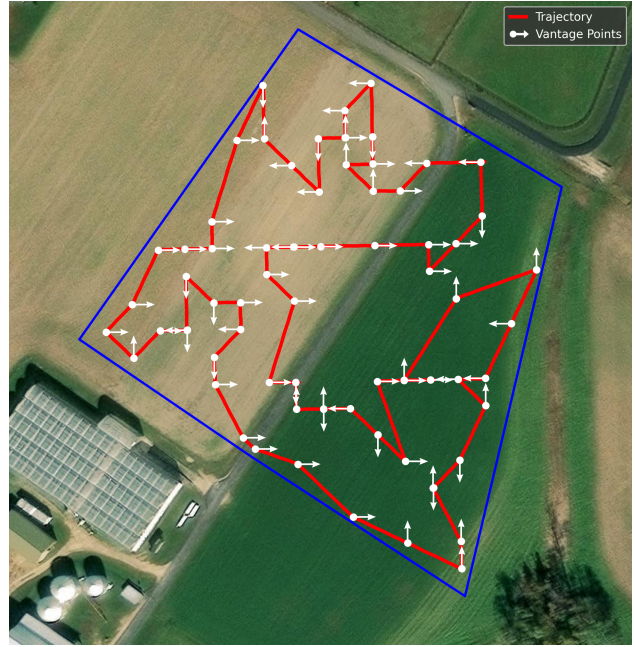
(b) Greedy
