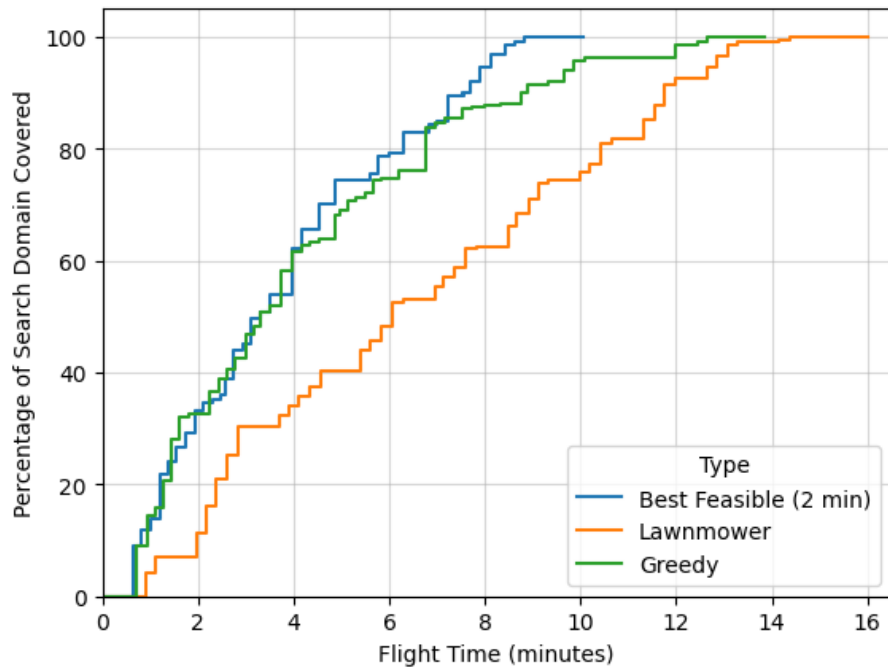
(a) 5 cm/pixel
