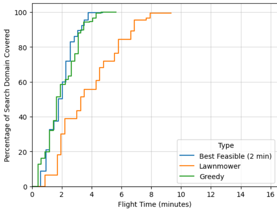
(b) 10 cm/pixel
