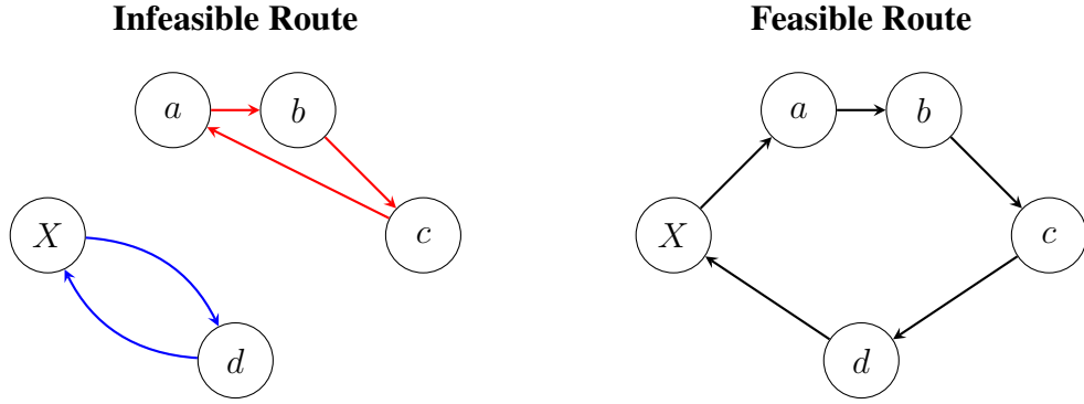
Figure 2.1: Left: An infeasible solution to the TSP with two subtours, violating MTZ constraints. Right: A feasible solution to the TSP with a single tour.
