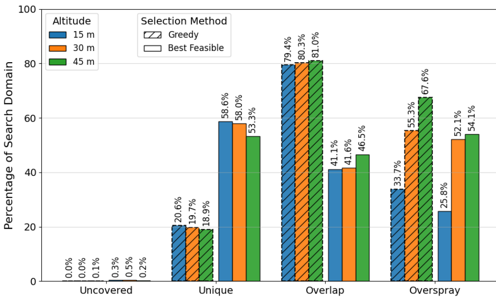
(b) Characterization of vantage point coverage relative to number of cells in search domain.
