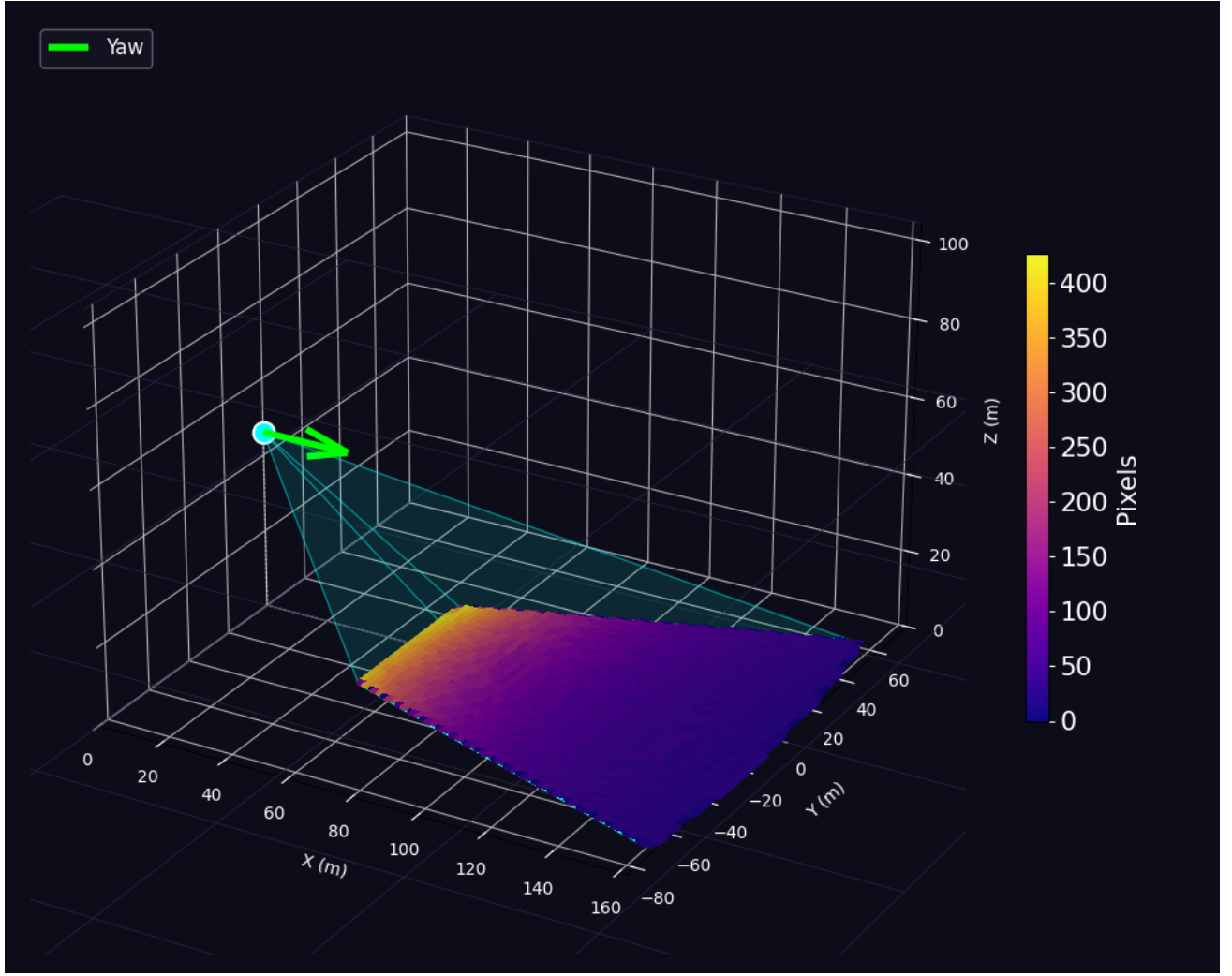
Figure 3.2: Example vantage point and pixel density map using Grazer-A hi-res Camera at an altitude of 46 meters and a pitch of 60^\circ from nadir to the direction of travel.
