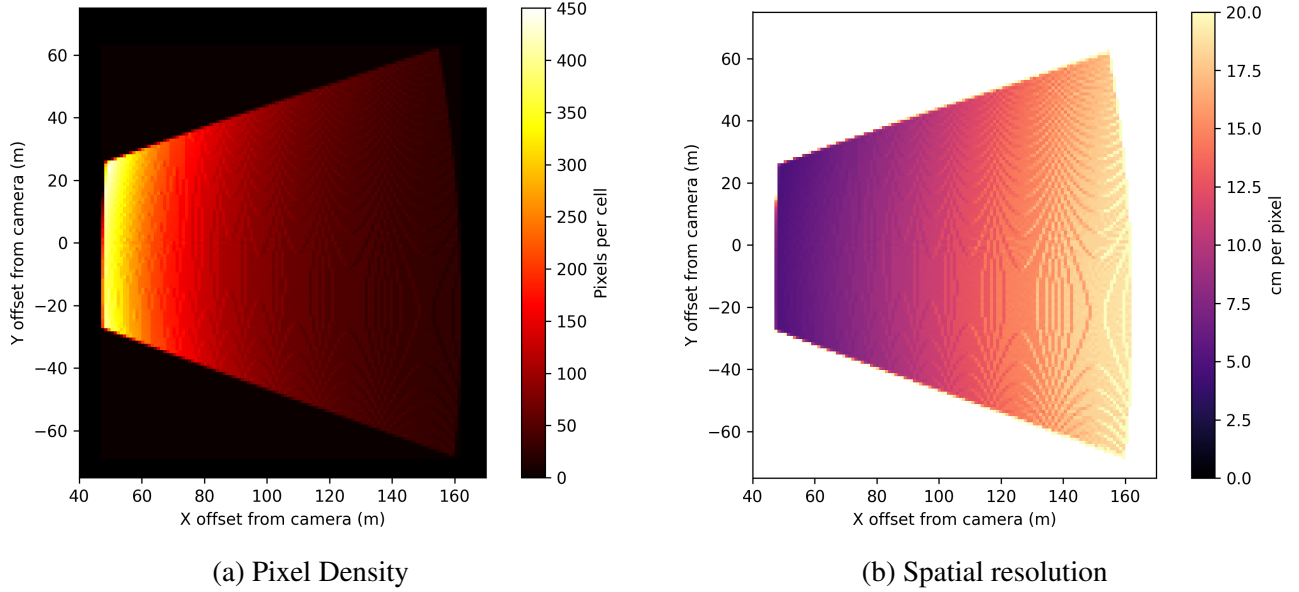
Figure 3.1: Sensor footprint of Grazer-A hi-res camera at an altitude of 46 meters and a pitch of 60^\circ from nadir to the direction of travel.
