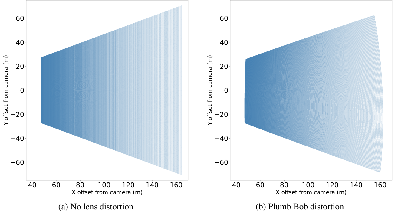
Figure 5.5: Projection of all pixels from the Grazer-A hi-res camera to the ground plane at an angle of 60^\circ from nadir to the direction of travel at an altitude of 46 meters.
