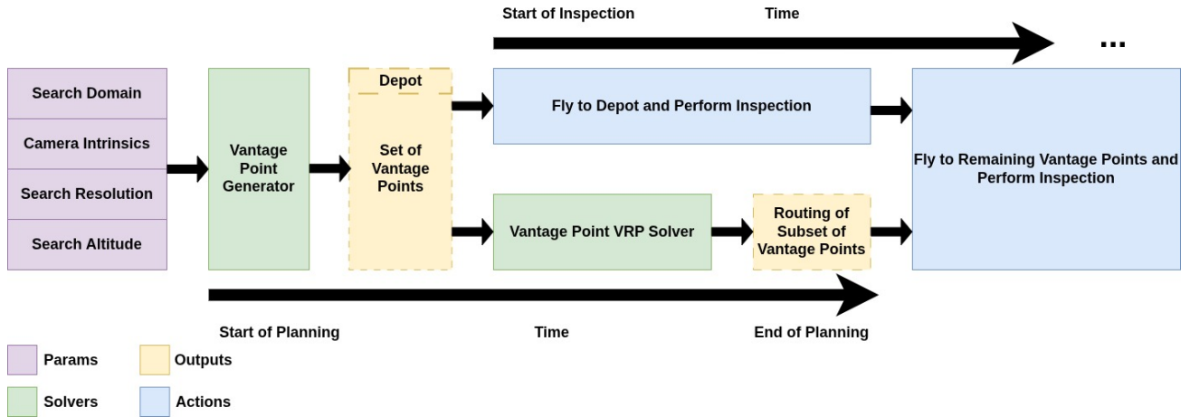
Figure 4.1: Framework for solving VRPs for real-time routing of vantage point-based coverage path plans.
