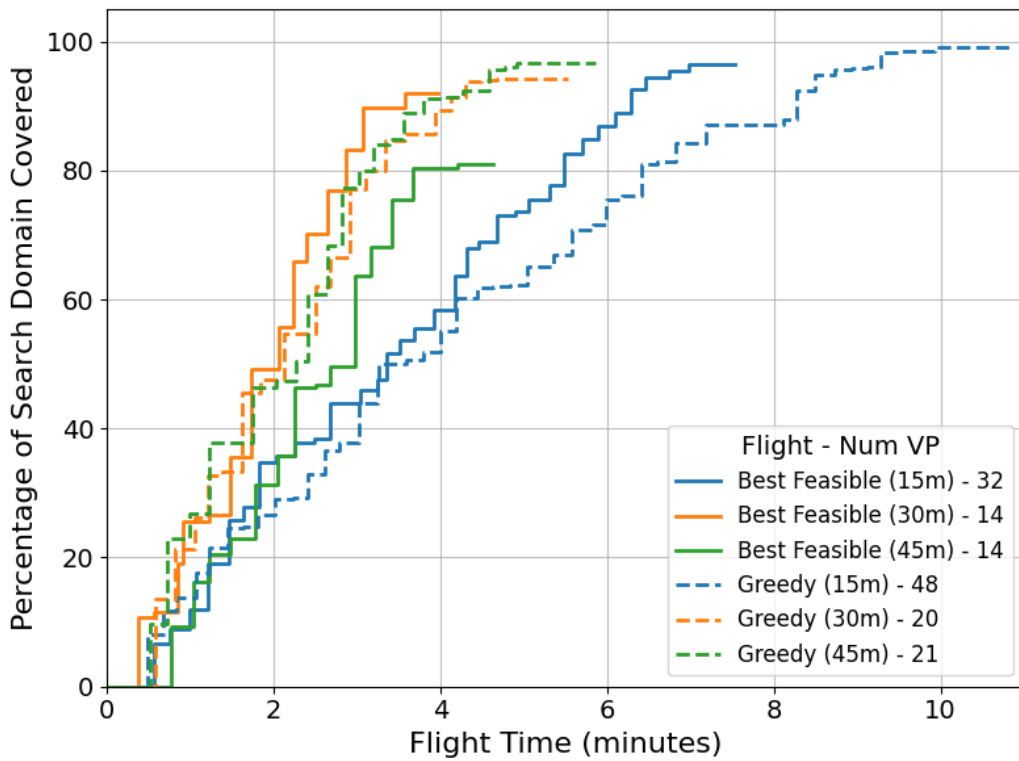
(a) Coverage over time. Num VP is the number of vantage points in each path plan.
