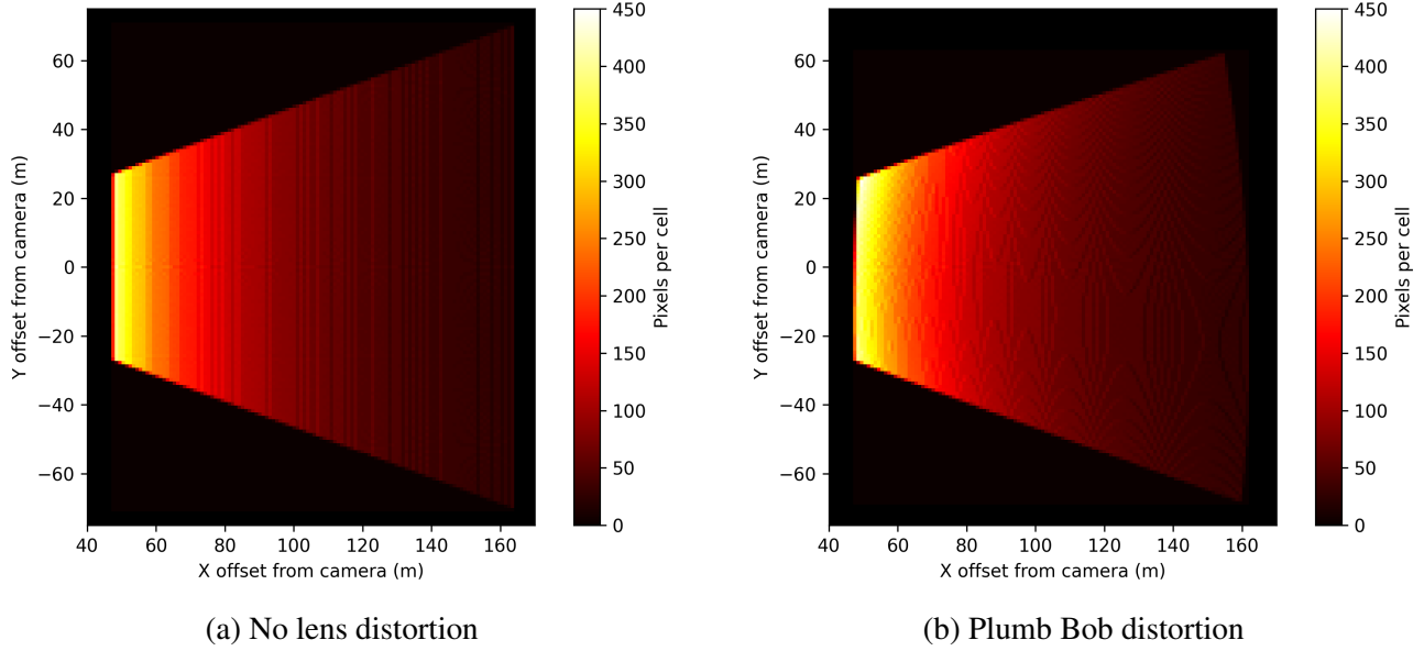
Figure 5.7: Pixel density within sensor footprint of the Grazer-A hi-res camera.
