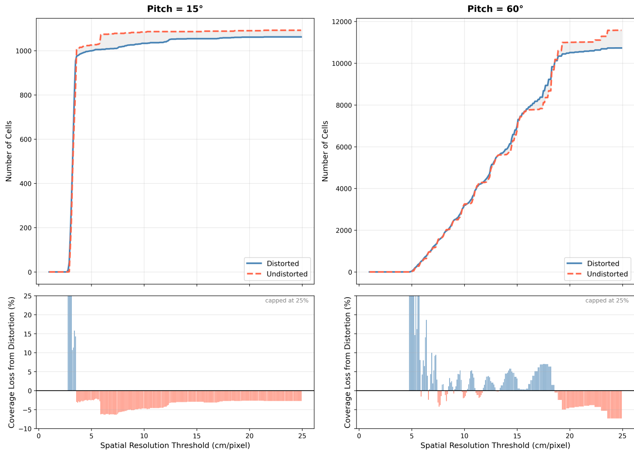
Figure 5.10: Difference in area of effective sensor footprint with and without lens distortion.
