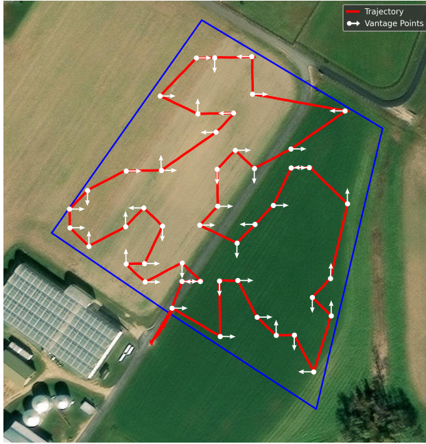
(a) Greedy
