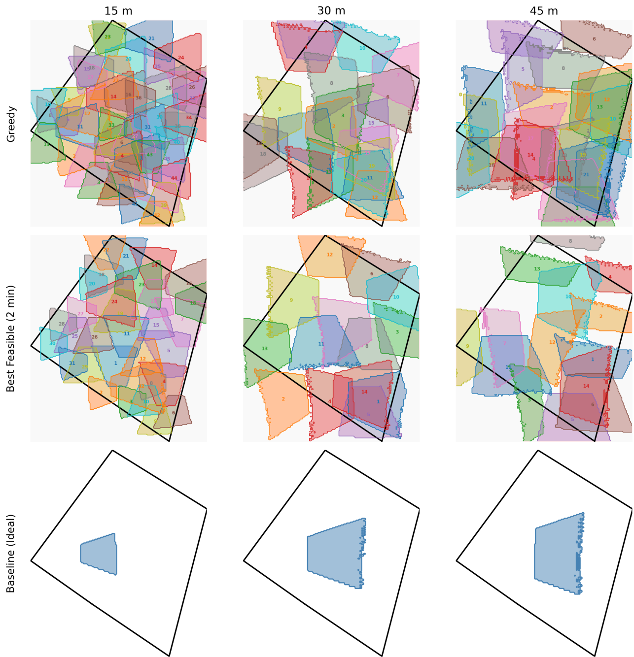
Figure 5.21: Effective sensor footprints at actual obtained vantage points from real-world testing at a spatial resolution of 10 cm/px.
