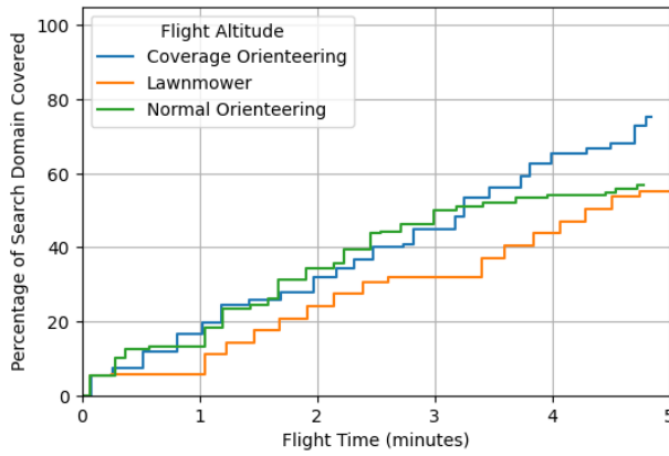
(a) 5 minutes
