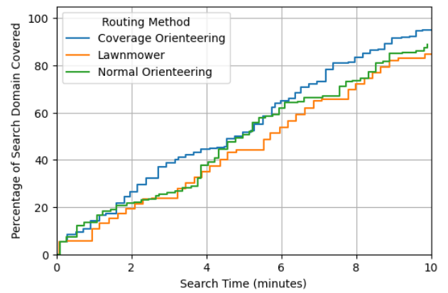
(b) 10 minutes
