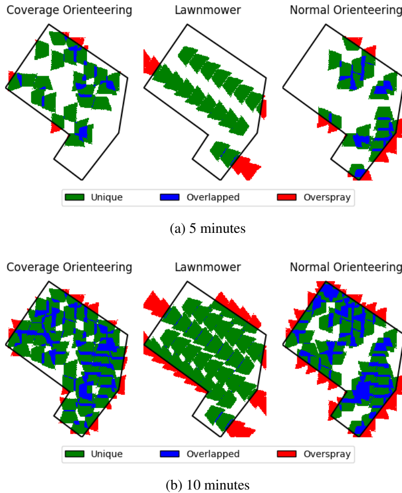
Figure 5.18: Characterization of coverage for different routing methods and time limits at a spatial resolution of 5 cm/px.
