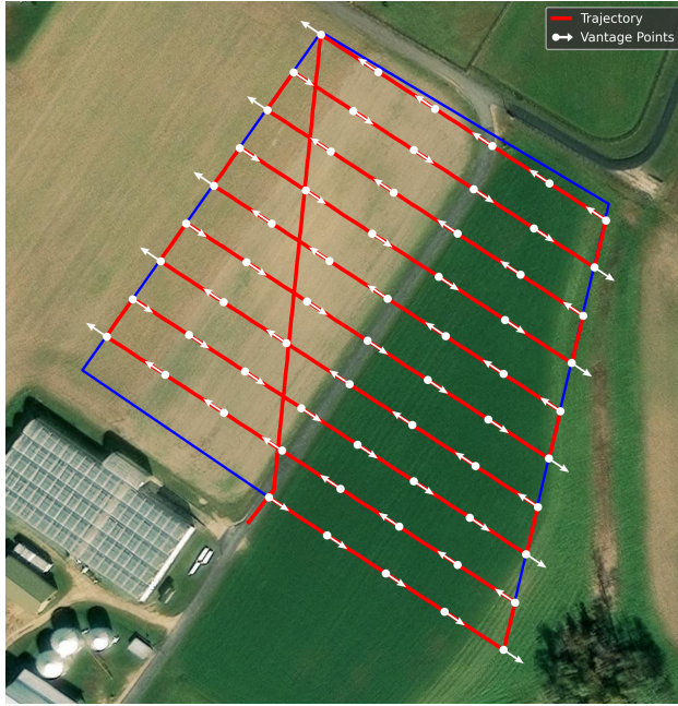
(a) Lawnmower-derived
