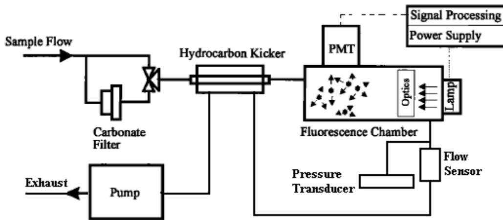
Figure 2.4. Schematic diagram of the modified SO 2 analyzer (adapted from [Luke, 1997]).
