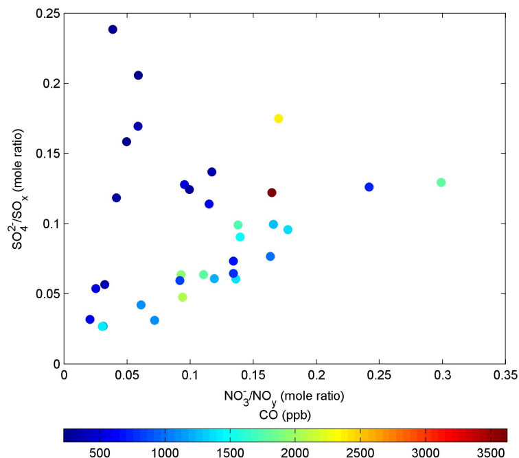
Figure 5.2. \text{SO}_4^{2-}/\text{SO}_x and \text{NO}_3^-/\text{NO}_y mole ratios as a function of CO concentration. Under relatively clean conditions, \text{SO}_4^{2-}/\text{SO}_x ratio is generally higher than \text{NO}_3^-/\text{NO}_y ratio, and vice versa under polluted conditions.
