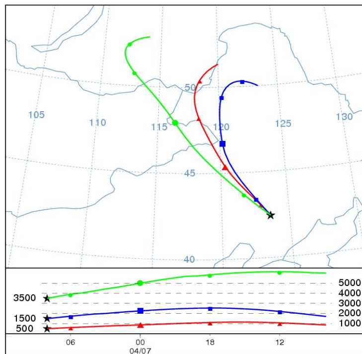
Figure 4.16. Backward trajectories calculated with the HYSPLIT model for air arriving at location of northern spiral (42.5°N, 123.5°E) on April 7 (Figure 4.18). The lower panel depicting vertical motions of the trajectories shows subsidence in this postfrontal air.
