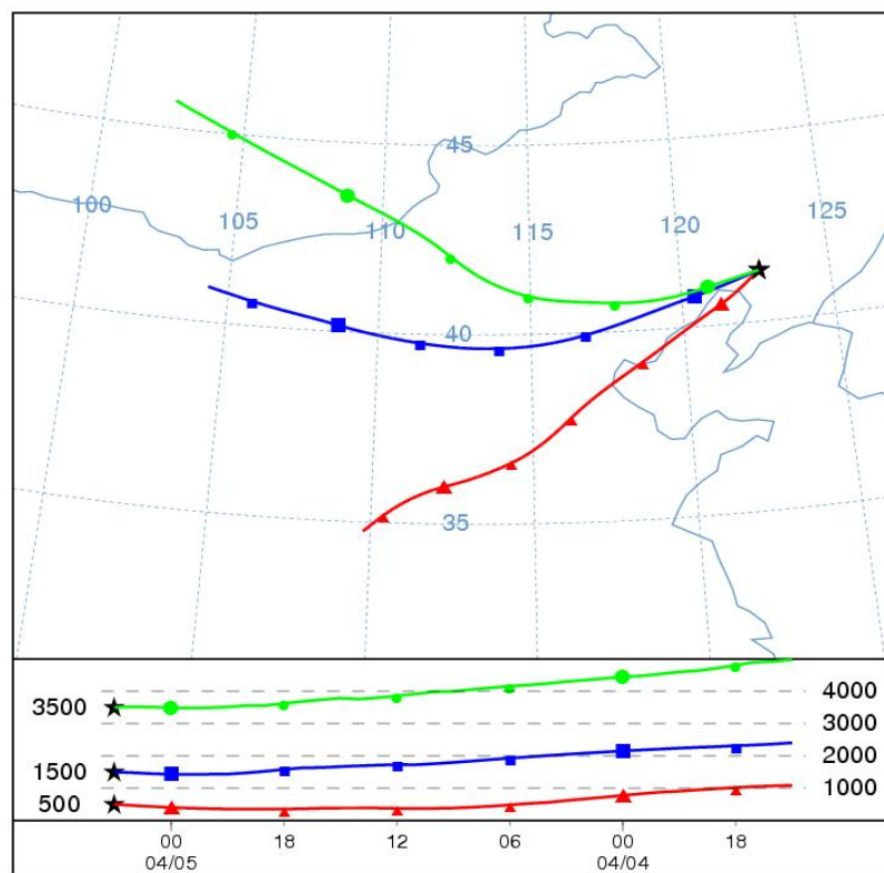
Figure 4.12. Backward trajectories calculated with the HYSPLIT model for air arriving at location of the southern spiral (41.4°N, 122.7°E, Figure 4.7) in the PBL (500 m above ground level) and in the FT (1500 and 3500 m) on April 5. The lower panel depicts vertical motions and shows little evidence of WCB lofting in the prefrontal zone for this episode. Back trajectories for the second spiral point, 200 km to the north and 2 hr later are similar.
