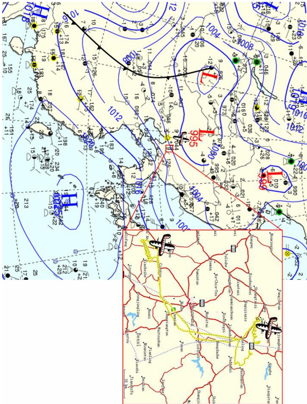
Figure 4.7. Surface analysis (Korean Meteorological Administration) for 00 UTC April 5, 2005 showing a low-pressure system (cyclone) moving towards Shenyang. The approximate location of the flights is shown by the symbol of an aircraft and the actual flight pattern is shown in the insert. Profiling spirals were conducted north and south of Shenyang (locations marked with aircraft symbols). Note little cloud cover or precipitation was reported in the vicinity of the flight and several hundred km to the south ahead of the surface cold front. Yellow circles indicate occurrence of fog.
