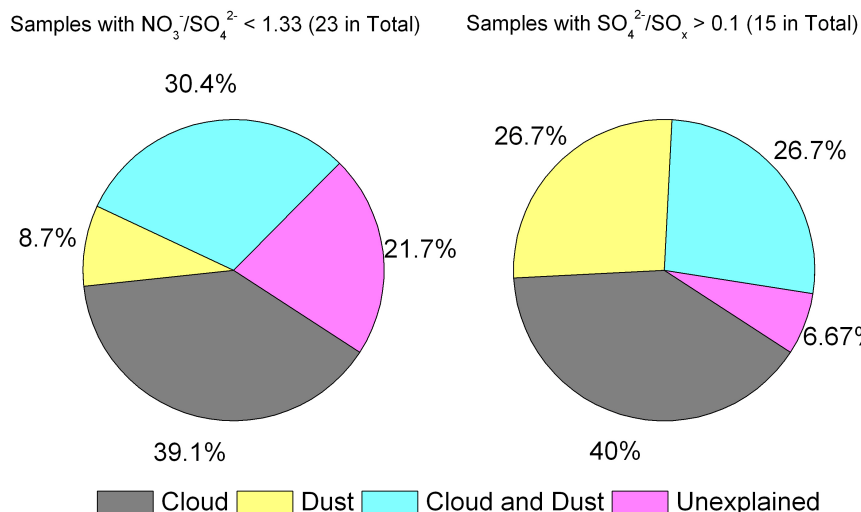
Figure 5.5. Percentage of “cloud”, “dust”, “cloud and dust”, and “unexplained” events for samples with \text{NO}_3^-/\text{SO}_4^{2-} mole ratio below 1.33 (left), and samples with \text{SO}_4^{2-}/\text{SO}_x mole ratio over 0.1 (right).
