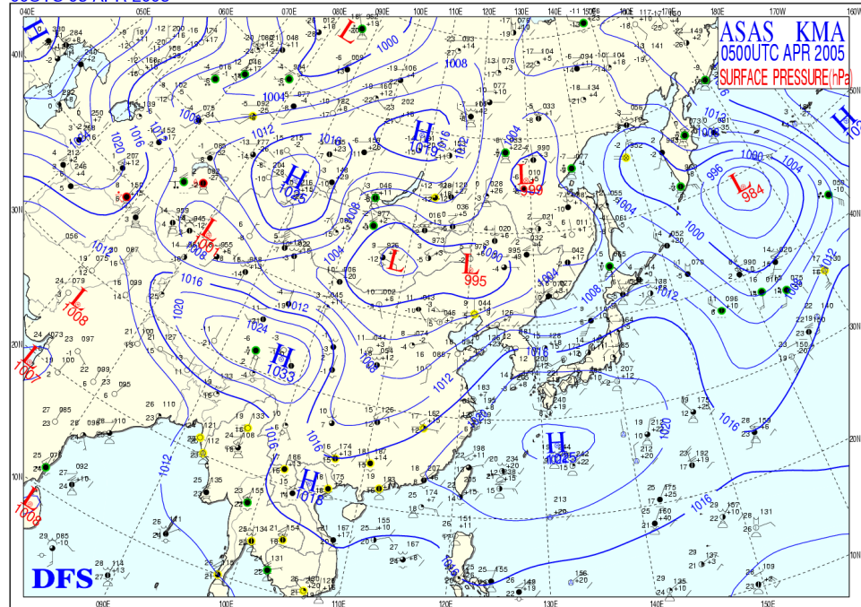
Appendix I.5. Surface weather analysis of East Asia at 00 UTC on April 5, 2005.
