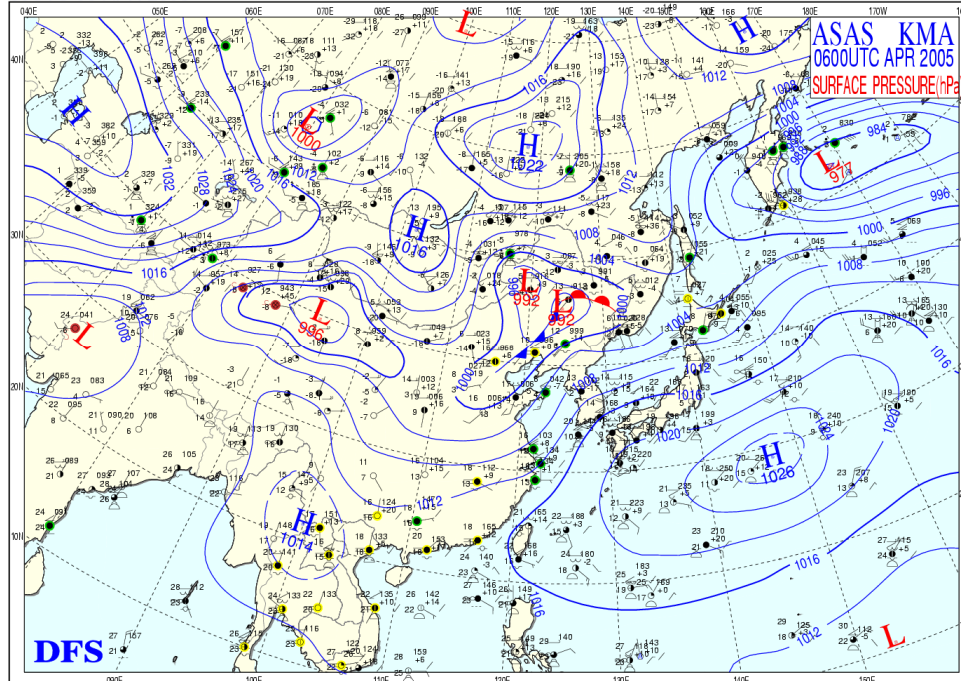
Appendix I.6. Surface weather analysis of East Asia at 00 UTC on April 6, 2005.
