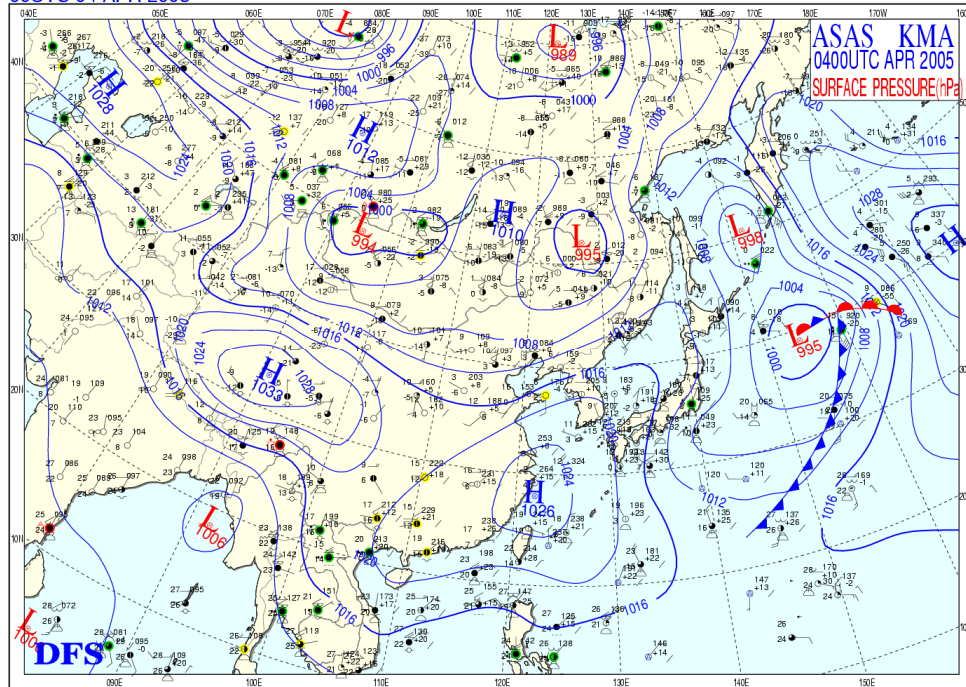
Appendix I.4. Surface weather analysis of East Asia at 00 UTC on April 4, 2005.
