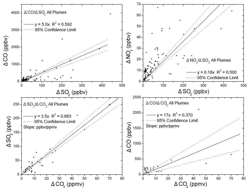
Figure 3.15. Correlations of \Delta\text{CO} , \Delta\text{SO}_2 , \Delta\text{NO}_y , and \Delta\text{CO}_2 for all plume data. Dotted lines mark the 95% confidence interval for the correlation analysis. Note the slopes for \Delta\text{SO}_2/\Delta\text{CO}_2 and \Delta\text{CO}/\Delta\text{CO}_2 are in ppbv/ppmv.
