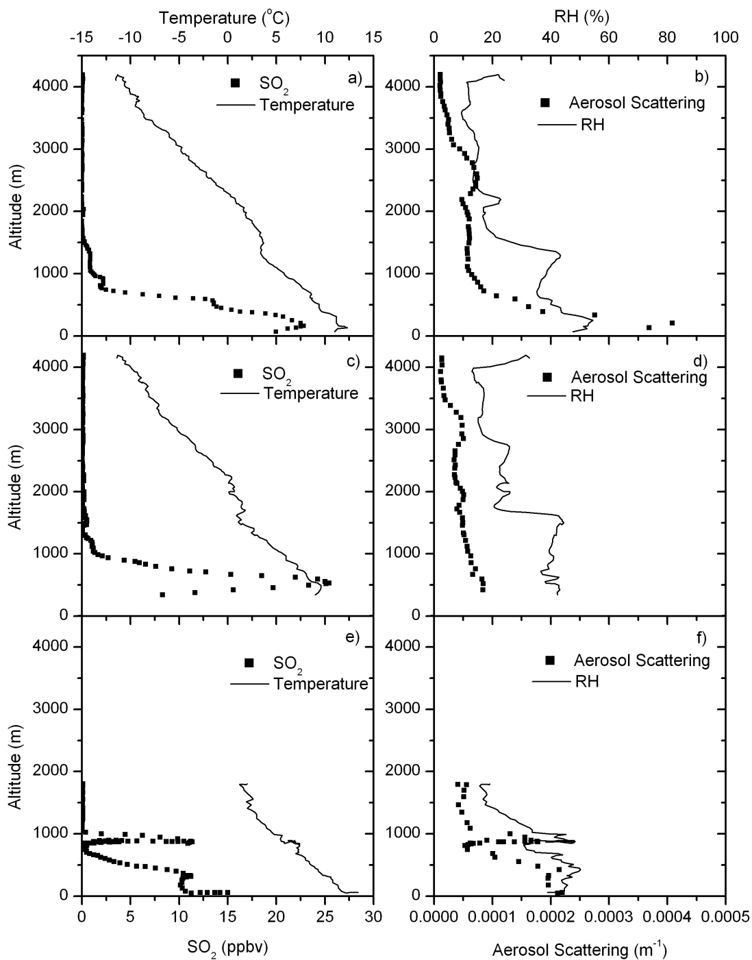
Appendix II.4. Vertical profiles of SO 2 , temperature, aerosol scattering coefficients (550 nm) and relative humidity on April 11, 2005. Panels a) and b) present data obtained from a spiral ascent south of Shenyang (41.35°N 122.65°E). Panels c) and d) present data obtained from a spiral ascent south of Shenyang (42.45°N 123.61°E). Panels e) and f) present data obtained when descending to the airport (41.64°N 123.49°E).
