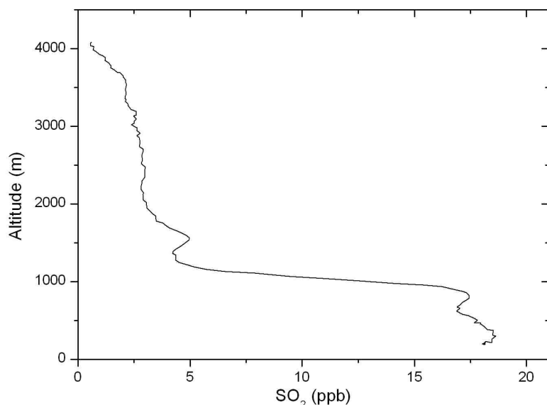
Figure 4.10. Vertical profile of SO 2 , for the morning (~11:30 LST) flight S of Shenyang on April 5, 2005. Note the high SO 2 level in PBL. Above the inversion layer SO 2 drops off quickly but remains almost 3 ppb between 2000 and 3000 m. The profile north of Shenyang (Appendix II) shows less but still around 1 ppb of SO 2 at the same altitudes.
