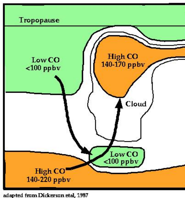
Figure 1. 8. Schematic of CO redistribution by a deep convective process [Dickerson et al. , 1987].
