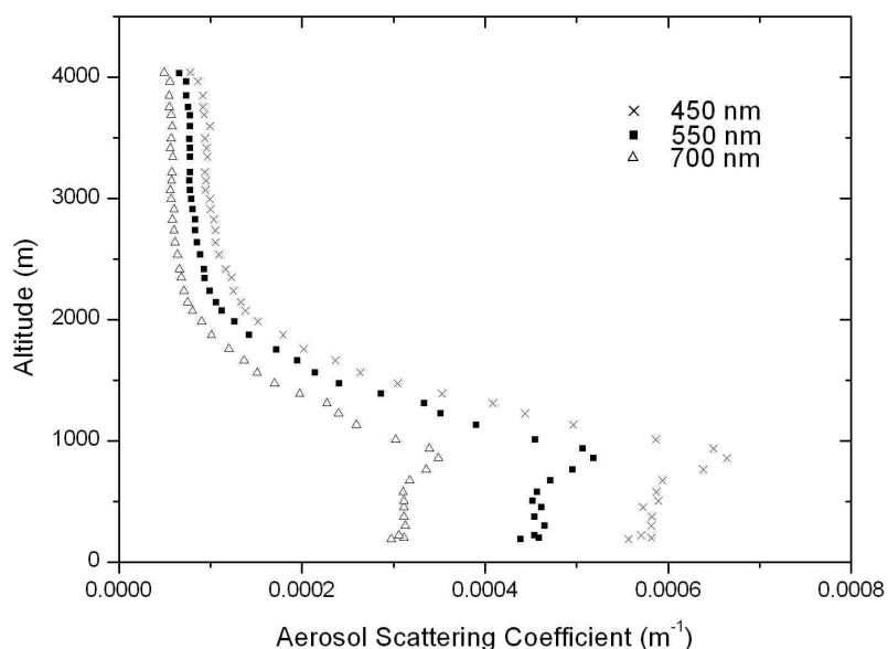
Figure 4.9. Vertical profile of aerosol scattering coefficients, b_{sp} , for the morning (11:30 LST) flight south of Shenyang on 5 April 2005.
