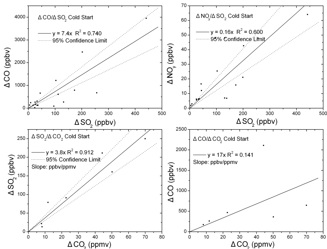
Figure 3.16. Same as Figure 3.15, but for cold start data.
