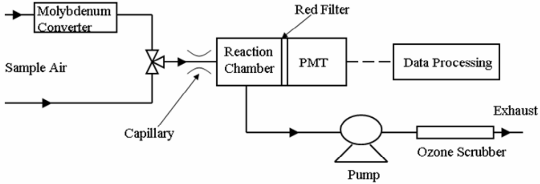
Figure 2.6. Schematic diagram of the modified NO/NO y detector (adapted from [Chen, 2002]).
