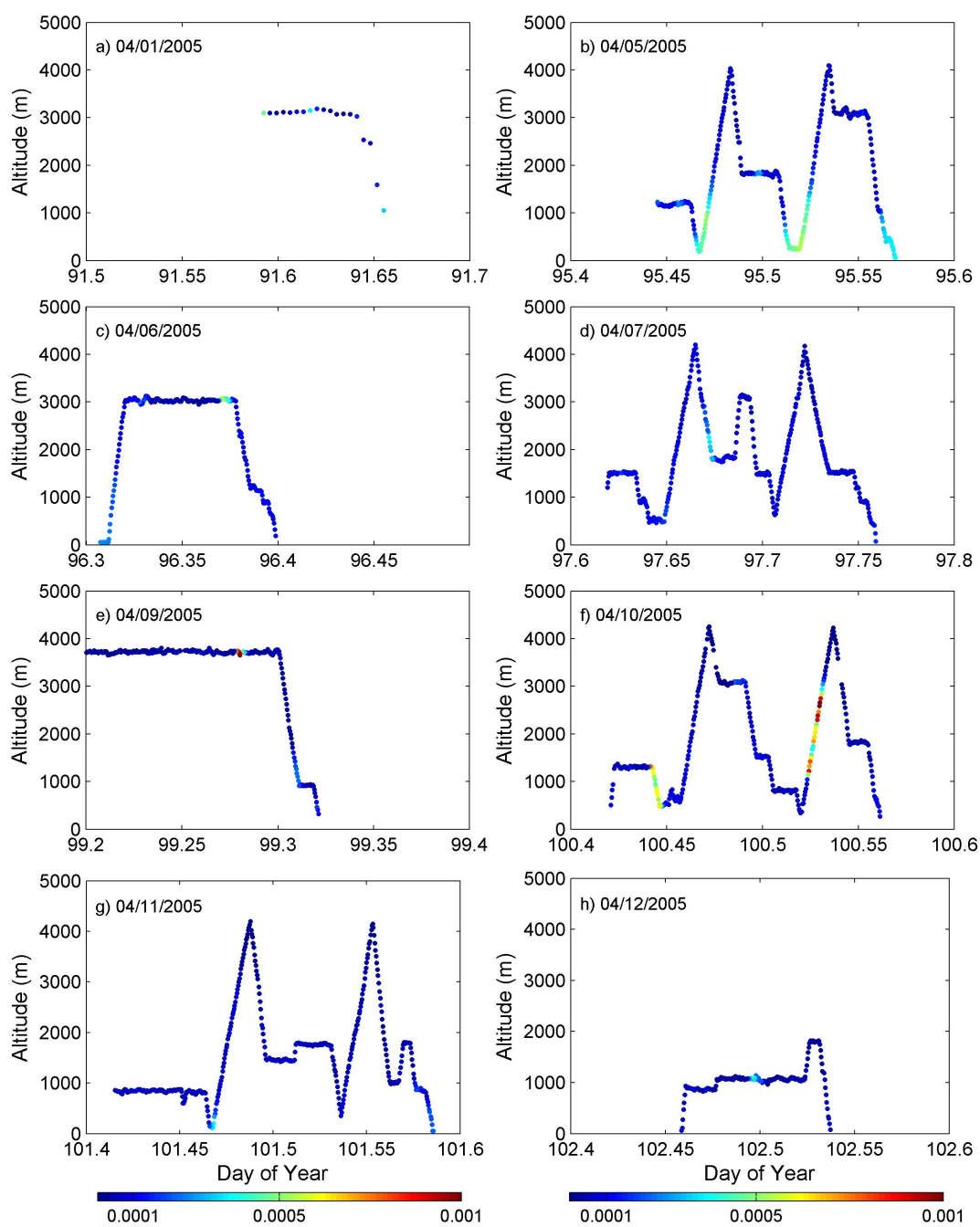
Figure 4.3. Flight altitudes and aerosol scattering at 550 nm (color, unit: \text{m}^{-1} ) along the flight tracks during the Shenyang aircraft campaign.
