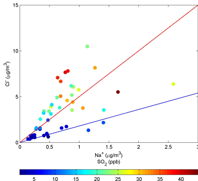
Figure 3.12. Scatter plot of \text{Cl}^- and \text{Na}^+ concentrations. The color of the dots represents the average \text{SO}_2 for the corresponding samples. Blue (slope = 1.8) and red (slope = 5) solid lines are for reference only.
