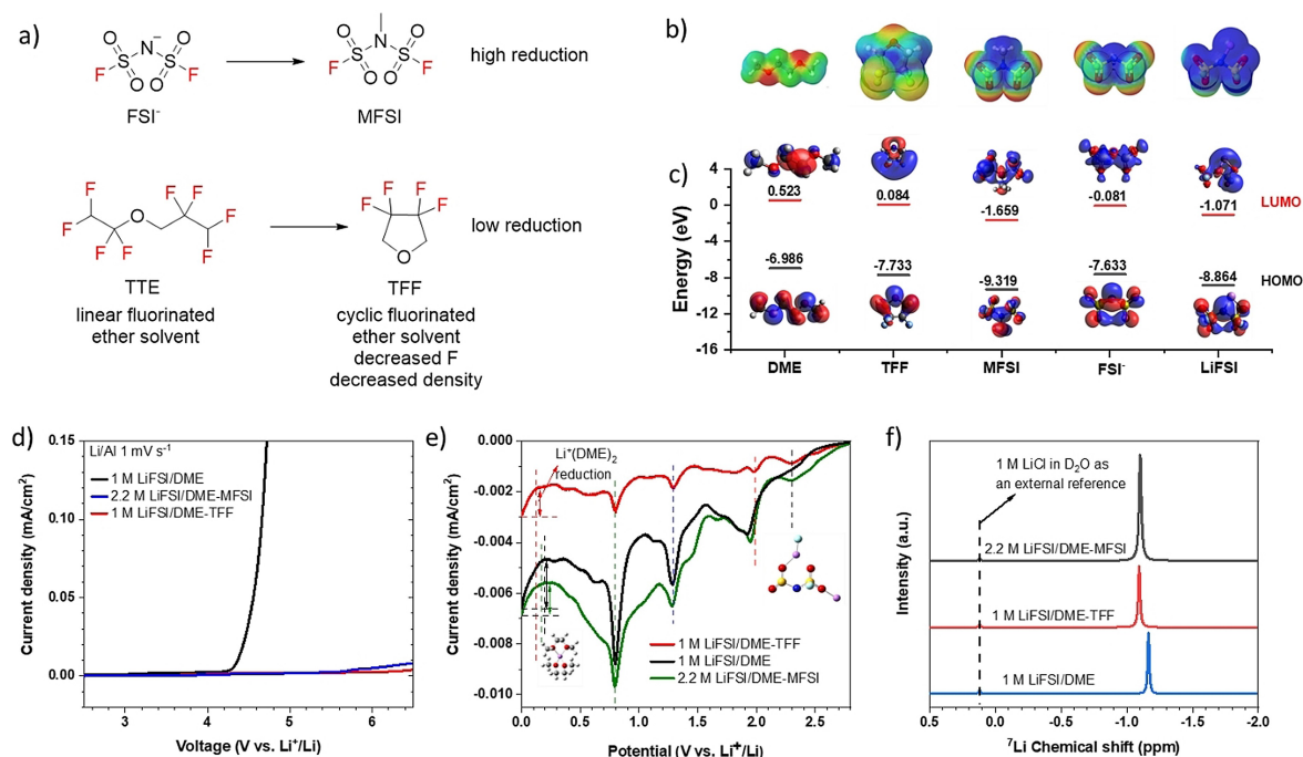
Figure 1. a) Design scheme and the molecular structures of MFSI and TFF; b) ESP surfaces, the ESP surfaces were depicted in the range of -0.1 to 0.1 . The red and blue regions represent a negative charge and positive charge, respectively; c) HOMO and LUMO of DME, TFF, MFSI, FSI - , and LiFSI; d) LSV of three electrolytes in Li||Al half cells at 1 \text{ mV s}^{-1} ; e) LSV reduction of Li||Cu cells at a scan rate of 0.2 \text{ mV s}^{-1} from 2.8 \text{ V} to 0 \text{ V} ; f) ^7\text{Li} NMR of three different electrolytes.
