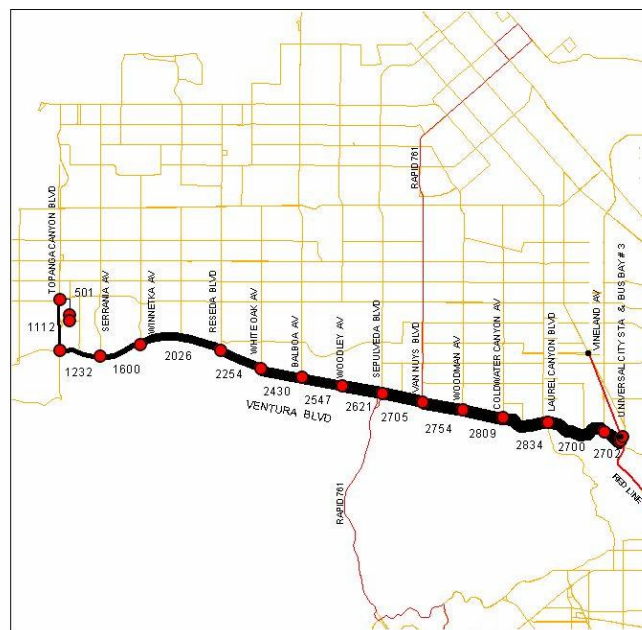
Figure 4.8-9: Transit flow map, along rapid bus routes, Ventura corridor, 2003
