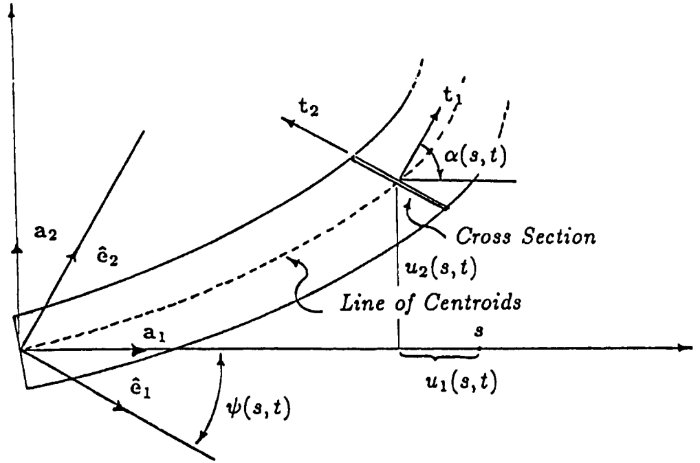
Figure 2.1. The Geometry of the Rod Model.
