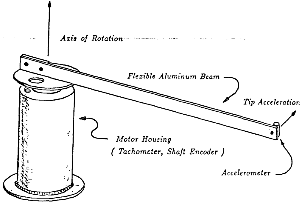
Figure 3.1. Planar Rigid Body and Flexible Appendage Experiment.
