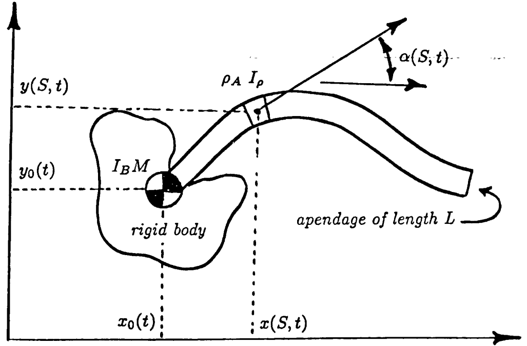
Figure 2.2. A Planar Rigid Body and Rod Configuration.
