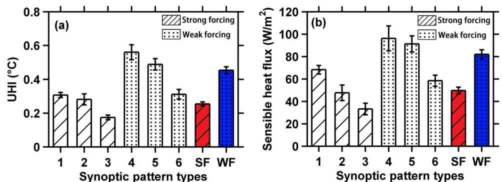
Figure 6. (a) Urban heat island (UHI) intensity (unit: ^{\circ}\text{C} ), and (b) Surface sensible heat flux ( \text{W/m}^2 ) for different synoptic pattern types and weather forcings. SF and WF stand for strong and weak forcings, respectively, and the colored bars for SF (WF) denote the results of the combined average of types 1, 2, 3 (types 4, 5, 6).
