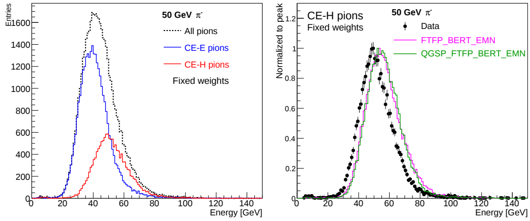
Figure 13. Energy measured for 50 GeV CE-E pions, CE-H pions, and all pions (left), and energy measured for 50 GeV CE-H pions and simulation (right).
