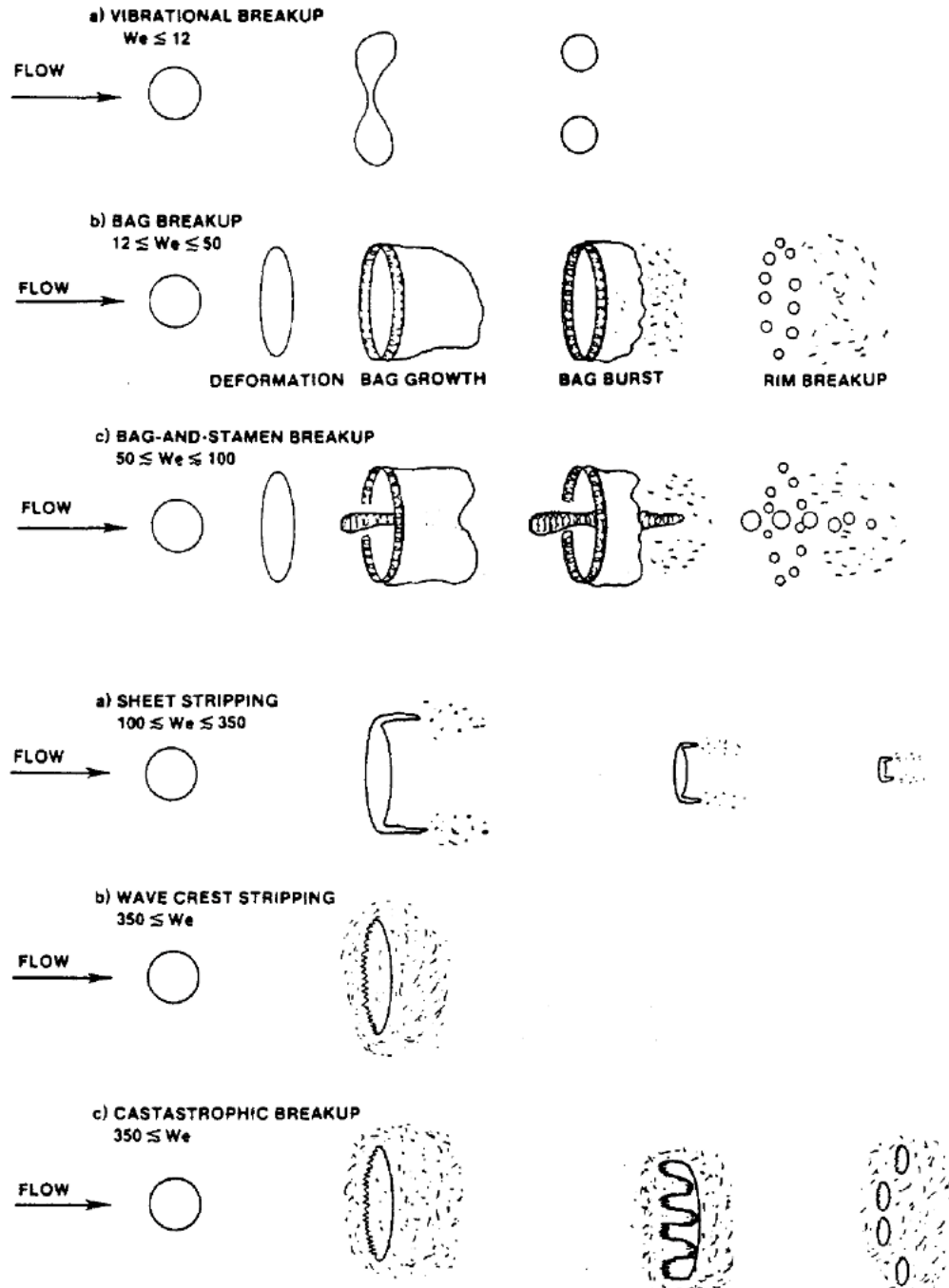
Figure 2.5.1 Breakup mechanisms [62]
