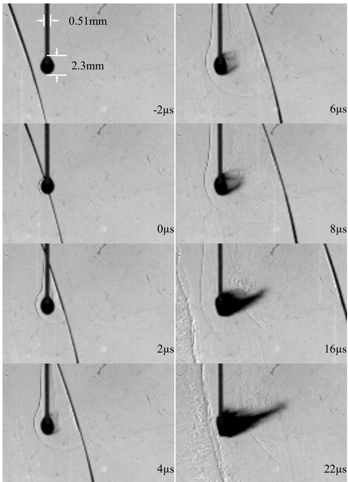
Figure 5.4.1 Lead shock wave, decoupled from the flame fronts, propagating over a suspended ethanol droplet
