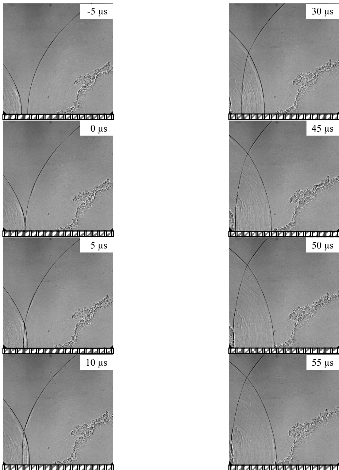
Figure D.1: Sequence of counter propagating decoupled shock-flame wave from t=-5\mu\text{s} to t=55\mu\text{s}
