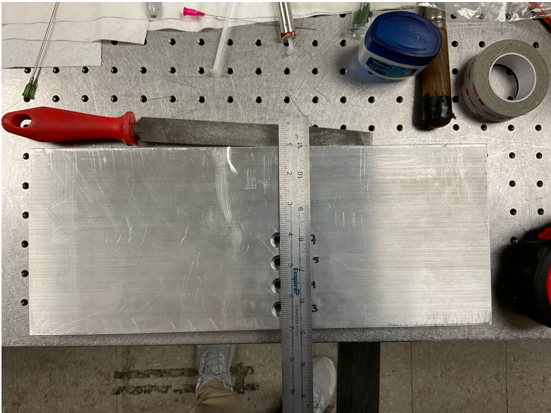
Figure A.3.2: Vertical array of pressure measurement taps on the metal window
