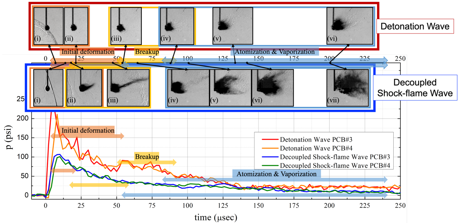
Figure 5.5.5 Pressure measurement for detonation wave and decoupled shock-flame wave cases until 200μs
