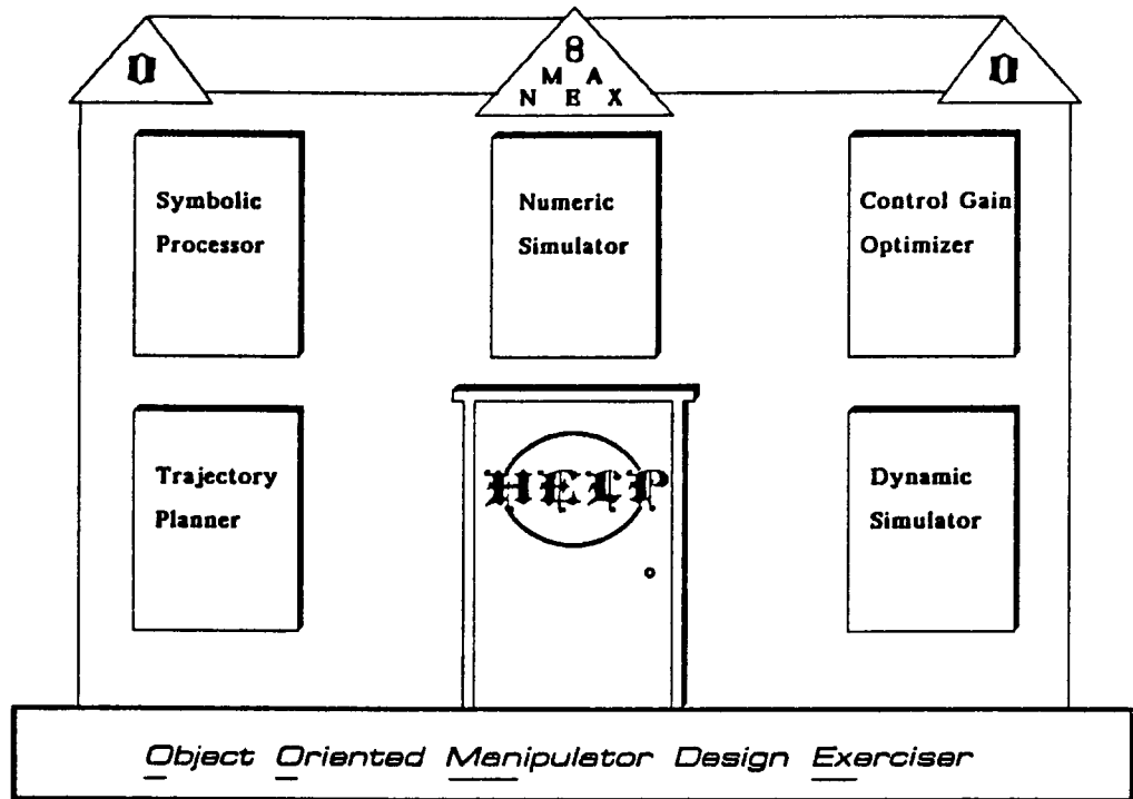
Figure 6. OOMANEX's User Interface
