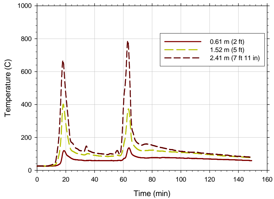
(c) Temperature in Room of Origin
