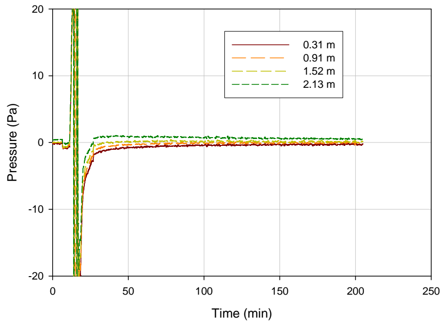
Figure 9-4. Test S1 (sofa, no ventilation) pressures in room of origin (living room)
