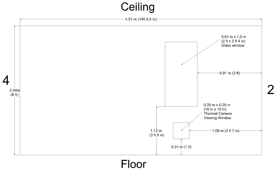
Figure A-5. Elevation View of Wall 3
