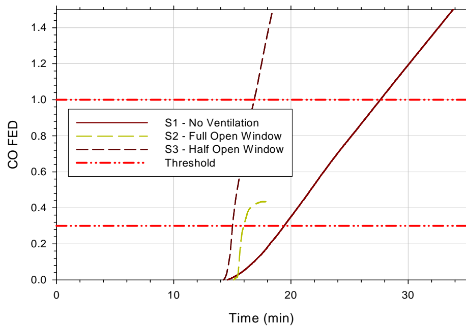
Figure 7-17. CO FED for sofa tests at 1.52 m (5 ft) in the living room.
