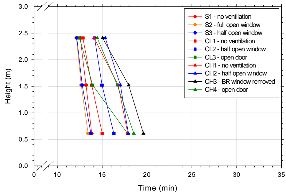
Figure 6-7. Time to 0.43 optical density per meter at sample elevations in the bedroom for all tests
