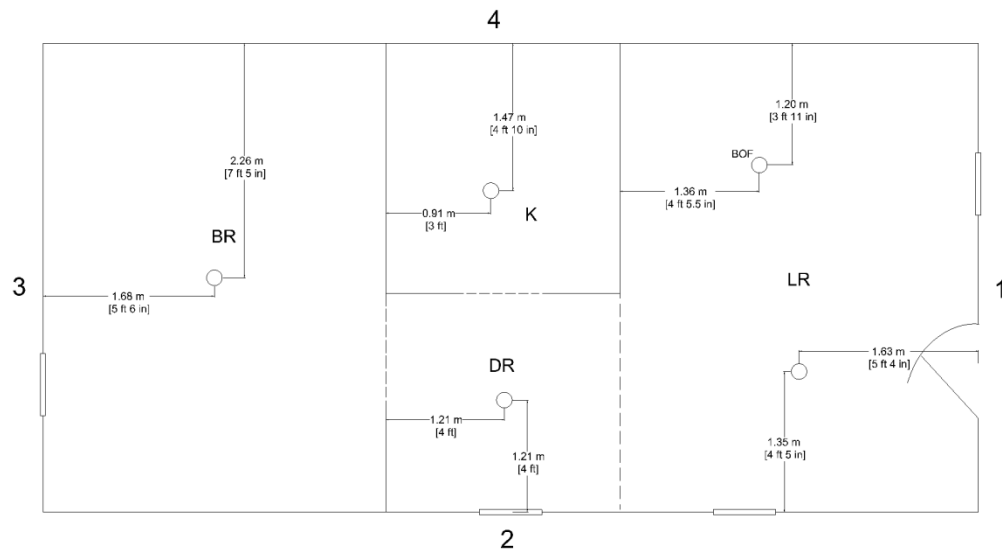
Figure 4-9: Gas Sampling Probe Locations
