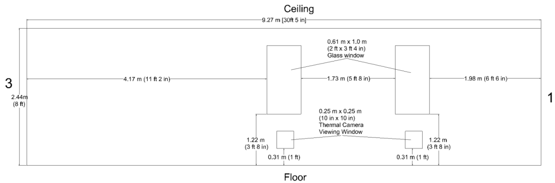
Figure A-4. Elevation View of Wall 2
