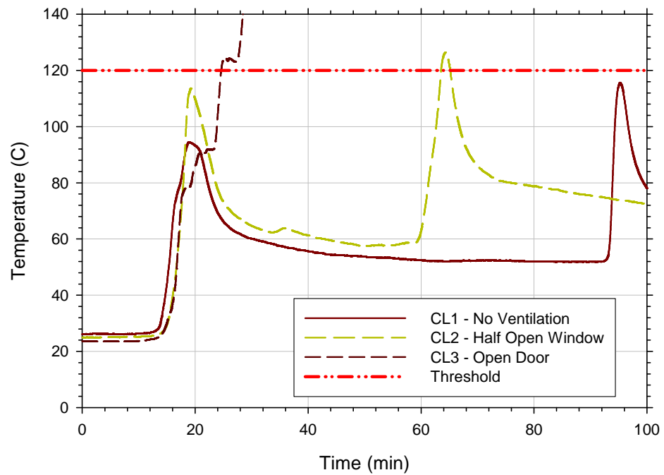
Figure 7-20. Temperature for low cabinet tests at 1.52 m (5 ft) in the bedroom
