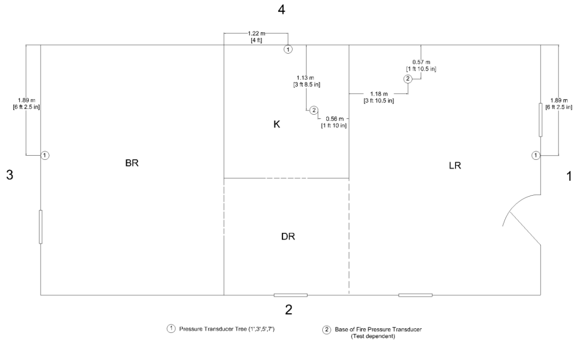
Figure 4-6: Pressure Transducer Locations
