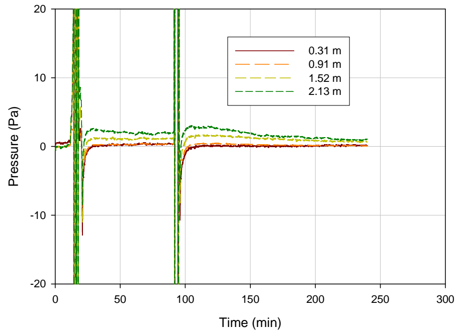
Figure 9-12. Test CL1 (low cabinets, no ventilation) pressures in room of origin (kitchen)
