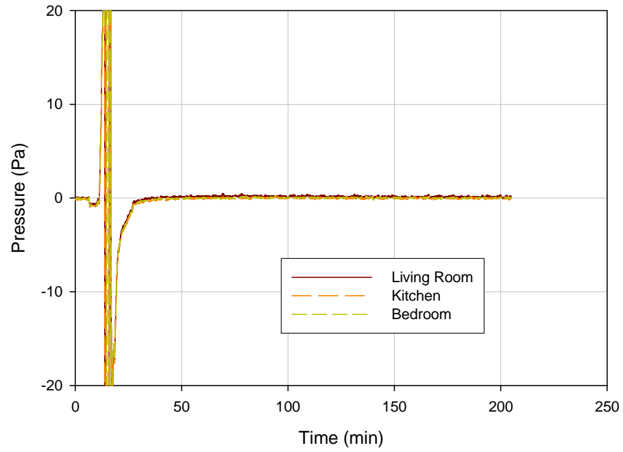
Figure 9-5. Test S1 (sofa, no ventilation) pressure comparison at 1.52 m
