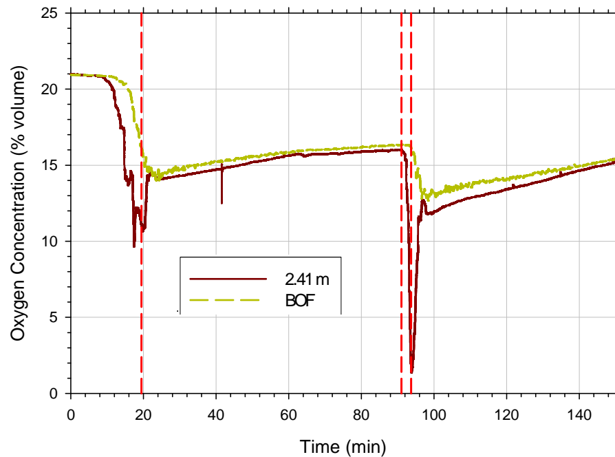
Figure 6-4. Oxygen concentration method of determining LOI at base of fire (BOF) for test CL1
