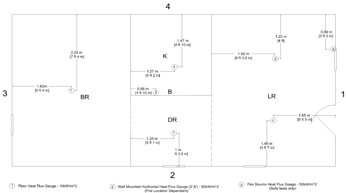
Figure 4-5: Heat Flux Transducer Locations
