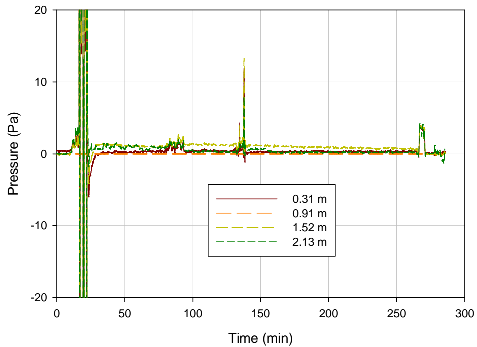
Figure 9-18. Test CH1 (high cabinets, no ventilation) pressures in rom of origin (kitchen)
