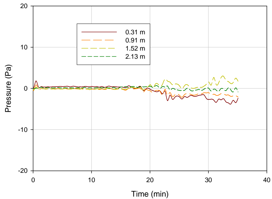
Figure 9-20. Test CH3 (high cabinets, window removed) pressures in room of origin (kitchen)
