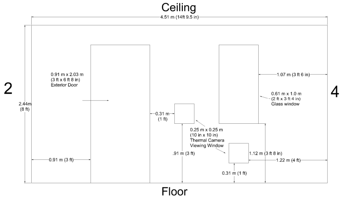
Figure A-3. Elevation view of Wall 1
