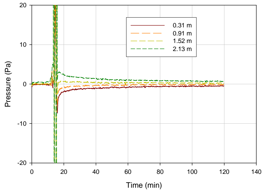
Figure 9-6. Test S3 (sofa, half open window) pressures in room of origin (living room)
