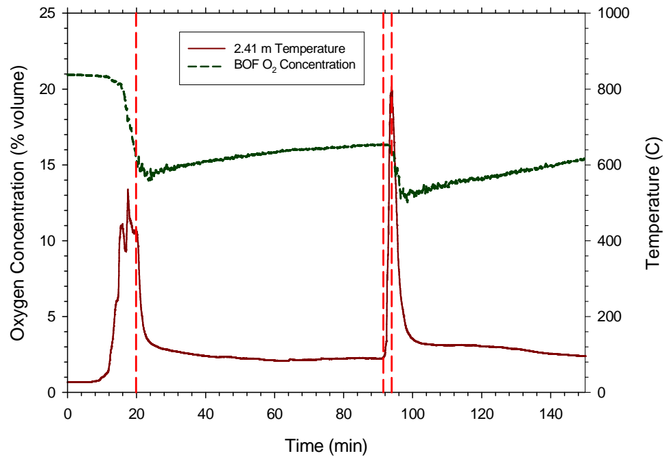
Figure 6-5. Temperature method of determining LOI for test CL1
