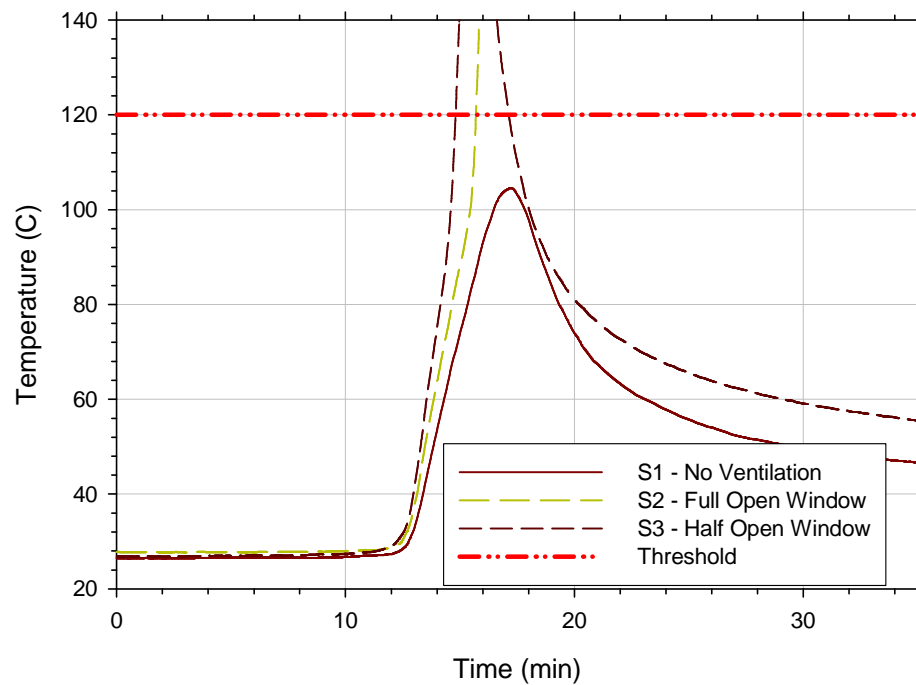
Figure 7-15. Temperature for sofa tests at 1.52 m (5 ft) in the bedroom
