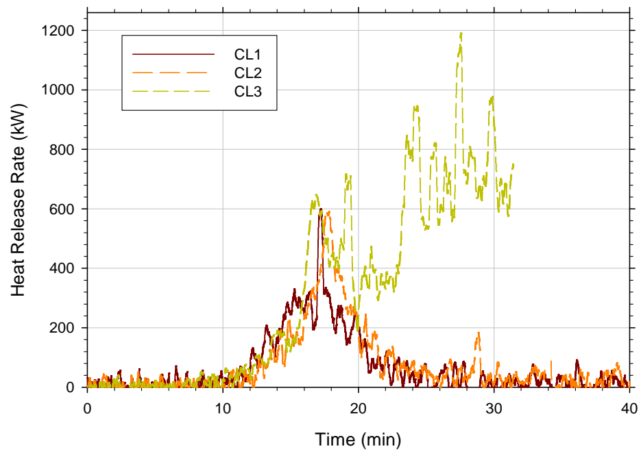
Figure 6-2. Initial HRR development for low cabinet fires
