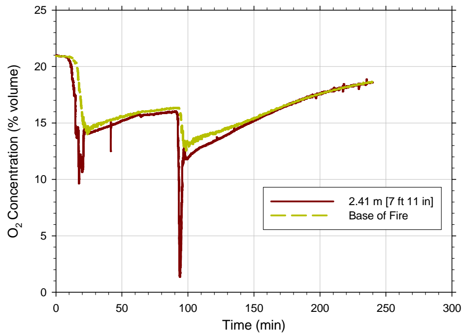
(b) Oxygen Concentrations in Room of Origin
