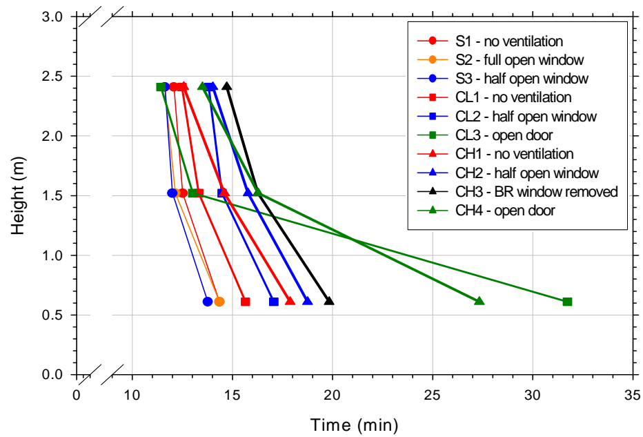
Figure 6-6. Time to 0.43 optical density per meter at sample elevations in the living room for all tests
