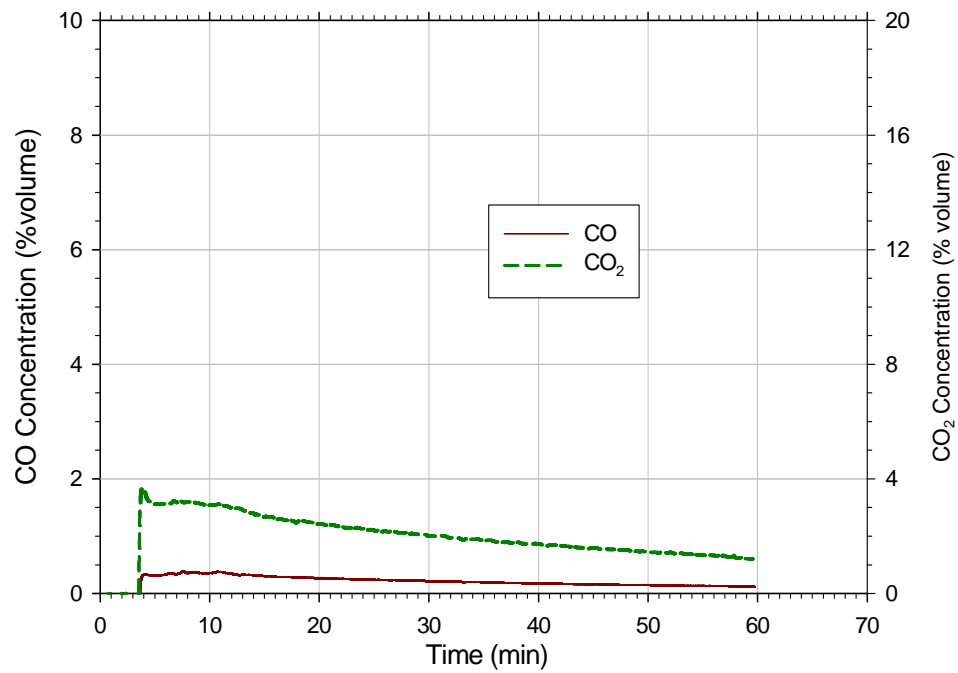
(d) Gas Concentrations at 2.41 m (7 ft 11 in) in Room of Origin
