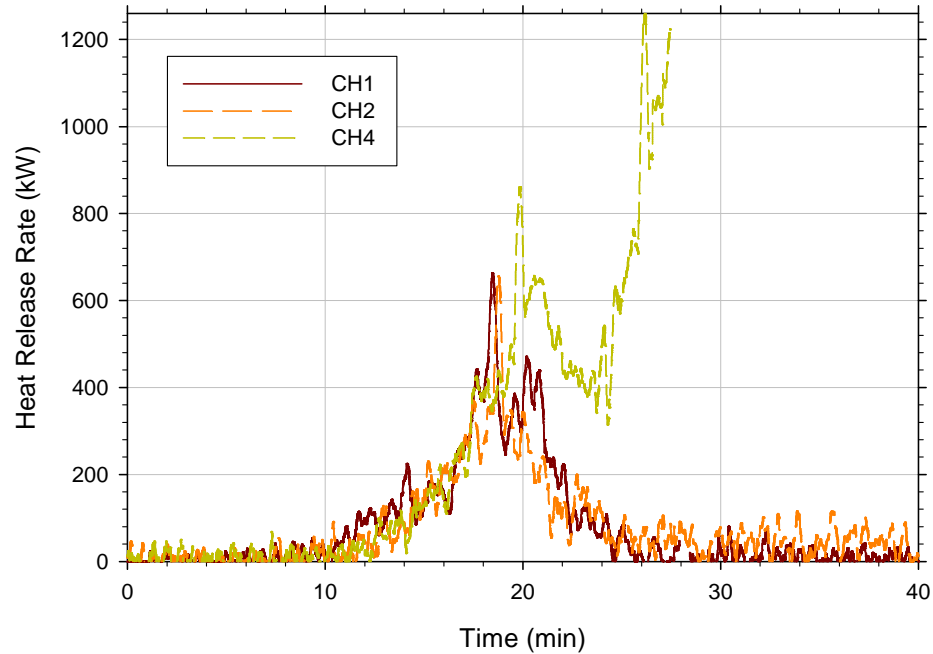
Figure 6-3. Initial HRR development for high cabinet fires
