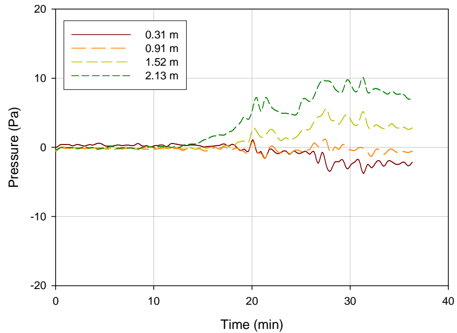
Figure 9-22. Test CH4 (high cabinets, open door) pressures in room of origin (kitchen)
