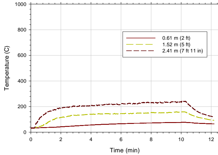
Figure 5-9. Room of origin temperature data for test B2 with a 125 kW natural gas fire and a full open window
