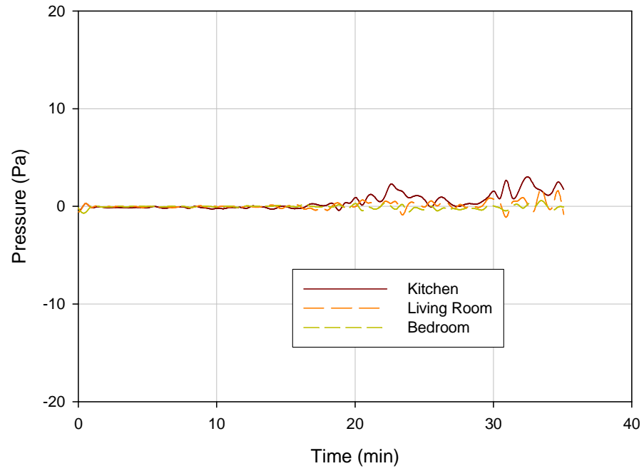
Figure 9-21. Test CH3 (high cabinets, window removed) pressure comparison at 1.52 m
