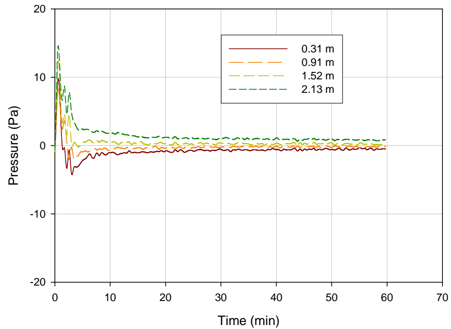
Figure 9-10. Test S4 (sofa, accelerated, half open window) pressure in room of origin (living room)
