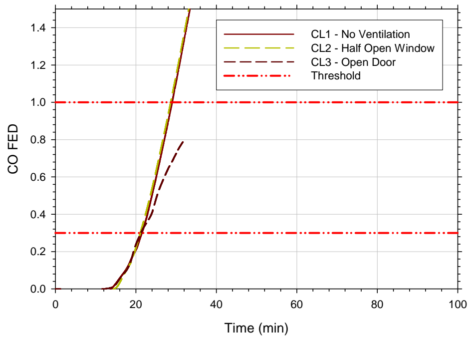
Figure 7-22. CO FED for low cabinet tests at 1.52 m (5 ft) in the bedroom
