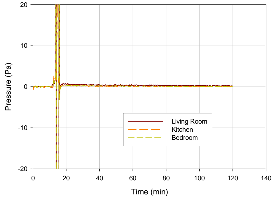
Figure 9-7. Test S3 (sofa, half open window) pressure comparison at 1.52 m
