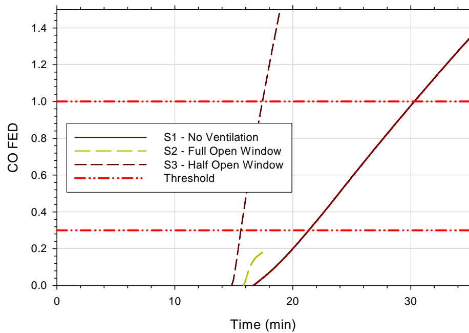
Figure 7-18. CO FED for sofa tests at 1.52 m (5 ft) in the bedroom
