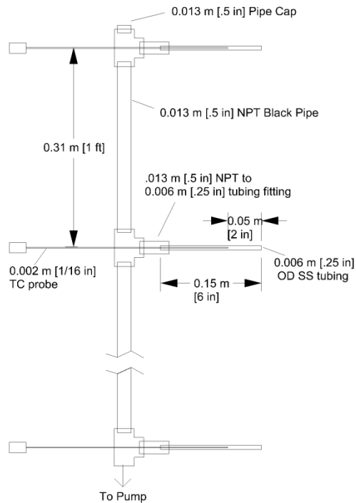
Figure 4-3: ATC Tree Detailed Layout
