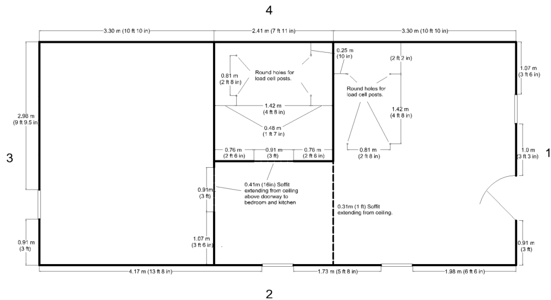
Figure A-1. Plan view with room and overall enclosure dimensions. Bold letters and numbers indicate naming conventions for exterior and interior walls. All dimensions given reflect interior dimensions.
