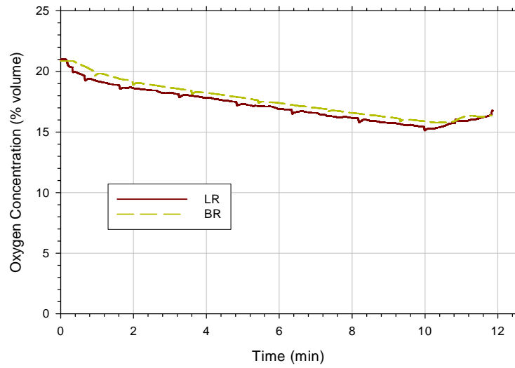
Figure 5-10. Oxygen concentration data for test B2 with a 125 kW natural gas fire and a full open window
