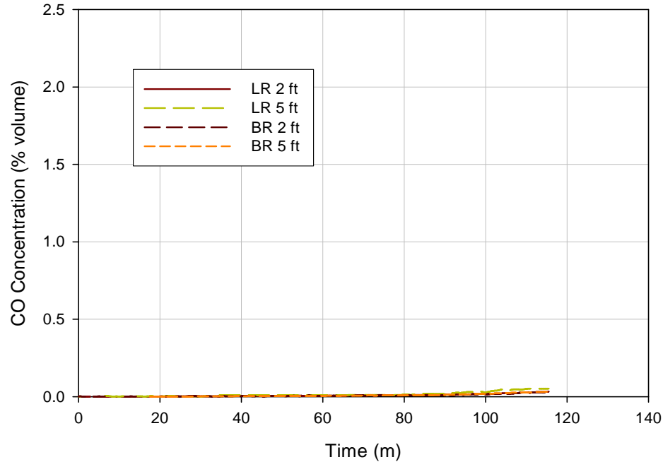
Figure 7-2. Test SM4 (smoldering sofa, no ventilation) CO concentrations
