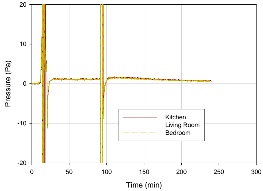
Figure 9-13. Test CL1 (low cabinets, no ventilation) pressure comparisons at 1.52 m
