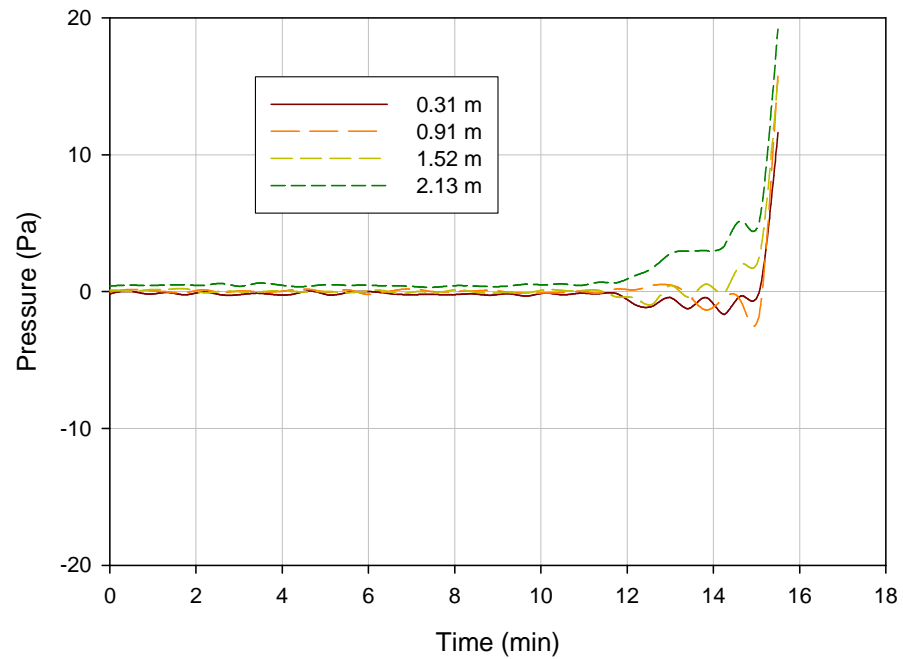
Figure 9-8. Test S2 (sofa, full open window) pressures in room of origin (living room)
