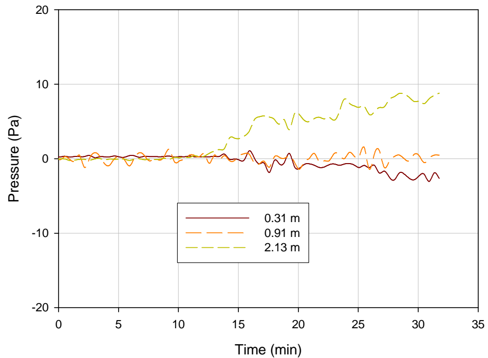
Figure 9-16. Test CL3 (low cabinets, open door) pressures in room of origin (kitchen)
