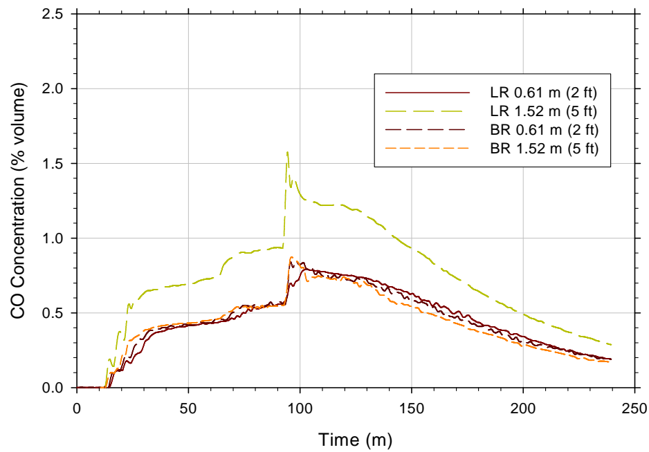
b) CO Concentrations Along Path of Egress
