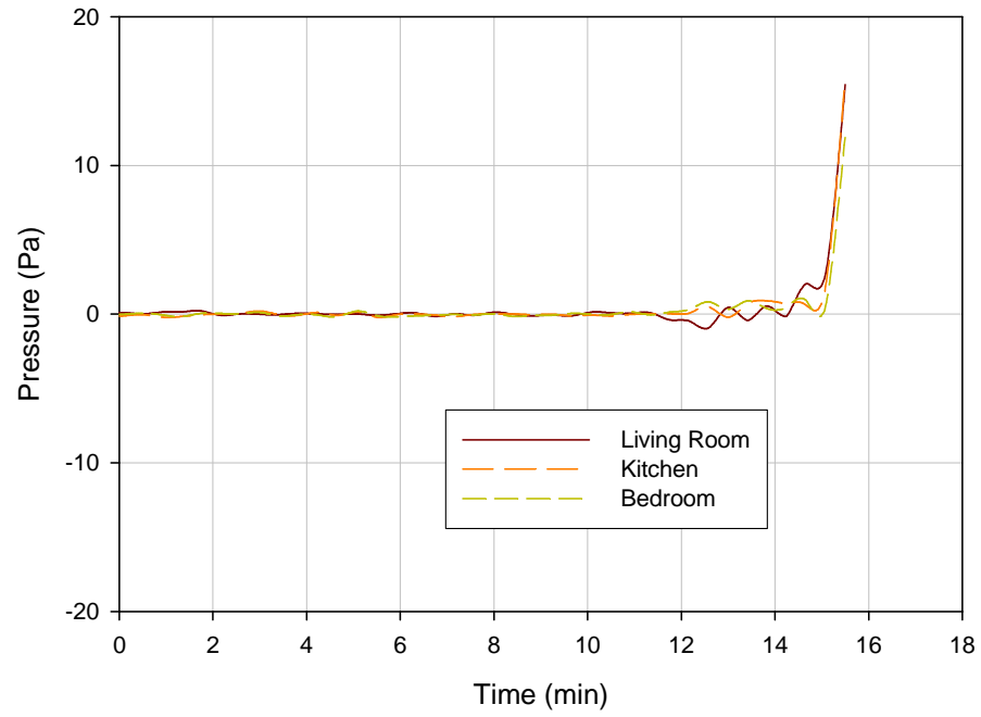
Figure 9-9. Test S2 (sofa, full open window) pressure comparisons at 1.52 m
