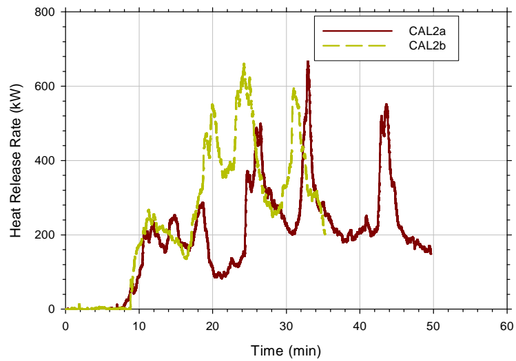
Figure 5-4. Cabinet array heat release rates for test CAL2
