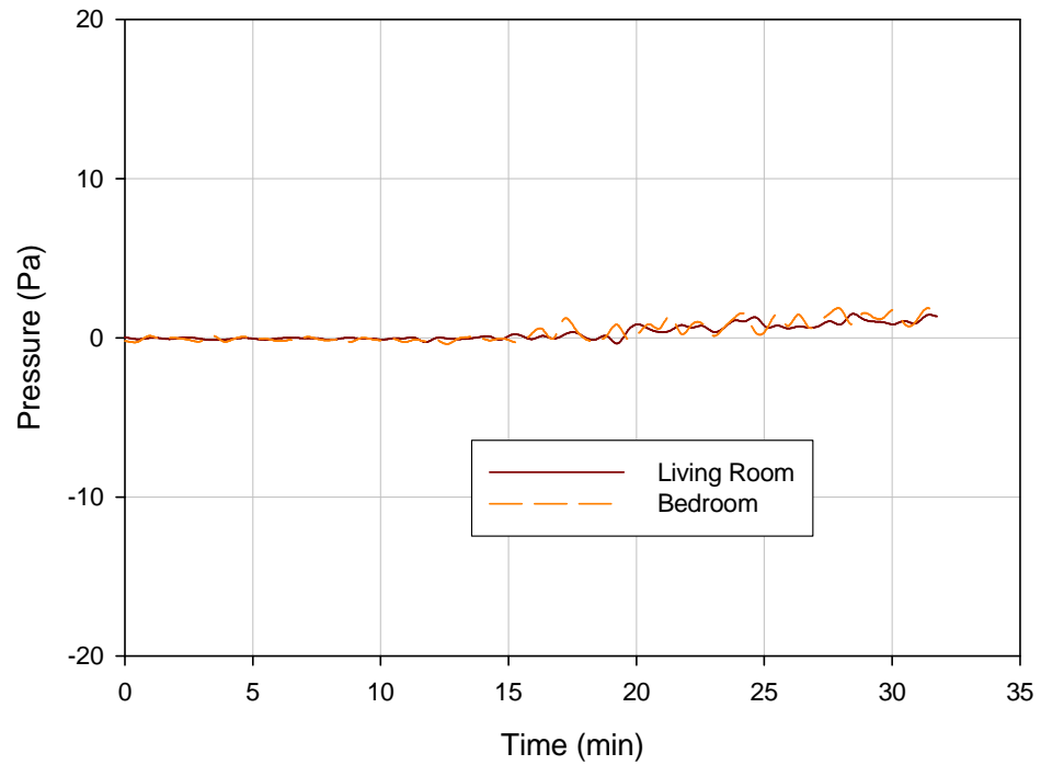
Figure 9-17. Test CL3 (low cabinets, open door) pressure comparison at 1.52 m *The 1.52 m pressure transducer in the kitchen malfunctioned during this test
