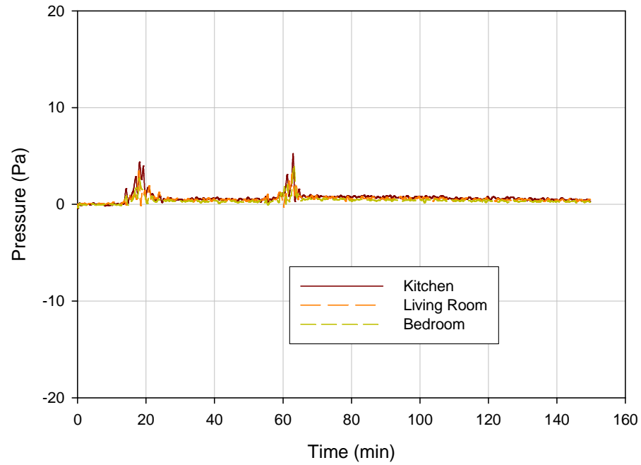
Figure 9-15. Test CL2 (low cabinets, half open window) pressure comparison at 1.52 m
