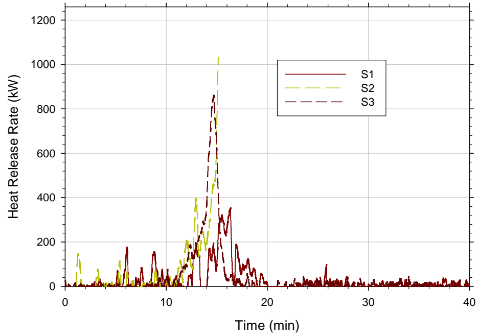
Figure 6-1. Initial HRR development for sofa fires
