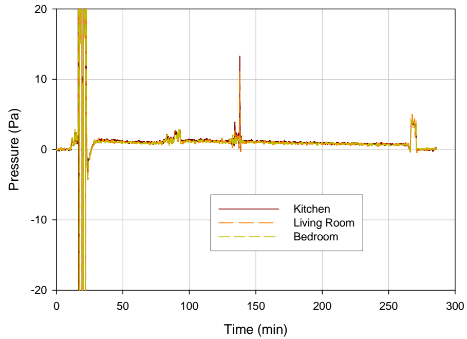
Figure 9-19. Test CH1 (high cabinets, no ventilation) pressure comparison at 1.52 m
