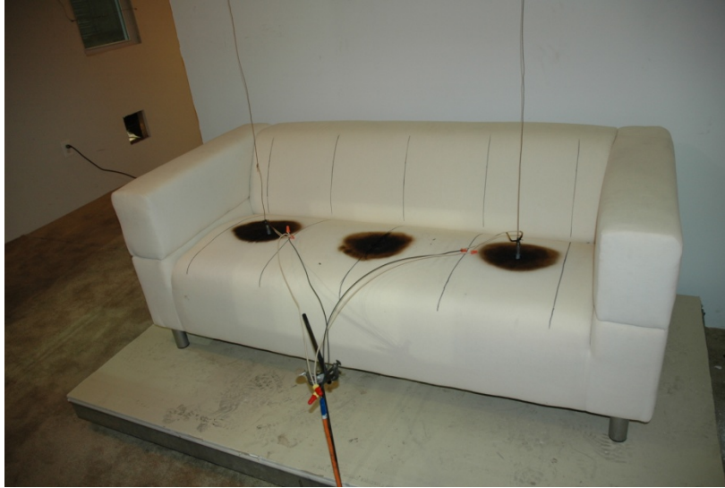
Figure 5-16. Test SM3 damage (the center char area is from test SM2)
