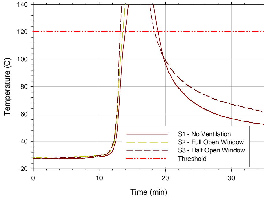
Figure 7-14. Temperature for sofa tests at 1.52 m (5 ft) in the living room (room of origin)
