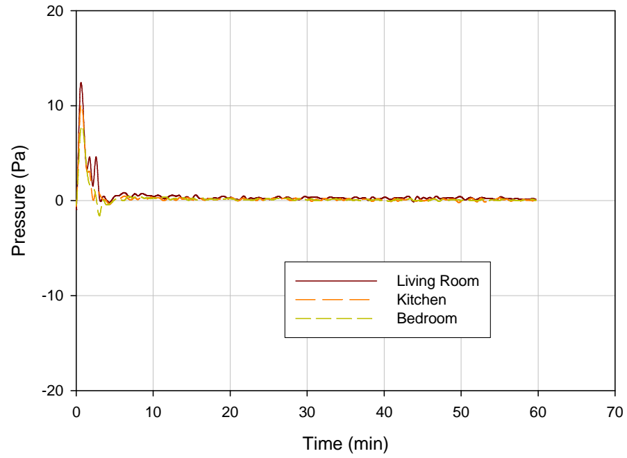
Figure 9-11. Test S4 (sofa, accelerated, half open window) pressure comparisons at 1.52 m
