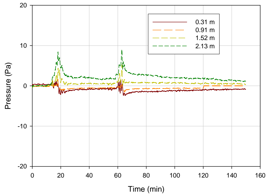
Figure 9-14. Test CL2 (low cabinets, half open window) pressures in room of origin (kitchen)
