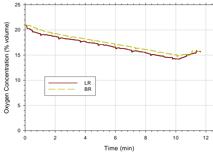
Figure 5-8. Oxygen concentration data for test B1 with a 125 kW natural gas fire and no ventilation
