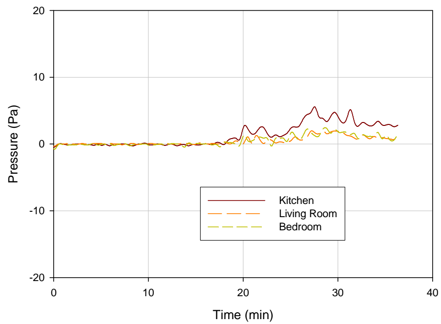
Figure 9-23. Test CH4 (high cabinets, open door) pressure comparison at 1.52 m
