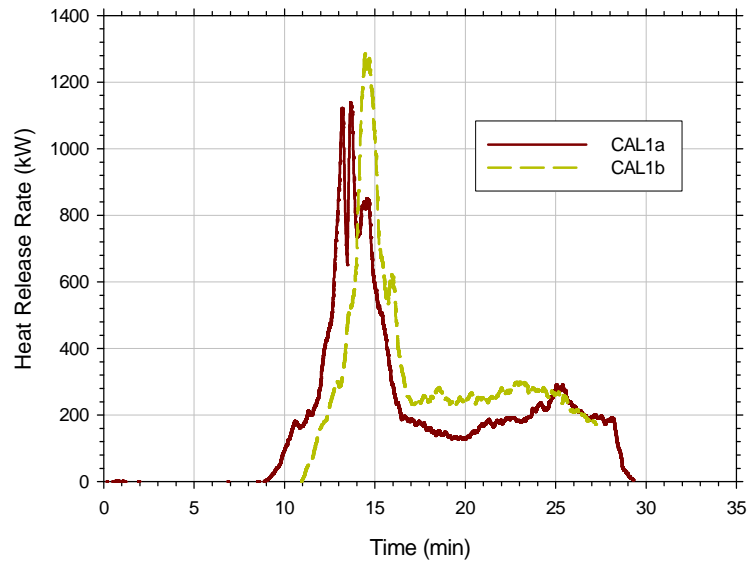
Figure 5-3. Sofa heat release rates for test CAL1
