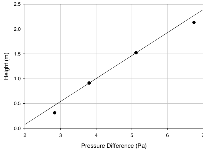
Figure 9-3. Pressure difference determination for test S3 at 14.16 seconds
