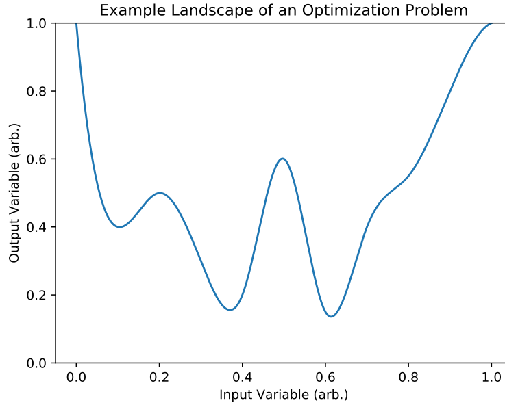
Figure 2.6: Example Landscape of an Optimization Problem. In this simple example, there is only one independent variable (variable that can be changed), and there are many local minima. The global minimum is x \approx 0.6 .
