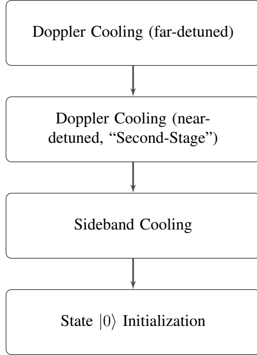
Figure 3.11: Sequence of Qubit State Initialization. These are the steps from Section 3.6.2.2 .
