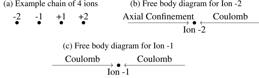
Figure 3.7: Diagram of forces on 4 ions in a chain. The horizontal direction is along \hat{X} , i.e. along the axis of the ion trap. The forces on Ions +1 and +2 are symmetric to the forces on Ions -1 and -2, respectively. These free body diagrams omit gravity, the RF confinement of the ion trap, and micromotion.
