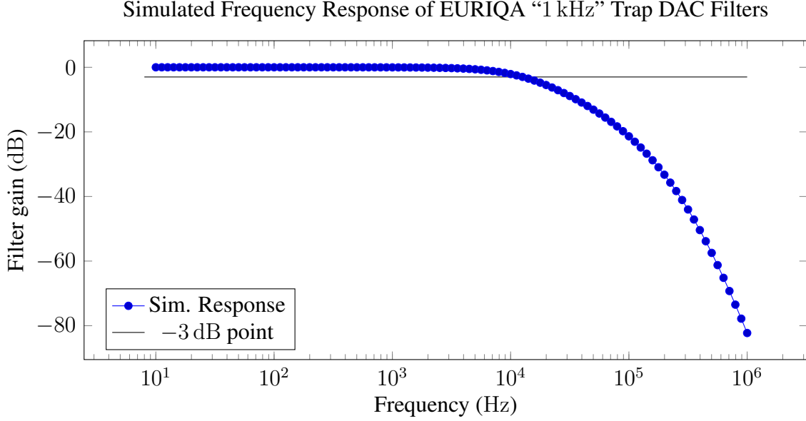
Figure 4.2: Simulated Frequency Response of EURIQA \approx 1 kHz Filter. This is a straightforward 5th-order lowpass RC filter.
