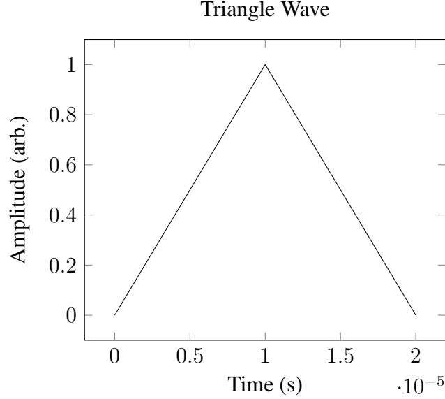
Figure 5.1: Example Triangle Wave Amplitude. The ramp-up can be described by A(t) = t , or CubicSpline( c_0 = 0.0, c_1 = 1.0, c_2 = 0.0, c_3 = 0.0 ) . The ramp-down can be described by A(t) = 1 - t (where t = 0 is referenced to the start of the ramp-down pulse), which is equivalent to CubicSpline( c_0 = 1.0, c_1 = -1.0, c_2 = 0.0, c_3 = 0.0 ) . Similar pulses, comprised of up to cubic (3rd-order) polynomials, could be equally well-represented by a pair of CubicSplines.
