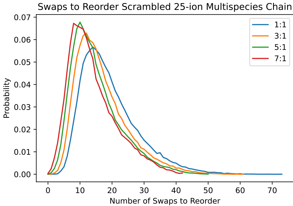
Figure 8.5: Effect of ratio of computational to coolant ions on the number of swaps needed to sort a scrambled 25-ion chain. Number of trials per coolant ratio is 100000. Each line is the bars from Fig. 8.3, but plotted as a line instead of a bar for visibility. Note that as the ratio of computational to coolant ions increases, the observed “tail” also decreases, implying that the worst-case number of swaps also decreases (or is at least made more unlikely).
