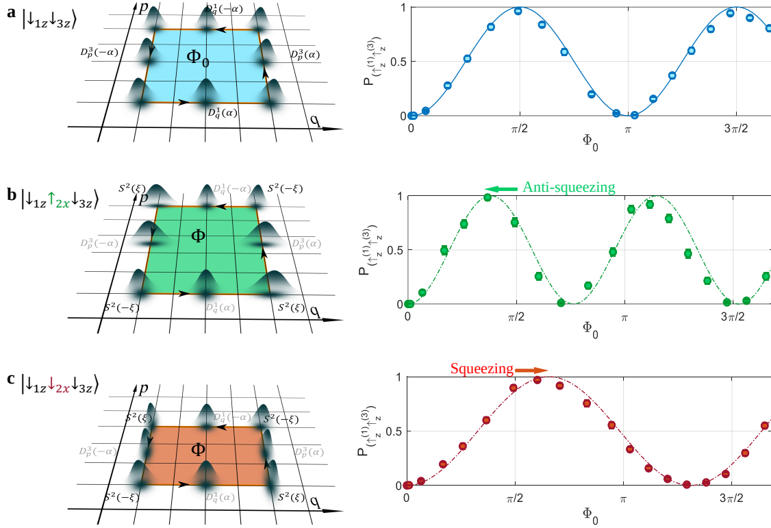
Figure 7.3: Demonstration of Quantum phase-gates on three ions. a , Mølmer-Sørensen gate between ions number 1 and 3 using displacement operations of one phonon mode using Milburn's scheme [131] as illustrated in Fig. 7.2 (a). The phase-space area of the enclosed rectangular contour \Phi_0 controls the spin evolution, jointly flipping the initial state |\downarrow_z^{(1)}\downarrow_z^{(3)}\rangle into the state |\uparrow_z^{(1)}\uparrow_z^{(3)}\rangle . D_q^{(n)}(\alpha) and D_p^{(n)}(\alpha) denote position and momentum displacement operations. b-c , Interspersing spin-dependent squeezing operations S^{(2)}(\pm\xi) on ion number 2 in-between displacement stages along the p coordinate scales the accumulated phase-space area \Phi conditioned on the state of that spin (c.f. Eq. (7.6)). (a-c) , The phonon wavepacket is brought back to its original state at the end of the gate operation to erase the spin-phonon correlations developed during the gate. Circles represent measured data, bars represent 1\sigma binomial uncertainties, and dash-dot lines are the analytically calculated Unitary evolution for the system parameters estimated independently. The applied experimental sequences are presented in Fig. 7.5 (a-b).
