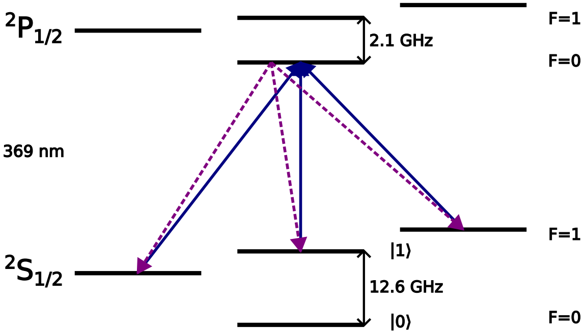
Figure 3.5: ^{171}\text{Yb}^+ Readout State Diagram. Only qubits that are in |1\rangle will be excited to emit light. Blue solid arrows represent driven transitions ( \approx 370 nm) via photon absorption. Dashed purple arrows represent spontaneous photon emission. 935 nm light is not shown here, though it is important to the readout process. The role 935 nm light is to “re-pump” from the ^2D_{3/2} state (which can be entered spontaneously when decaying from ^2P_{1/2} ) to the ^2S_{1/2} |F = 1\rangle manifold. This ensures that the cycling transition will continue to emit light if the qubit is in |1\rangle , instead of stopping whenever the ion enters the ^2D_{3/2} state.
