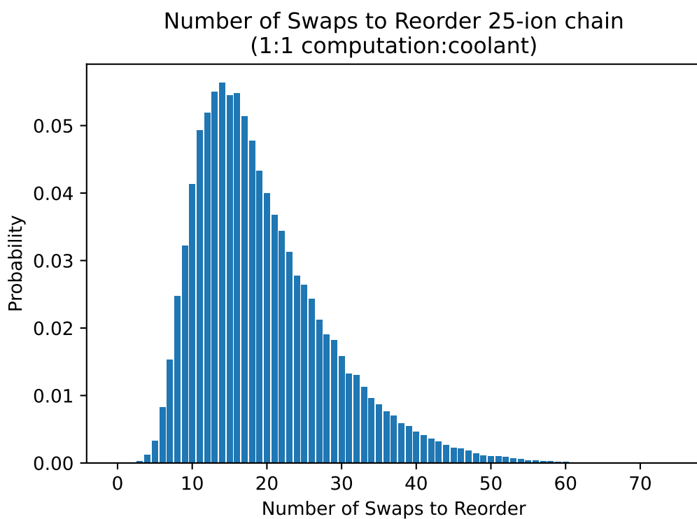
Figure 8.3: Simulation of the number of swaps to reconfigure a randomly-scrambled 25-ion chain, with 1 : 1 computational to coolant ion ratio. This is shown as probability to reflect the random nature of the chain scrambling. Note that the tail of the distribution goes out to almost 70 swaps, approximately a factor of 3.5\times more than the average case.
