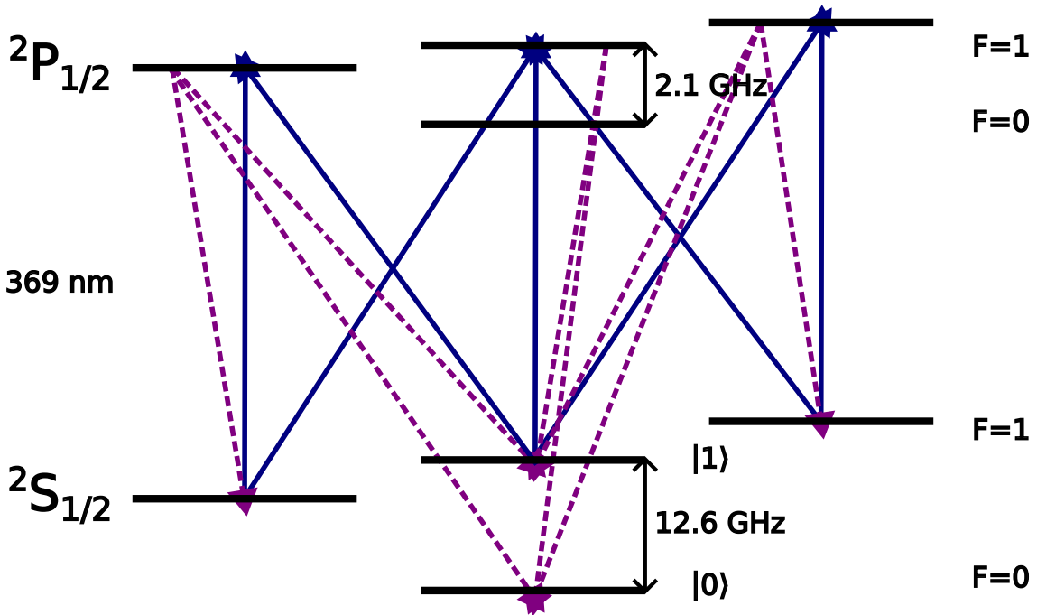
Figure 3.4: ^{171}\text{Yb}^+ Optical Pumping State Diagram. This diagram illustrates the transitions that are needed to pump into the state |0\rangle of ^{171}\text{Yb}^+ ( 2S_{1/2} , |F=0, m_F=0\rangle ). Blue solid arrows represent driven transitions ( \approx 370 nm) via photon absorption. Dashed purple arrows represent spontaneous photon emission. 369 nm and 370 nm are used interchangeably because the transition is near 369.5 nm.
