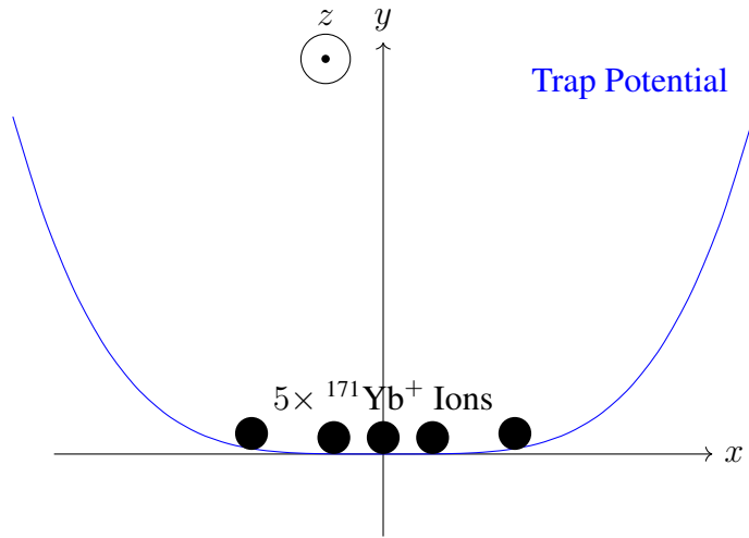
Figure 3.9: Five ions trapped in a quartic potential. Relative to Fig. 3.8, this image has a total of five ions. With several ions, we elect to use a quartic (not harmonic) trapping potential to approximately equally space the ions in the chain from each other. We also use the term “chain” to describe a crystal of \geq 2 ions that are trapped in a well. Having a chain will break symmetry in an axis, so it now makes sense to add the concept of the “trap axis”. In this frame, vibration along the x axis is said to be axial motion, and the vibrational modes in that direction are called the axial modes. With multiple ions, each additional ion will add one motional mode in each axis. Thus, a two-ion chain will have a total of 6 modes; five ions will have a total of 15 modes. For a chain of \geq 2 ions, the axial mode will be the lowest-frequency mode, and generally subject to the highest heating/number of phonons.
