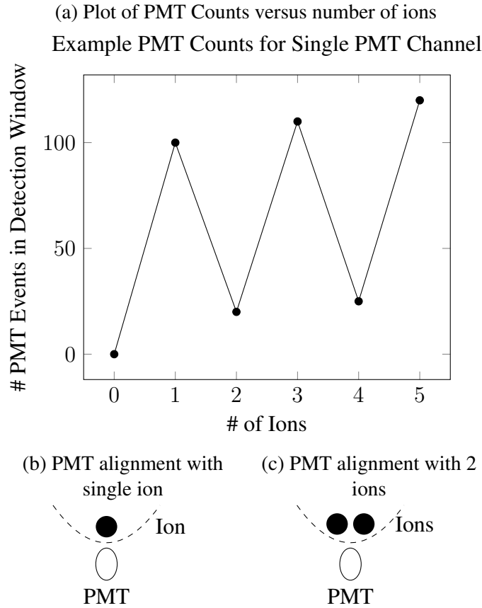
Figure 3.6: Example of light collection aligning then anti-aligning with ion(s). As the number of ions in the well changes from odd to even, the number of photons collected will dramatically drop because the ion chain is no longer aligned with the collection PMT. To visualize this effect, imagine a single PMT imaging the bottom of a parabola (simulating the potential well). With one ion, the bottom of the parabola is aligned with the PMT. With two ions, the ions will repel each other, and now the center of the well will be halfway between the two ions, causing the fluorescence collected by the PMT to drop dramatically. This effect could be mitigated by shifting the center of the well to align to the PMTs as the number of ions changes. However, we take advantage of this effect during loading to produce a strong signal indicating that an ion has been added to the well, indicating success in a loading attempt.
