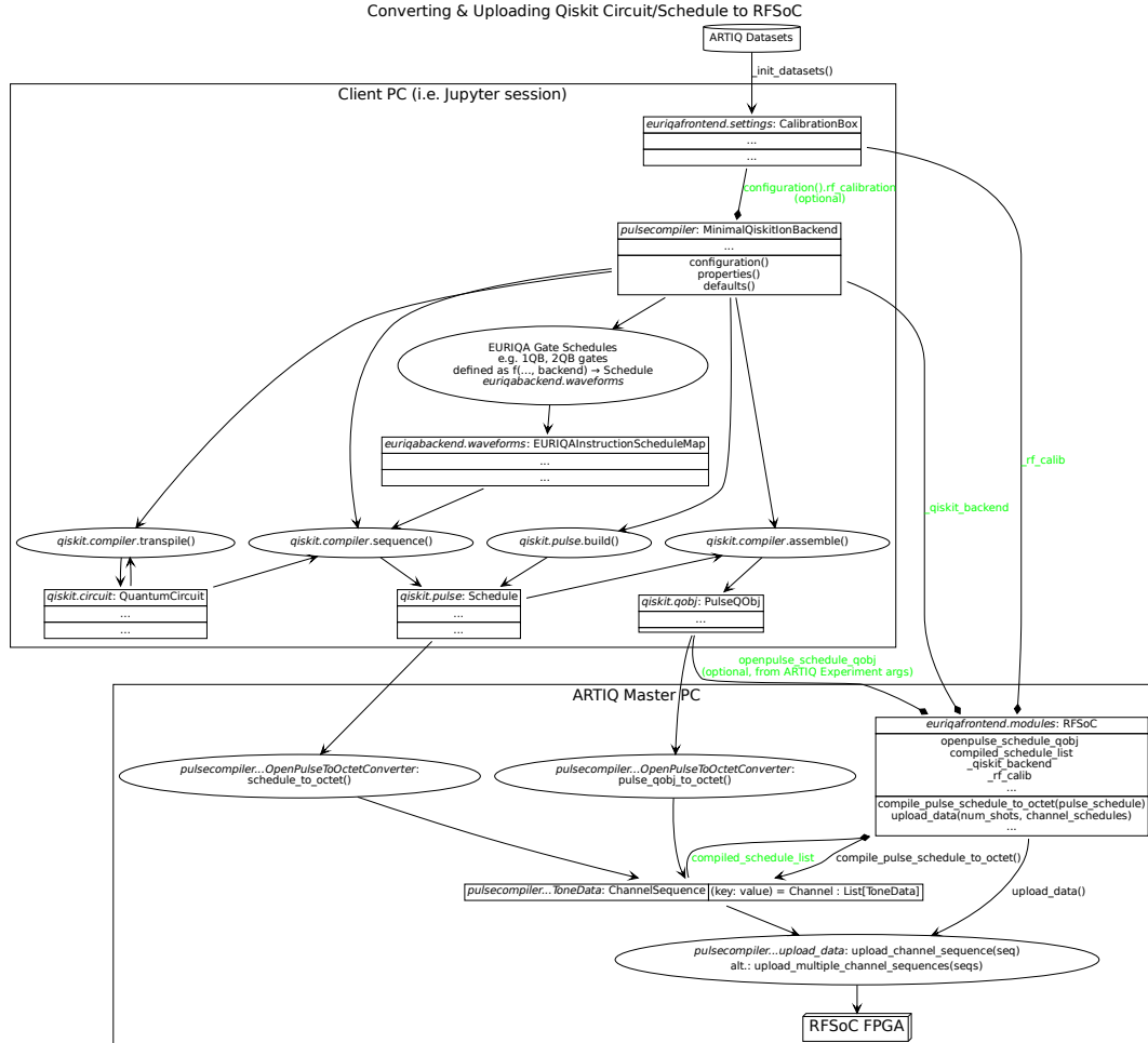
Figure 6.3: Diagram of the different inputs needed to convert a Qiskit QuantumCircuit to a ChannelSequence. Incoming arrows denote inputs to a given entity. Squares are classes, ovals are functions. Italics denote the package that a class/function can be found in. Green text on a diamond arrow denotes that a class attribute (text) of the pointed class is an instance of the arrow's source. Not every class is necessary in this diagram: for instance, the PulseQObj can be bypassed entirely if serialization is not needed, or a CalibrationBox is not needed if your gate waveforms do not require calibrated values.
