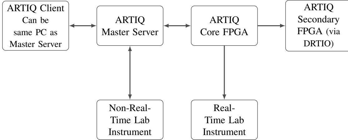
Figure 4.3: Example ARTIQ Laboratory network. Connections between devices indicate that direct communication can be made between the two devices over some protocol (e.g. Ethernet, or a real-time protocol like SPI) during the course of an experiment. Note the direction of (typical) flow is denoted by the arrowhead direction. Practically, the ARTIQ Core FPGA can communicate bidirectionally with any real-time device, but practically the Core FPGA will act as the primary controller/sequencer for any other devices during an experiment.
