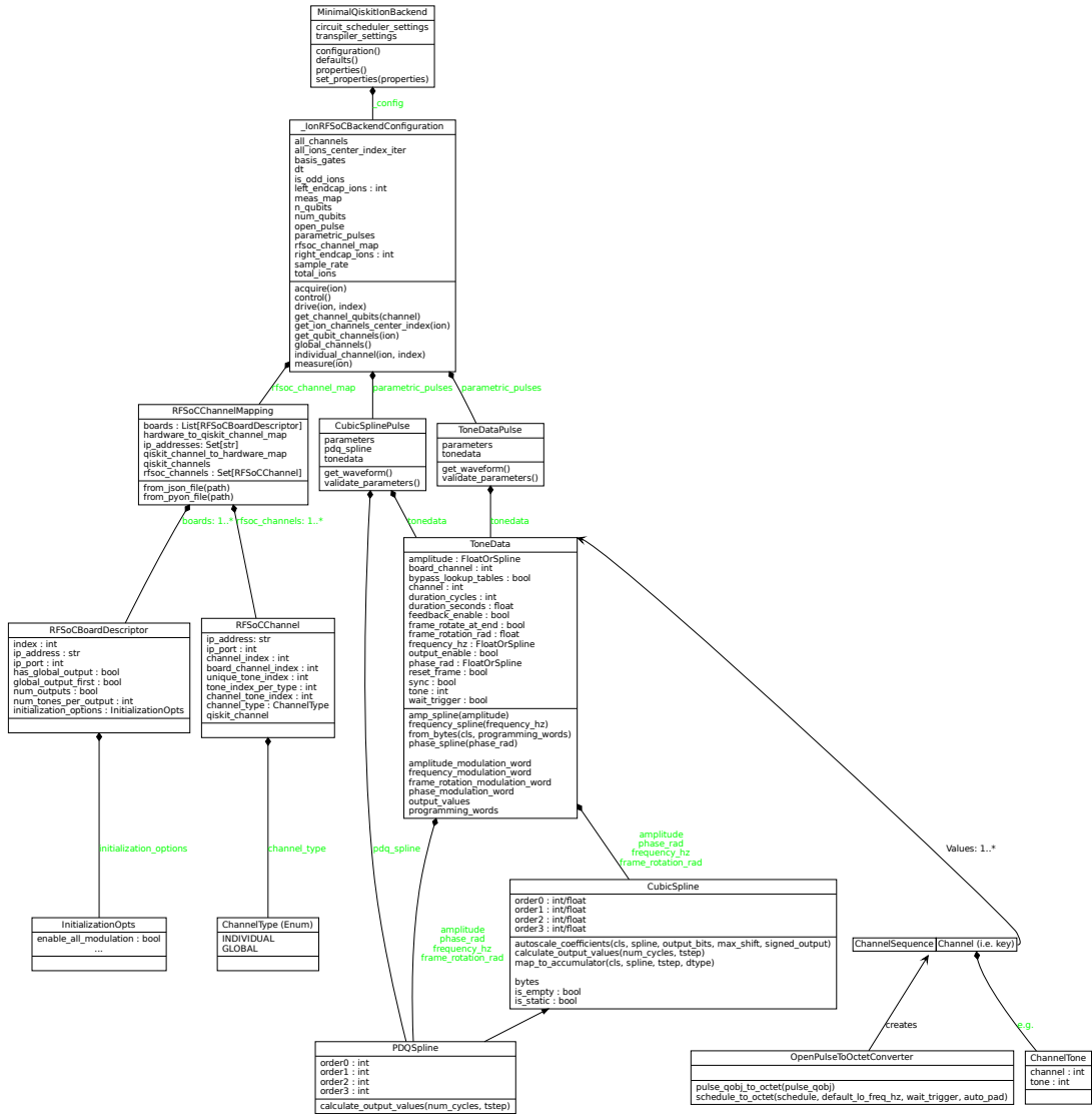
Figure 6.1: Primary pulsecompiler classes, as a UML class diagram. Higher-level classes are optional, and are only relevant if you are using qiskit for describing pulses. The base classes are at the bottom, and more abstract ones are towards the top. Green text w/ an arrow denotes a class attribute is an instance of the other class, most other arrows are inheritance.
