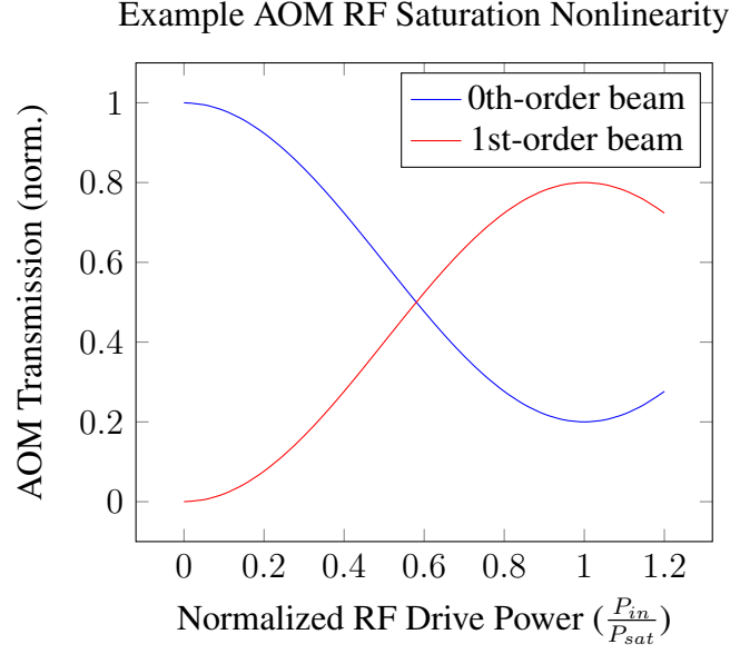
Figure A.1: Example of AOM Transmission Saturation as a function of RF Drive Power. The AOM transmission on the first-order beam (desired) saturates at P_{in} = P_{sat} . The x-axis is the normalized drive power (normalized so that 1.0 is the saturation point), and the y-axis is the amount of the total beam power diffracted into a given AOM beam order (normalized to total beam power). This AOM has diffraction efficiency of 80 %.
