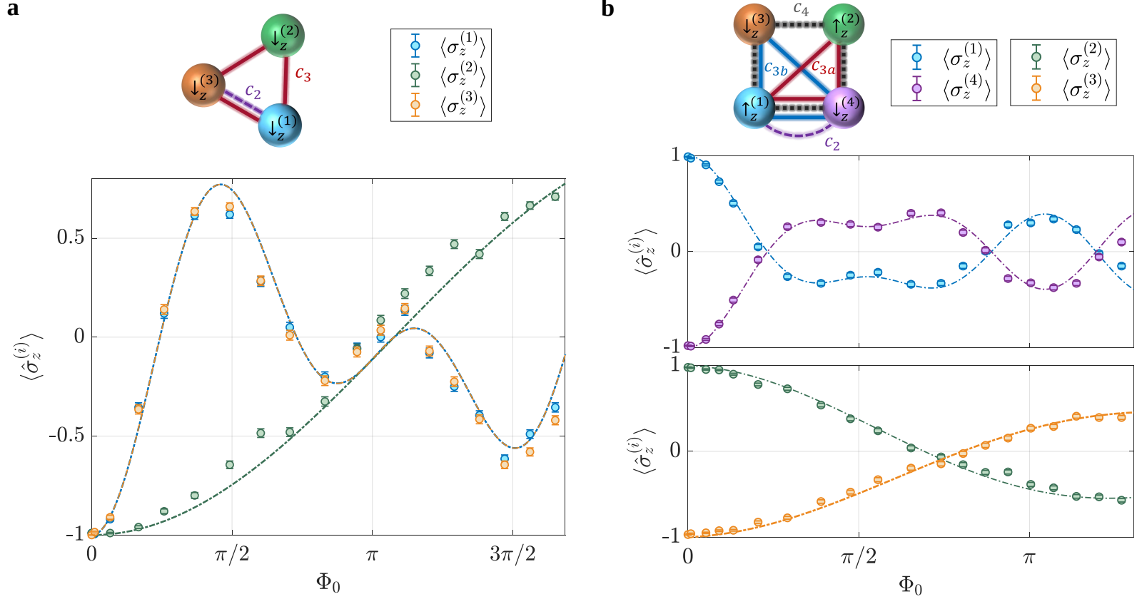
Figure 7.6: Effective Hamiltonians with three- and four-body interactions. a , Evolution of three spins by the effective Hamiltonian H_{\text{eff}} = \hbar\Phi/T for \Phi in Eq. (7.6) for the initial state |\downarrow_z^{(1)} \downarrow_z^{(2)} \downarrow_z^{(3)}\rangle . The effective Hamiltonian comprises two- and three-body terms whose magnitudes c_2 = 1.03 and c_3 = 0.23 as illustrated via the links connecting the different spins. The evolution as a function of \Phi_0 is realized with a fixed sequence time. b , Evolution of four spins by the effective Hamiltonian in Eq. (7.7) containing simultaneously two-, three- and four-body terms with amplitudes c_2 = 1.1 , c_{3a} = 0.36 , c_{3b} = 0.31 and c_4 = 0.1 . Dot-dashed lines are the analytically calculated magnetizations for the same initial state |\uparrow_z^{(1)} \uparrow_z^{(2)} \downarrow_z^{(3)} \downarrow_z^{(4)}\rangle where the c amplitudes are determined from the calculate squeezing parameters. Bars represent 1\sigma binomial uncertainties. The applied experimental sequences are presented in Fig. 7.5 (b-c).
