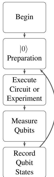
Figure 3.10: Diagram of a standard experiment cycle using trapped ion qubits. This diagram is only the part of the cycle that interfaces with the ions directly. Other preparation, calibration, and analysis steps will need to be performed external to the experiment runtime on the ions. Each loop iteration here is commonly referred to as a shot .
