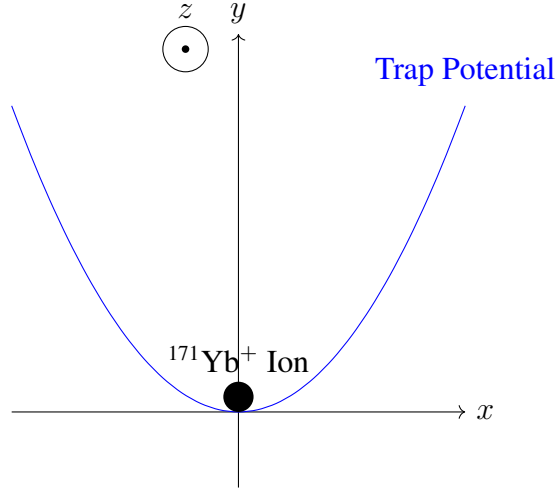
Figure 3.8: Axes of an ion in a harmonic trap. The x axis is the axis of the trap. Vibration along the y (vertical) and z (out of page) axes is called the radial (transverse) modes. A single ion trapped in this potential will have 3 motional modes, each with their own energy and number of phonons.
