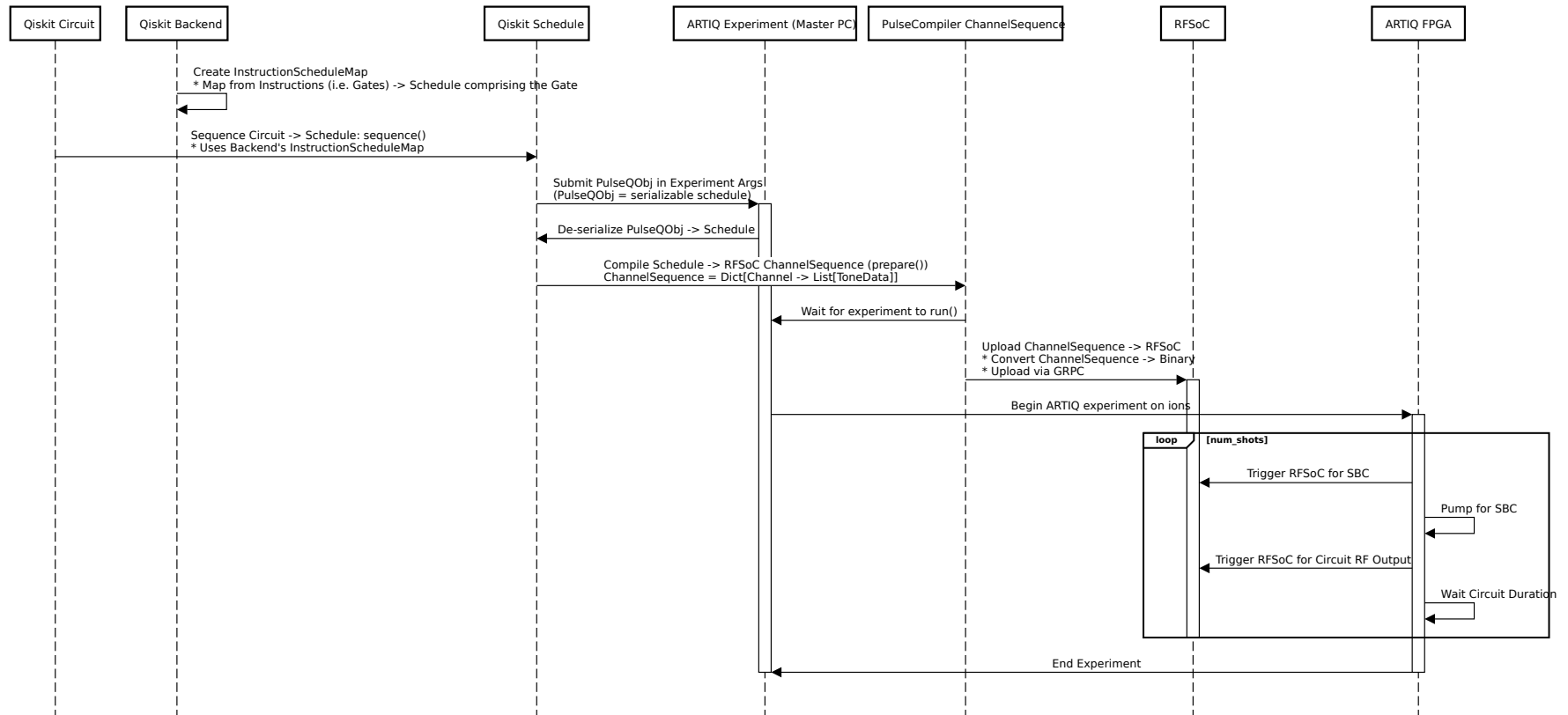
Figure 6.4: Diagram of the order of operations for converting a QuantumCircuit to run on an RFSoc. Once a QuantumCircuit is converted to run on an RFSoc, it can be triggered and executed as described in Chapter 5 .
