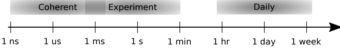
Figure 4.1: Diagram of the various experimental timescales and their corresponding control realm. The gap between experiment and daily is filled in our experiment via control software, which manages issues at this timescale via e.g. ensuring that the appropriate number of ions is present.
