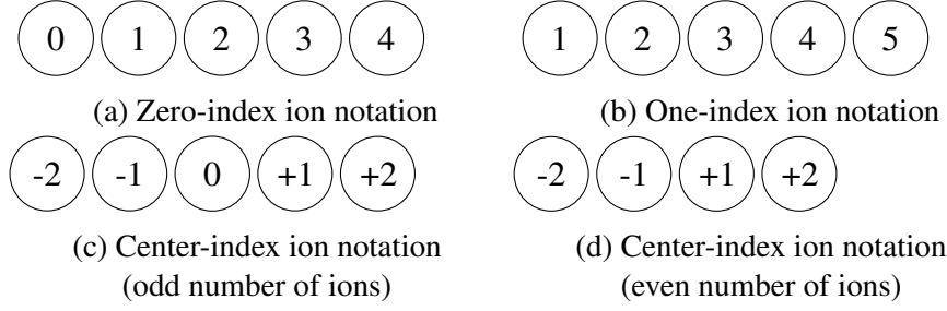
Figure 8.1: Ion Physical Qubit Indexing Options These indexing schemes are illustrated for ion chains of N_{ions} \in \{4, 5\} , though they can be extended to an arbitrary number of ions. For new systems under development, we recommend solely using center-index notation wherever possible, though the other indexing options might still be desirable in certain use cases. Some examples include when working with certain quantum circuit packages such as Qiskit, which does not support negative qubit indices natively.
