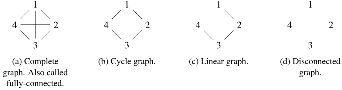
Figure 2.5: Example Qubit Connectivity Graphs for N_{qubits} = 4 . There are a limited amount of graphs that can be demonstrated with only 4 nodes, but this illustrates a few of the major classes.
