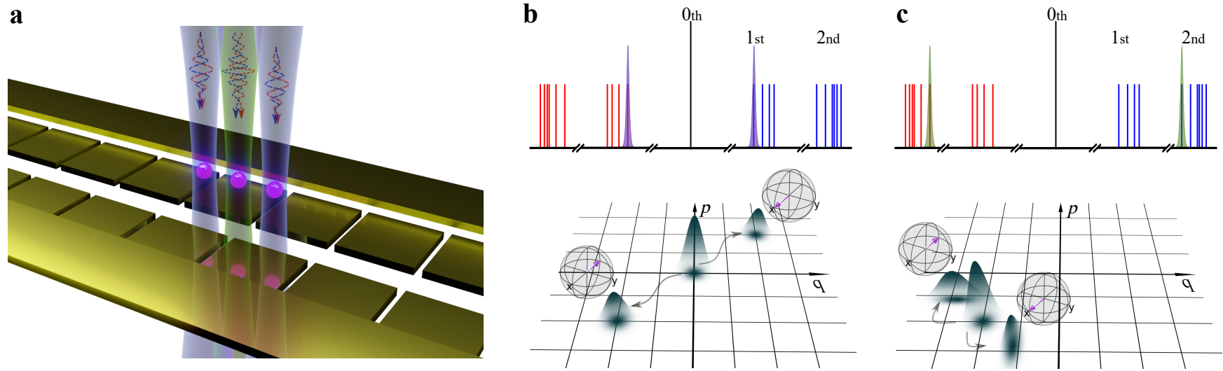
Figure 7.1: Native N-body operations of a trapped-ion quantum processor. a , Linear chain of laser-cooled ion spins in a chip trap. An array of optical beams addressing individual ions enable exquisite control over the state of each spin and its coupling to collective phonon-modes using Raman transitions (additional global beam forming the Raman pairs not shown). b , Spin-dependent displacement of one phonon-mode and its representation over the acoustic phase-space. Simultaneous driving of the first red and blue sideband transitions of one ion near resonance with one phonon mode displaces the phonon wavepacket (gray Gaussian) into two distinct trajectories, depending on the state of that spin along the X direction over its Bloch sphere (purple arrow). c , Spin-dependent squeezing of one phonon-mode. Simultaneous resonant driving of the second red and blue sideband transitions of one ion and one phonon mode squeezes (anti-squeezes) the phonon wavepacket along one direction of phase-space depending on the state of that spin along the x direction. Thin-lines in the 2D plots of (b-c) represent the sideband spectrum and narrow red and blue Gaussians represent the spectral content of the Raman coupling near the sidebands.
