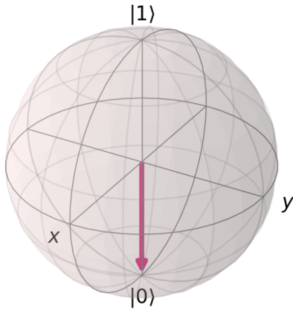
Figure 2.1: Bloch sphere representation of |0\rangle . In the Bloch sphere representation, any point on the surface of the sphere is a valid state. Some conventions will invert the Z ( |0\rangle , |1\rangle ) axis, but this thesis will not use that convention to align more closely with the ( |\downarrow\rangle , |\uparrow\rangle ) physics convention. The only difference between these two conventions is an inversion of the sphere across the x - y plane.
