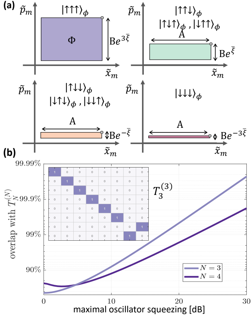
Figure 7.2: 3-body entangling gates (3-Toffoli) (a) Phase space evolution for three spins, following the sequence of alternating spin-independent displacements and spin-dependent squeezing operations. Each ion squeezes the momentum quadrature of the m th motional mode by a factor e^{-\xi} if its spin points downwards ( |0\rangle ), and anti-squeezes the momentum quadrature of the m th motional mode by a factor e^{+\xi} if its spin points upwards ( |1\rangle ). The state-dependent phase-space area \hat{\Phi}_{seq} accumulated in the evolution generates the gate U_{seq} = e^{-i\hat{\Phi}_{seq}} (Eq. (7.1)) with a maximal squeezing of the oscillator mode by a factor e^{N\xi} when all spins are aligned. The total area enclosed by the phase-space rectangle depends on the number of spins along the axis \phi_i : if 3 spins are along \phi_i then the largest rectangle is produced; if 2 spins are along \phi_i then the next-largest rectangle is produced; if 1 spin is along \phi_i then the second-smallest rectangle is produced; if no spins are along \phi_i then the smallest rectangle is produced.
