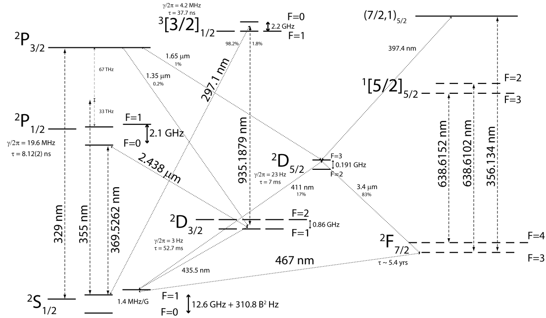
Figure 3.3: Diagram of the atomic energy levels of ^{171}\text{Yb}^+ ions. The horizontal lines in this diagram denote different energy levels of ^{171}\text{Yb}^+ . Within a given shell configuration (e.g. 2S_{1/2} ), there are different sub-levels that correspond to different electron- & nucleus-spin configurations. We chose to define our qubit states as sub-levels of the 2S_{1/2} manifold: |0\rangle \equiv |F=0, m_F=0\rangle , |1\rangle \equiv |F=1, m_F=0\rangle . To rotate between |0\rangle \leftrightarrow |1\rangle , we use a pulsed 355 nm laser to off-resonantly couple to the 2P_{3/2} & 2P_{3/2} levels, which can yield a transition between |0\rangle \leftrightarrow |1\rangle if the difference between two paths of this laser are equal to the frequency difference between the |F=0, m_F=0\rangle & |F=1, m_F=0\rangle states. This is called a stimulated two-photon Raman transition. Note that this frequency difference can change depending on e.g. the magnetic field. The dashed lines denote transition wavelengths between two energy levels. Dotted lines indicate spontaneous decay transitions from a higher-level energy state to a lower-level energy state. The \frac{\gamma}{2\pi} denotes the transition wavelength of this state, and \tau denotes the lifetime of that state. For quantum computation, the primary states in this diagram that concern us are 2S_{1/2} , & 2P_{1/2} . For state preparation, we also need to consider 2D_{3/2} , as discussed in Section 3.6.2.2 . Finally, note that this is a partial state diagram, and not every possible state of ^{171}\text{Yb}^+ is shown here. Image courtesy of George Toh.
