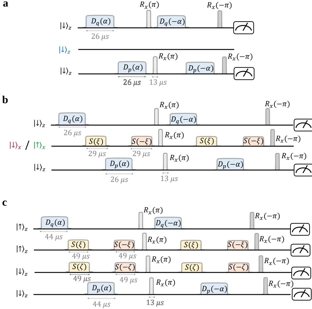
Figure 7.5: Experimental N-Body gate sequences. a , Sequence of displacement operations acting on the two edge ions and composing the MS interaction, enclosing a closed rectangular loop in phase-space and generating the evolution Fig. 7.3a. b , Superimposing spin-dependent squeezing operations on the second spin scales the displacement generated by the third spin by a factor \exp(\sigma_x^{(2)}\xi) and consequently also the enclosed phase-space area. This sequence was applied to the configurations in Fig. 7.3 (b-c) and in Fig. 7.4 and Fig. 7.6 (a). c , Displacement of the edge two spins and simultaneous squeezing of the middle spins for the four ions configuration presented in Fig. 7.6 (b). The simultaneous squeezing scales the displacement generated by the fourth spin by a spin-dependent factor \exp(\sigma_x^{(2)}\xi + \sigma_x^{(3)}\zeta) as seen from the identity S^{(m)}(-\xi)D_p^{(n)}(\pm\alpha)S^{(m)}(\xi) = D_p^{(n)}(\pm e^{\sigma_x^{(m)}\xi}\alpha) . The operators D_p^{(n)}(\pm\alpha) and D_q^{(n)}(\pm\alpha) denote displacement of the target phonon mode via the n th ion by \pm\alpha along the p and q coordinates respectively. S^{(m)}(\pm\xi) denotes the squeezing operator acting on ion m and R_\theta^{(n)}(\pm\pi) denotes short single-qubit \pi -pulses acting on the n th ion, which commute with the spin-dependent displacement operations and which correct for slowly-varying uncompensated Stark shifts without altering the target state.
