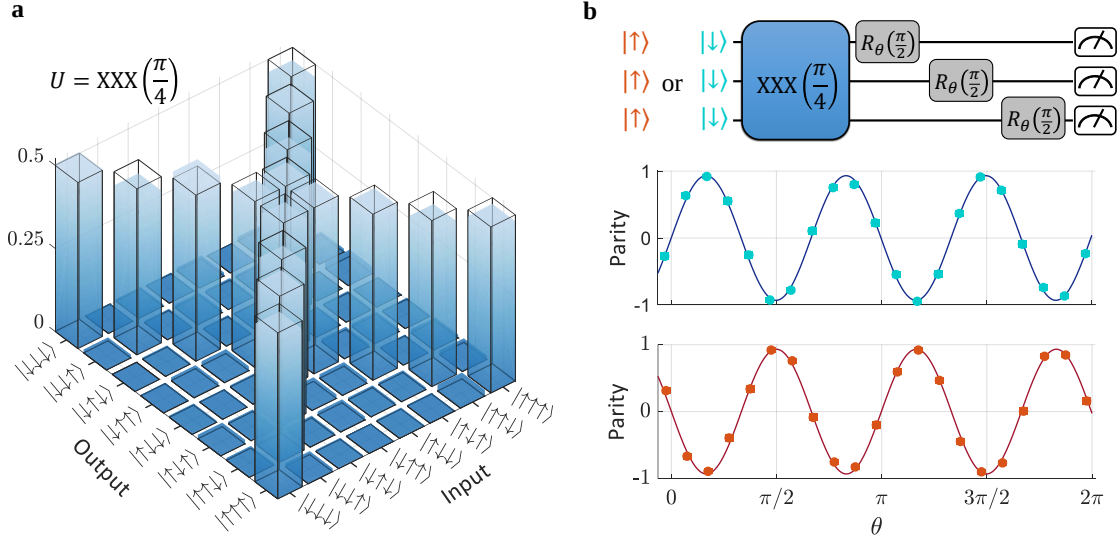
Figure 7.4: Characterization of a three-body interaction gate. a , Truth table of a three-body gate XXX(\frac{\pi}{4}) = \exp(-i\frac{\pi}{4}\sigma_x^{(1)}\sigma_x^{(2)}\sigma_x^{(3)}) gate generated by sequence of displacement and squeezing operations. The input and output spin states are along the z basis. Each input state is ideally mapped into a pair of output states (wire frames), and raw measurement are shown in solid bars. The measured populations of these target states is (95.8 \pm 0.9)\% , averaged over the 8 measured configurations. b , Parity measurement of the output GHZ state for the two initial states |\downarrow_z^{(1)}\downarrow_z^{(2)}\downarrow_z^{(3)}\rangle (light blue) and |\uparrow_z^{(1)}\uparrow_z^{(2)}\uparrow_z^{(3)}\rangle (red) with a fitted amplitude of 0.932 \pm 0.015 for the two states. The extracted GHZ fidelities for this operation for the two states are \mathcal{F} = (94.8 \pm 1.5)\% and \mathcal{F} = (94.4 \pm 1.9)\% . Bars represent 1\sigma binomial uncertainties and dashed lines are sine functions. The operation R_\theta(\pi/2) denotes single qubit rotation by azimuthal angle \theta and a polar angle \pi/2 on the Bloch sphere.
