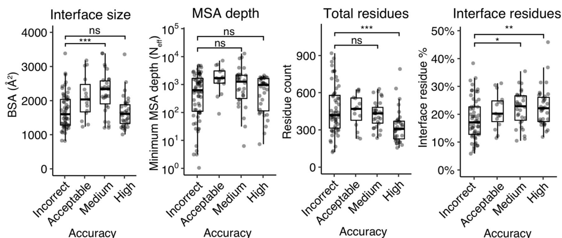
FIGURE 3 Assessing test case features associated with AlphaFold success. Protein complex and MSA feature values were computed for all cases, which are shown according to AlphaFold success (best AlphaFold model accuracy in the five models for that case). Features shown are interface buried surface area (BSA), MSA depth ( N_{eff} ) for the ligand or receptor (minimum value of the two), total number of residues, and percent of total residues in the protein–protein interface. Statistical significance values (Wilcoxon rank-sum test) were calculated between feature values for sets of cases with incorrect versus medium and incorrect versus high- CAPRI accuracy, as noted at top (ns: p > .05 , * p \leq .05 , ** p \leq .01 , *** p \leq .001 )
