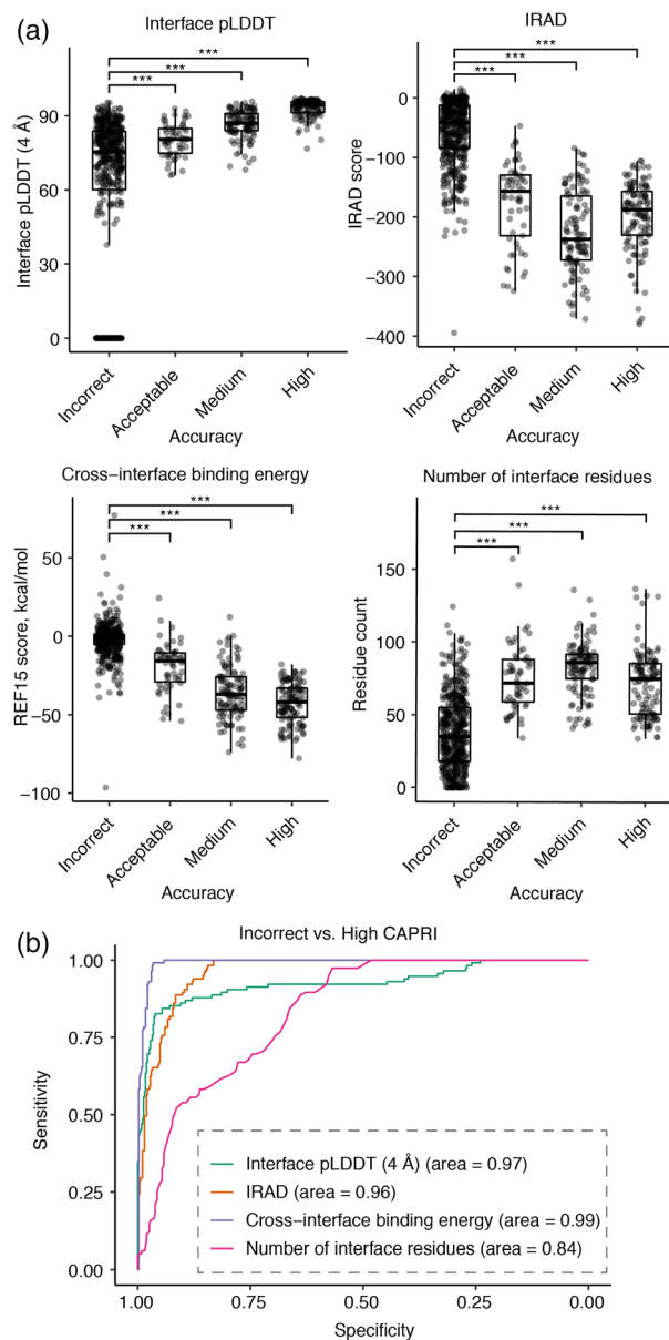
FIGURE 6 Association between alternative scoring metrics and docking model quality. (a) Distributions of interface pLDDT (4 Å), IRAD, Rosetta cross-interface binding energy, and number of interface residues for AlphaFold models grouped by CAPRI criteria. An interface pLDDT score of 0 was assigned to models without any interface contacts within the distance cutoff (4 Å). Constrained local minimization was performed using Rosetta FastRelax 65 to resolve unfavorable local geometries or clashes in models, and post-relaxation models were scored with IRAD and the Rosetta 45 InterfaceAnalyzer protocol, with the latter used to calculate cross-interface binding energy scores (based on the Rosetta REF15 energy function 66 ) and the number of interface residues. Statistical significance values (Wilcoxon rank-sum test) between scores of incorrect versus acceptable, incorrect versus medium, incorrect versus high CAPRI criteria are indicated at the top of each plot ( ***p \leq .001 ). Each point corresponds to one AlphaFold model, and all five AlphaFold models for 149 test cases are represented. (b) ROC curves among the scoring metrics for classifying incorrect versus high accuracy models by CAPRI criteria, with corresponding AUC values denoted in parentheses
