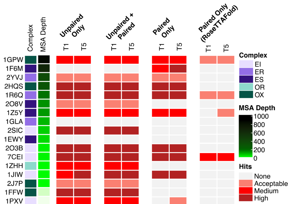
FIGURE 4 The impact of MSA pairing on prediction accuracy. MSAs were generated using MMseqs2 using the “advanced” interface of ColabFold. 29 Pairing was performed in ColabFold on a total of 17 cases whose ligand and receptor proteins come from the same prokaryotic organism. Cases in the heatmap were sorted by the paired MSA depth ( N_{\text{eff}} ; see Material and Methods for details) from the largest to the smallest values. Structural predictions were generated with the “advanced” interface of ColabFold, and RoseTTAFold 28 (through the Robetta server). All models were assessed for near-native predictions within the top-ranked (T1) and top 5 (T5) models using CAPRI criteria. Complex category: Enzyme-inhibitor (EI), enzyme complex with a regulatory or accessory chain (ER), enzyme-substrate (ES), others, receptor-containing (OR); others, miscellaneous (OX)
