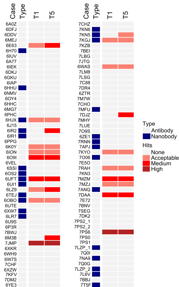
FIGURE 8 AlphaFold-Multimer modeling success for an expanded set of recently released antibody–antigen complex structures. A benchmark set of 100 recently released antibody–antigen complex structures was modeled with AlphaFold-Multimer, and all five models from AlphaFold-Multimer per test case were assessed for accuracy using CAPRI criteria. AlphaFold-Multimer was run in ColabFold with MSA input and with the use of structural templates released before April 30, 2018, and models were ranked by pTM score. Success for top 1 and top 5 (T1, T5) ranked predictions is shown, colored by CAPRI model accuracy as indicated in the key on right (Hits). “Type” distinguishes complexes containing heavy-light chain antibodies (“Antibody”) and single-chain nanobodies (“Nanobody”).
