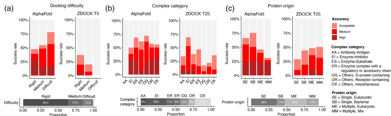
FIGURE 2 Determinants of successful performance. (a) Prediction success of AlphaFold and ZDOCK, grouped by docking difficulty. Based on binding conformational changes as defined by BM5.5, 20,23 cases are categorized into “rigid,” “medium,” and “difficult” docking difficulty levels. To evaluate the success rate, all five models from AlphaFold and top five ZDOCK models were considered. (b) Prediction success of AlphaFold and ZDOCK grouped by complex category. To evaluate the success rate, all five models from AlphaFold and top 25 ZDOCK models were considered. The number of ZDOCK models was increased to 25 to allow for sufficient success rates to show its relative performance among the categories. (c) Prediction success of AlphaFold and ZDOCK grouped by protein source organism(s). To evaluate the success rate, all five models from AlphaFold and top 25 ZDOCK models were considered. Based on the source of subunit proteins in the complex structures, each case is classified as either “single, eukaryotic” (SE, denoting proteins from the same eukaryotic organism), “single, bacterial” (SB, denoting proteins from the same bacterial organism), “multiple, eukaryotic” (ME, denoting proteins from different eukaryotic organisms), or “multiple, mix” (MM, denoting proteins from mixed origins). Two additional protein source classes, corresponding to proteins from different bacterial organisms, and proteins of viral origin, were omitted from the success plot due to limited representation in each category (four and two cases in those classes, respectively). Bars are colored by model accuracy as indicated in (a). The horizontal stacked bars below each success rate plot denote the composition of the categories by class
