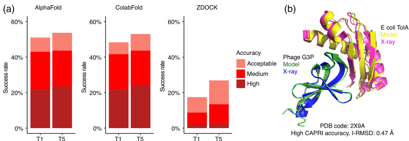
FIGURE 1 Transient protein–protein complex structure prediction success by AlphaFold, ColabFold and ZDOCK. End-to-end modeling using AlphaFold 24 and ColabFold 29 was performed on 152 complex test cases (details in Figure S1). AlphaFold failed to generate predictions for three complexes, thus AlphaFold predictions were obtained for 149 complexes; these 149 test cases were used to calculate success rates in this figure. Docking models were also generated with ZDOCK, 33 using unbound protein structures as input. All sets of models were assessed for near-native predictions using CAPRI criteria for high, medium, and acceptable accuracy. (a) Complex prediction success of AlphaFold, ColabFold, and ZDOCK for the top 1 (T1) and top 5 (T5) models considered. AlphaFold and ColabFold models were ranked by AlphaFold pTM scores, and ZDOCK models were ranked by IRAD scores. 39 The percent success was calculated as the percentage of test cases with a given model accuracy from the top N models considered. Bars are colored according to the CAPRI quality classes. (b) Example of an accurately predicted complex structure (PDB code: 2X9A) by AlphaFold. This model has high accuracy by CAPRI criteria (I-RMSD = 0.47) and has the highest pTM score (pTM = 0.77) of all five models generated for this complex. Structures are superposed by Phage G3P, with the model and the X-ray structure chains are colored separately as indicated. For clarity, regions modeled by AlphaFold but unresolved in the X-ray structure are not shown in the figure
