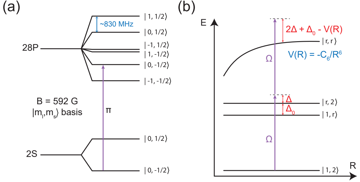
Figure E.1: Rydberg dressing of ^6\text{Li} . (a) Level diagram showing the hyperfine ground states of ^6\text{Li} directly coupled to the 28P Rydberg state using linearly ( \pi ) polarized light at a field of 592 G. The basis used is |m_l, m_s\rangle . (b) Rydberg dressing scheme for two atoms in different hyperfine ground states |1\rangle and |2\rangle coupled to the Rydberg state |r\rangle . \Omega is the Rabi coupling of the laser, \Delta is the detuning from the resonant transition between |1\rangle and |r\rangle , \Delta_0 is the hyperfine splitting between |1\rangle and |2\rangle and V(R) = -C_6/R^6 is the van der Waals interaction potential between two Rydberg states |r\rangle .
