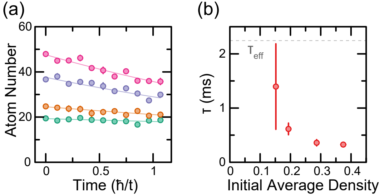
Figure E.3: Atom loss during charge density wave dynamics. (a) Atom number decay over the quenches shown in Fig. 6.5. Each color represents a set with a different initial density. Circles are measured data with error bars and lines are simple exponential decay fits. The dressing parameters were \Omega = 2\pi \times 6.99(8) MHz and \Delta = 2\pi \times 30 MHz. (b) Lifetime vs. the initial average density of the charge density wave as extracted from the data in (a). This behavior is in agreement with our observations shown in Fig. 6.3. Experimental error bars correspond to standard error of the mean.
