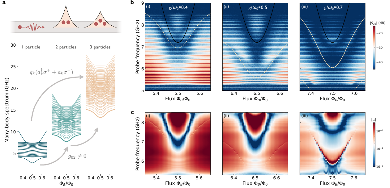
Figure 4.3: Many-body scattering dynamics of a single propagating photon. a. If the artificial atom is restricted to a two-level system and the RWA approximation is valid, the multi-particle eigenstates of the joint system form isolated bands of fixed-excitation manifolds. In the full model, these particle sectors are coupled through counter-rotating terms and parity-breaking transitions to higher fluxonium states, as highlighted by arrows. The multiphoton bound states scatter a single propagating photon as they enter the single-particle band, see upper diagram where the photons are represented as red dots. b. This nonperturbative effect is captured in the measured transmission amplitude of a weak probe tone for increasing values of the SQUID coupler inductance which leads to an increased light-matter coupling (normalized coupling strength at the flux sweet spot is listed at the top of each plot). In addition to the main fluxonium transition resonance (solid black curve), we observe the two-photon and three-photon bound states entering the passband. The yellow theory curves are the calculated energy levels from diagonalizing the full model Hamiltonian. The dashed yellow curve corresponds to the calculated two-photon state, while the solid yellow curve (above the measured three-photon resonance) corresponds to the calculated three-photon state. c. The appearance of these additional multiparticle resonances are validated with MPS scattering simulations of the transmission amplitude t_k . The faint resonance that gets shifted down in frequency as we increase the coupling strength qualitatively follows the calculated energy for the two-photon bound state, while the strong Fano-like resonance in (iii) matches the calculated energy for the three-photon bound state.
