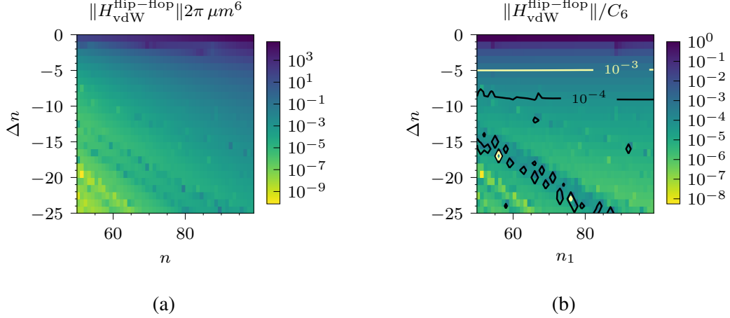
Figure F.1: Flip-flop vdW interactions for n_1S + n_2S as a function of n_1 and \Delta n = n_2 - n_1 . (a) Norm of the off-diagonal vdW block. (b) Ratio of the off-diagonal vdW interactions to the diagonal identity interactions.
