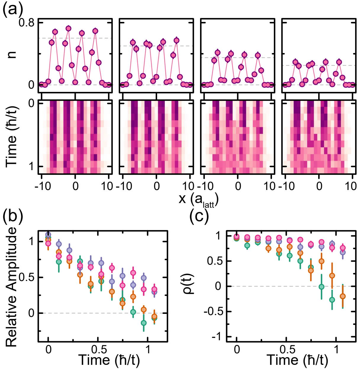
Figure 6.5: Density dependence of quench dynamics. (a) (top) Initial state density profiles. (bottom) Corresponding time evolution of each initial state for V/t = 2.9(2) . Colorbar is same as Fig. 6.4a with limits set by dotted lines on top panel. (b) Fitted relative amplitude of density profiles vs. time. Colors (green, orange, purple, and pink) correspond to the initial states in (a) from low to high density. (c) Autocorrelation function of the density pattern. Colors are same as in (b). Experimental error bars correspond to standard error of the mean.
