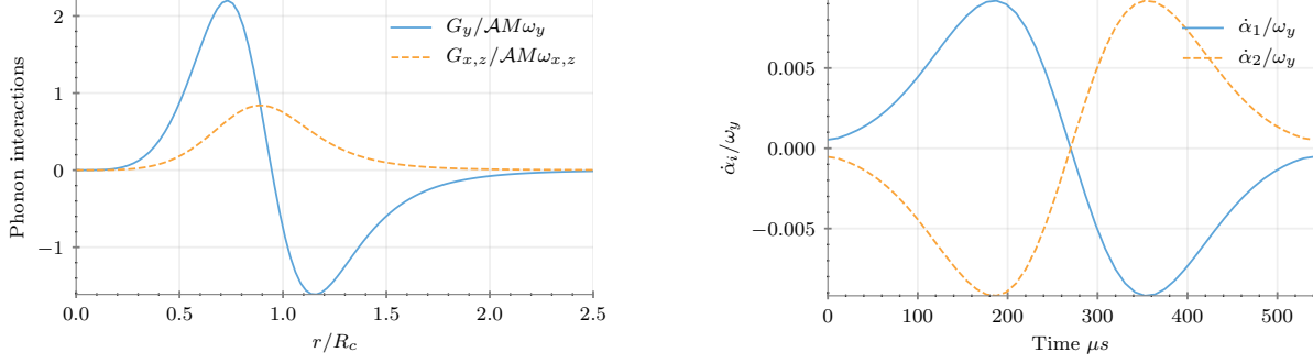
Figure F.2: (a) Normalized phonon interactions as a function of distance. (b) Non-adiabatic corrections normalized to the trap frequency \omega_y/2\pi = 50 kHz as a function of time for a Gaussian pulse with \mathcal{A}_{max}/2\pi = 34.4 MHz \mu m^6 , \sigma = 6.7 \mu s , t_0 = 215.9 \mu s for a trap separation of r_0 = 1.93 \mu m .
