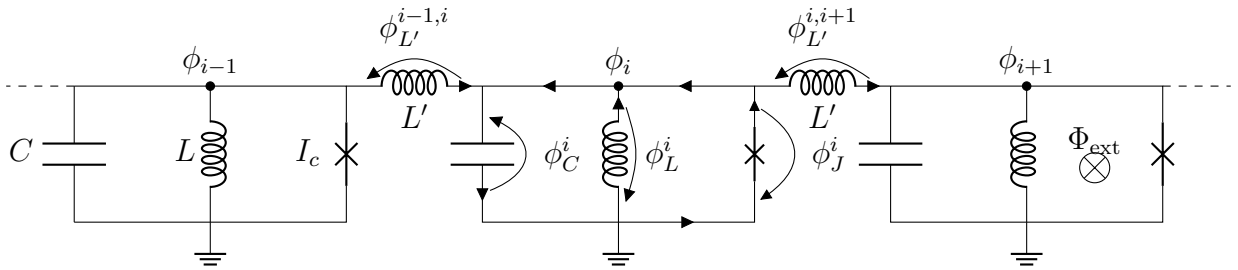
Figure A.2: Circuit diagram implementing the massive Thirring-Schwinger model. An external flux \Phi_{\text{ext}} threads each L-J loop.
