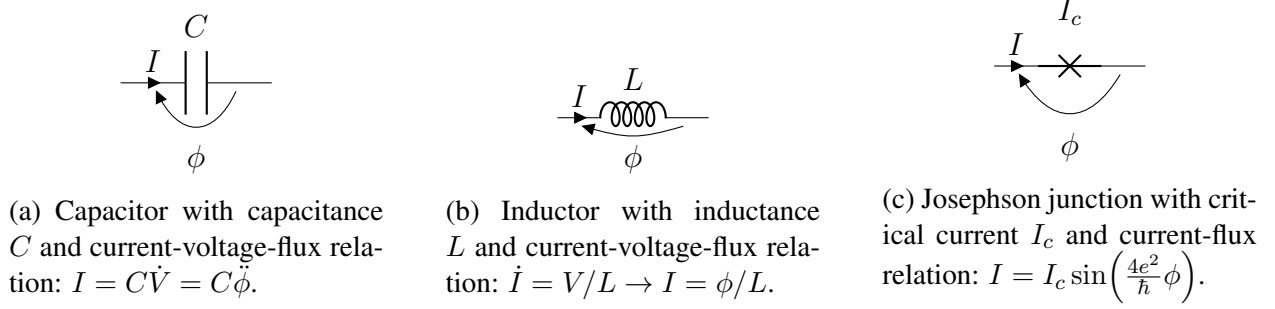
Figure 1.1: Building blocks of circuit QED.
