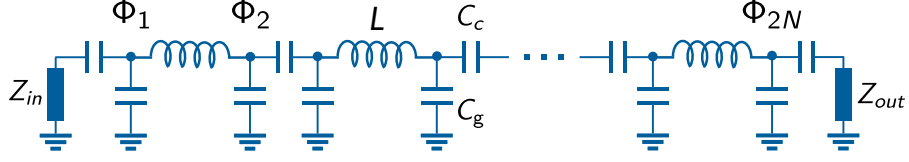
Figure C.2: Circuit diagram for a discretized photonic crystal. Schematic diagram of a one-dimensional chain of capacitively coupled microwave resonators.
