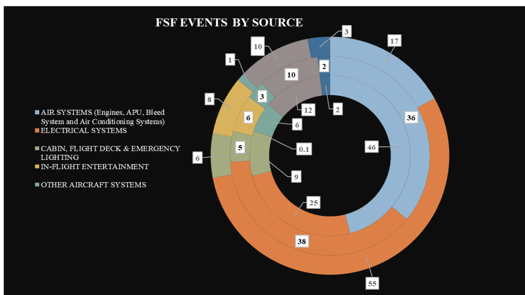
Figure 1.1 FSF Events by the source from Cherry (2017) across various passenger planes, Wide Body Passenger Airplanes (Outer Circle), Narrow Body Passenger Airplanes (Middle Circle) & Regional Passenger Airplanes (Inner Circle)
