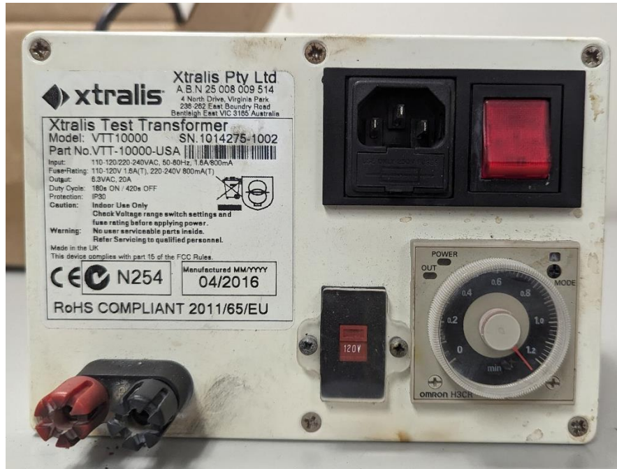
Figure 6.2 Xtralis Test Transformer used for cable failure tests
