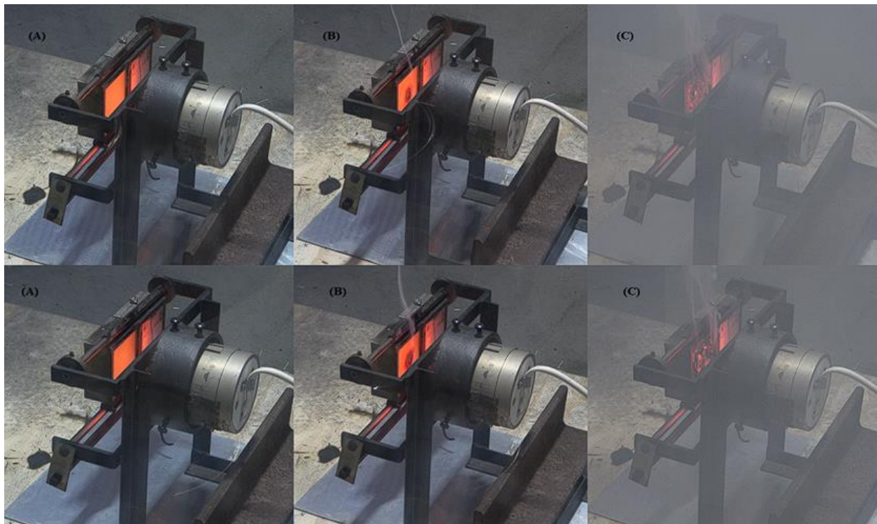
Figure 4.9 (TOP) FR-6 at (A) Time of placement of the sample (B) 3 minutes into the testing (B) 6 minutes into the testing
