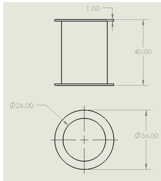
Fig. 46. Iteration 1 of the wire coil holder (dimensions in mm)
