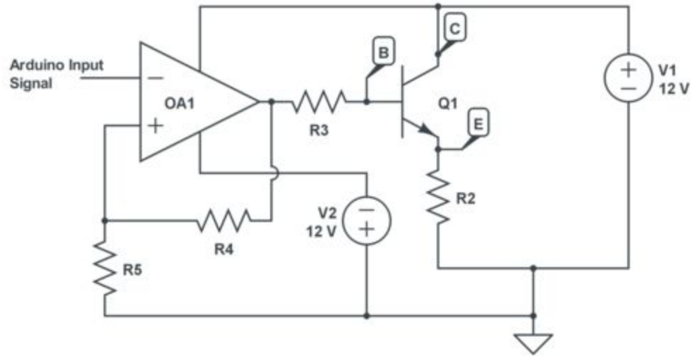
Fig. 38. Second iteration of circuit for magnetic actuation
