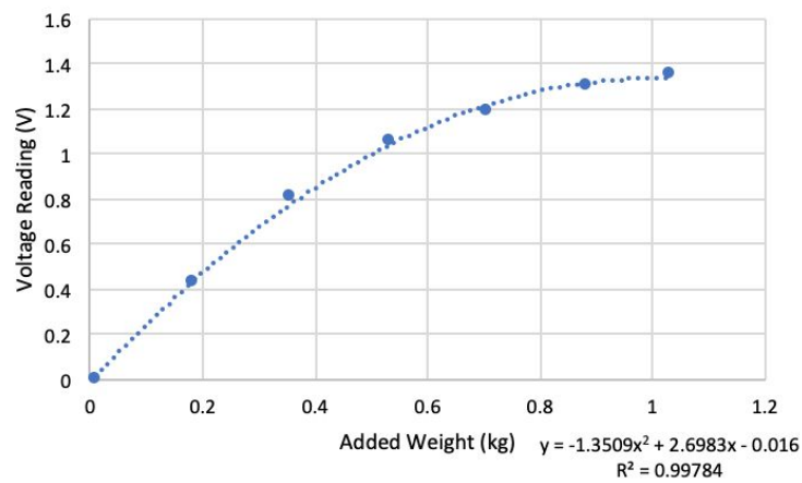
Fig. 25. Obtained sensor characteristic curve with the experimental methods described above, one measurement taken for each weight
