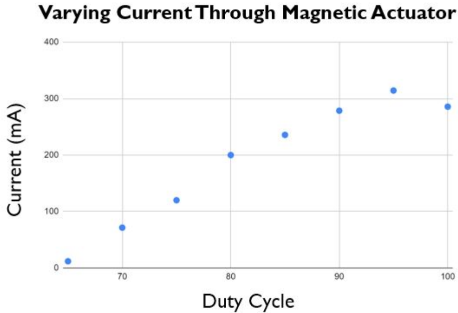
Fig. 43. Current through magnetic actuator for various duty cycle inputs
