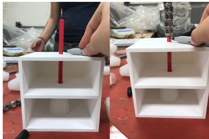
Fig. 22. Box and probe system in action
