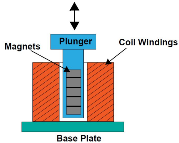
Fig. 8. Image of a basic linear solenoid
