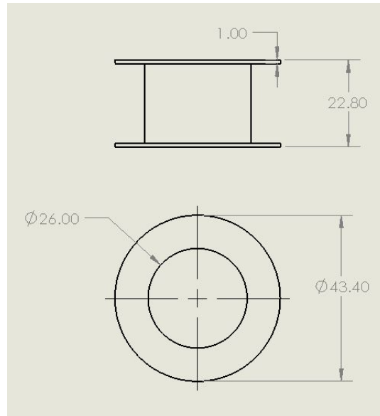
Fig. 47. Iteration 2 of the wire coil holder (dimensions in mm)
