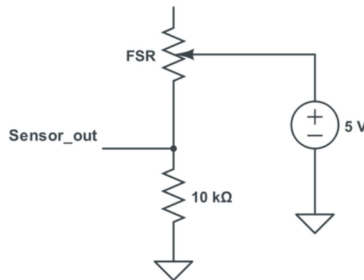
Fig. 24. Sensor circuit diagram as prescribed by sensor instruction
