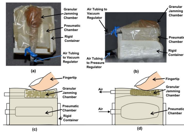
Fig. 7. Particle jamming system [7] © IOP Publishing. Reproduced with permission. All rights reserved
