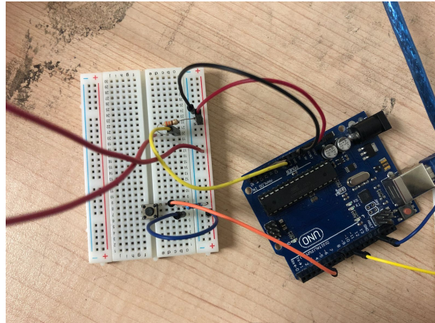
Fig. 32. Circuit and Arduino Uno for reading of data from the sensor, with the addition of a button for data acquisition
