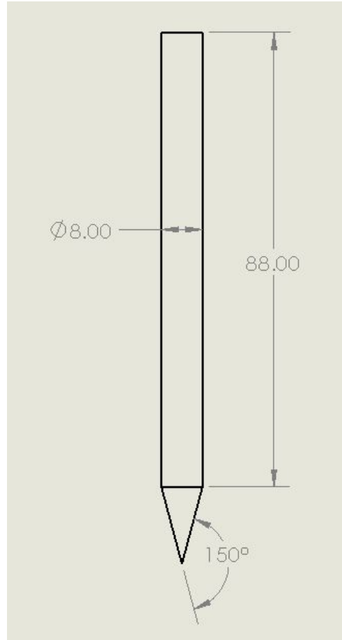
Fig. 21. Technical drawing of probe
