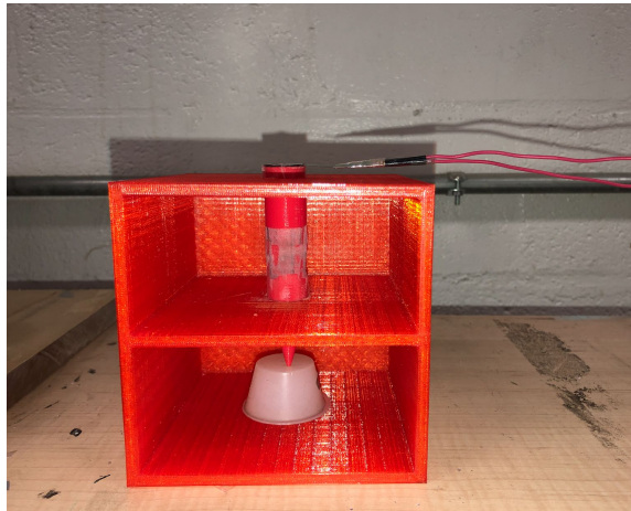
Fig. 27. Design of sensor to silicone testing box, prior to any added force for displacement
