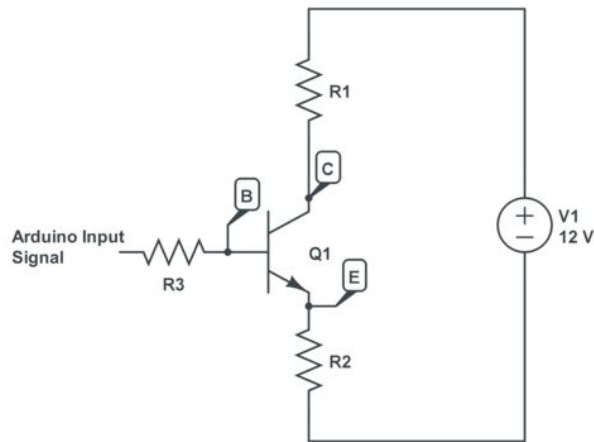
Fig. 36. First iteration of circuit for magnetic actuation.
