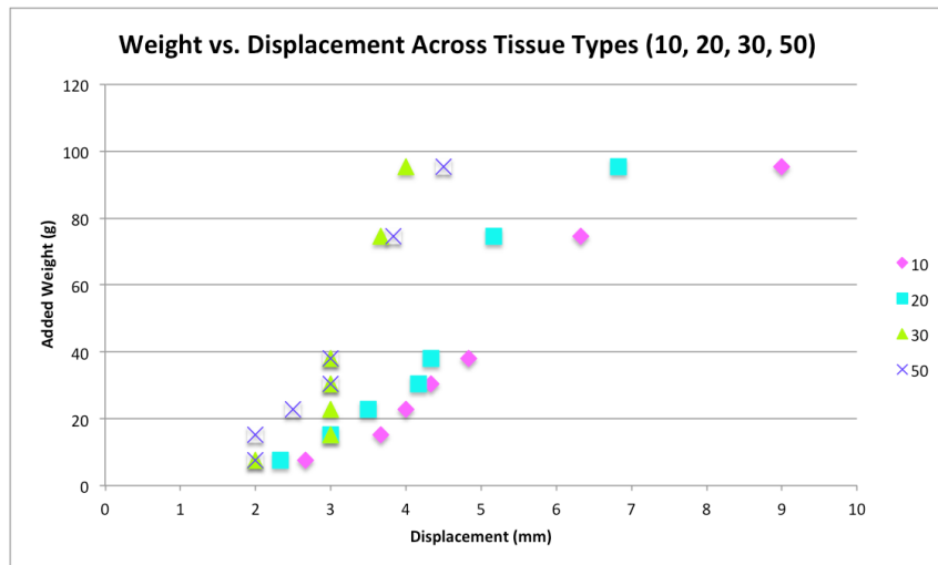
Fig. 20. Added weight versus displacement over silicone types 10, 20, 30, and 50
