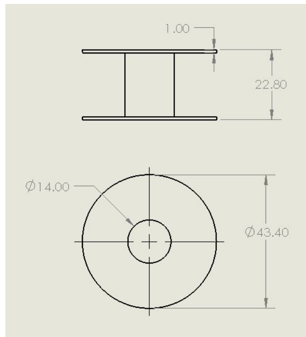
Fig. 48. Iteration 3, the final design, of the wire coil holder (dimensions in mm)
