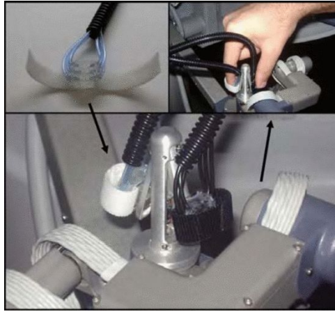
Fig. 5. Balloon-based pneumatic actuator [34] © 2008 IEEE
