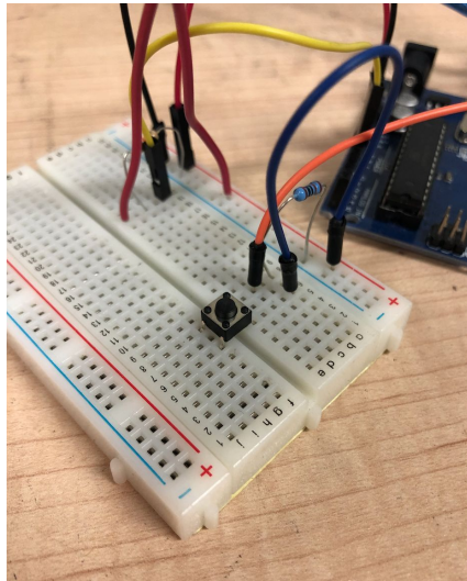
Fig. 33. The simple button addition to the sensor circuit, seen as the small black and silver square on the circuit board
