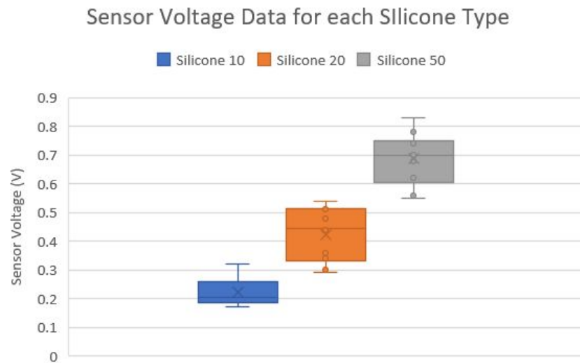
Fig. 29. Voltage values obtained from each silicone type ( n=10 )
