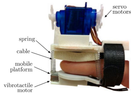
Fig. 6. Moving platform mechanism [4] © 2015 IEEE
