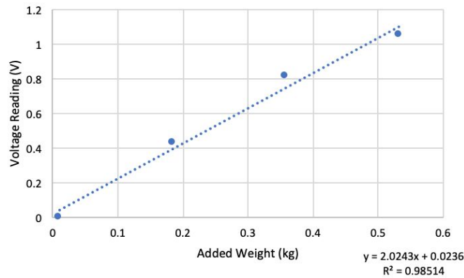
Fig. 26. Narrowed sensor characteristic curve to linear region with the experimental methods described above, one measurement for each weight
