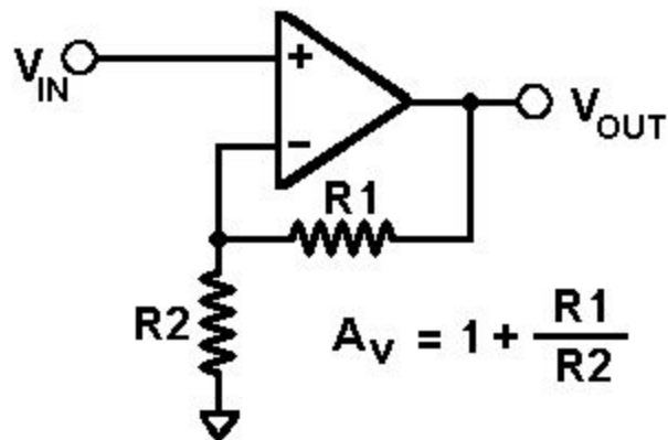
Fig. 39. Non-inverting amplifier using operational amplifier
