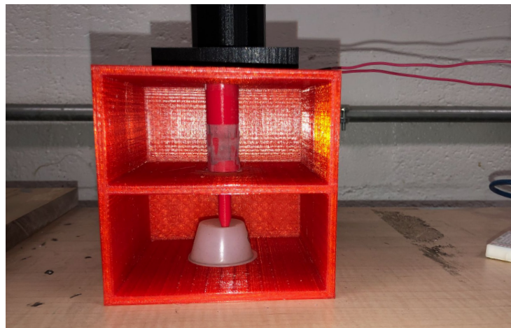
Fig. 28. Design of sensor to silicone testing box, after force has been applied to cause deformation in the silicone
