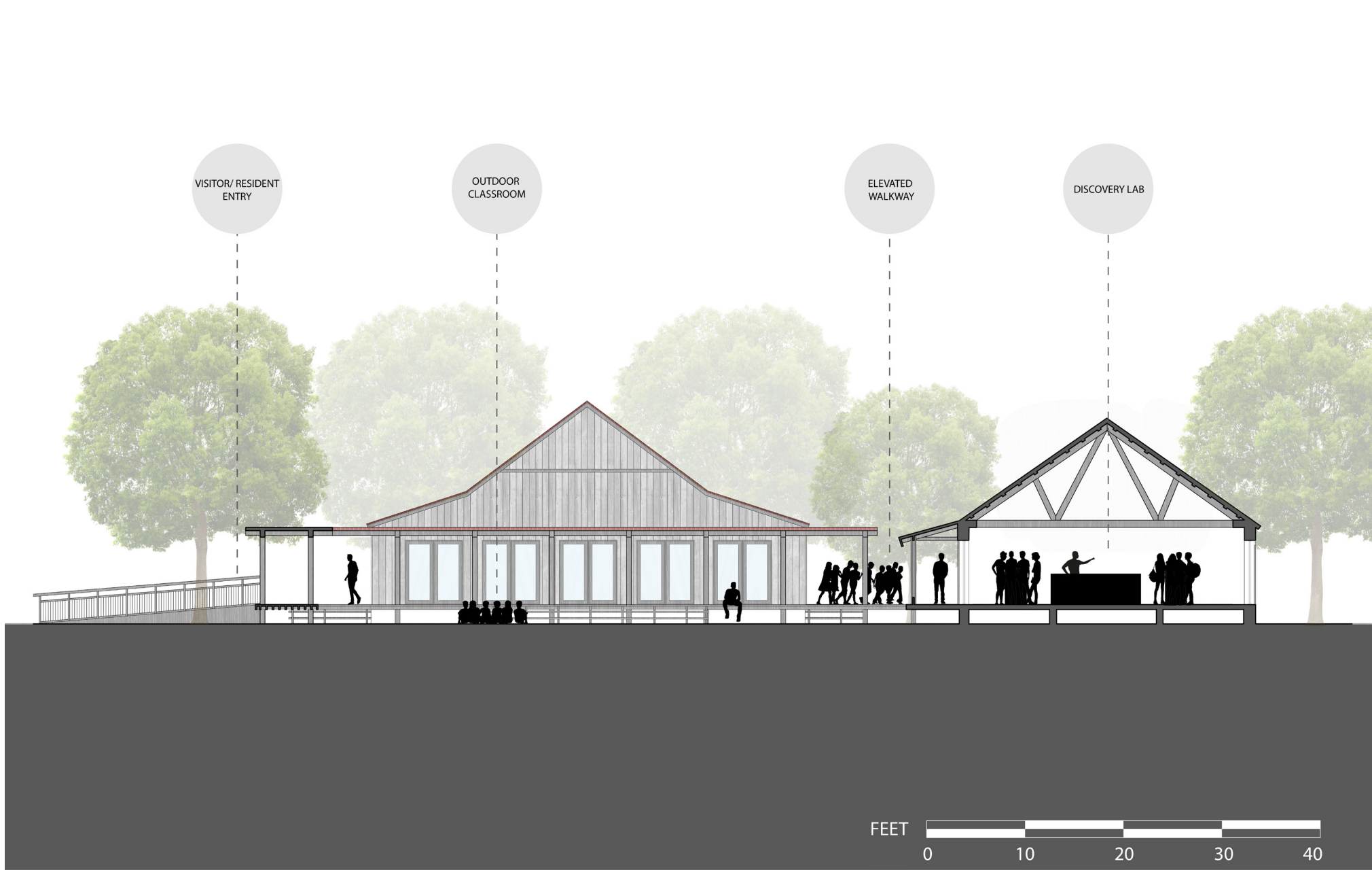
SECTION THROUGH DISCOVERY LAB
