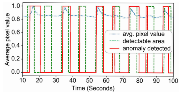
Figure 6: Detecting anomalous file write operations using the machine-learning-based technique.
