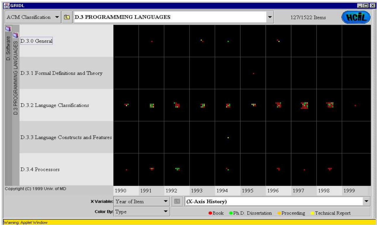
Figure4d:GRIDLwiththeACMComputingClassificationSystemaftertwocategoryexpansionsontheaxis, D.SoftwareandD.3ProgrammingLanguages
