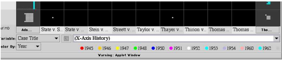
Figure5c:ManagingOvercrowdedAxes:Paging
