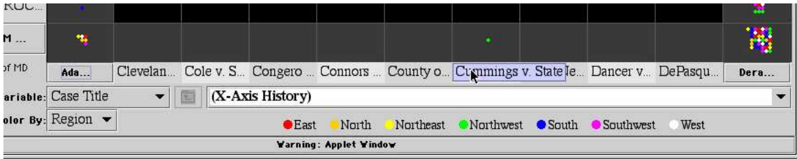
Figure5a:ManagingOvercrowdedAxes:ToolTips
