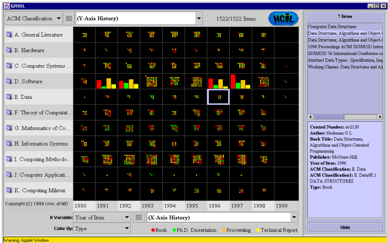
Figure4c:GRIDLwiththeACMComputingClassificationSystem,afteruserclicksonacluster
