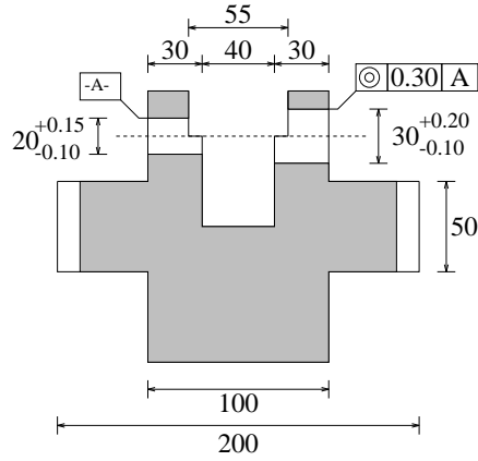
Figure 2: Design for the socket P_0 .
