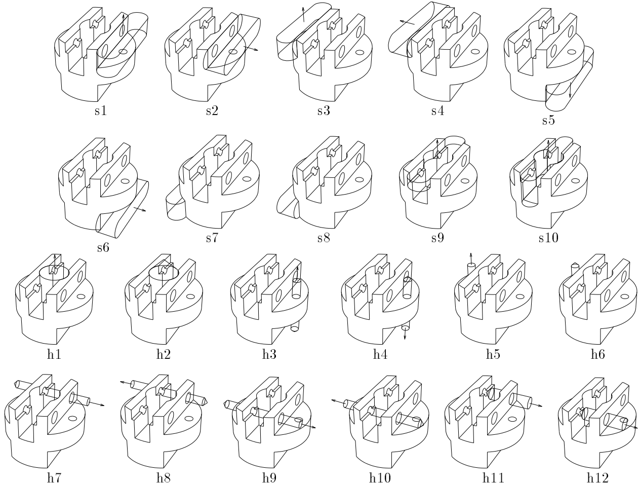
Figure 5: The set \mathcal{F} of all primary features for the socket P_0 . s_1, \dots, s_{10} are end-milling features; h_1, \dots, h_{12} are drilling features.
