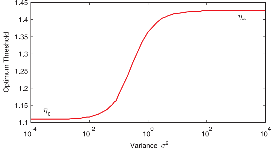
FIGURE 3. Optimum threshold as a function of the initial variance \sigma^2 , with a = 1 .
