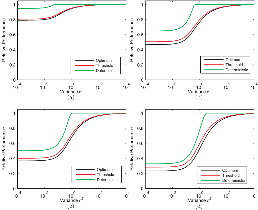
FIGURE 5. Relative performance of Optimum, Threshold and Deterministic samplers as a function of initial variance \sigma^2 and parameter values (a) a = 10 , (b) a = 1 , (c) a = 0 and (d) a = -1 .
