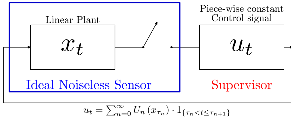
FIGURE 1. Sample and hold control
