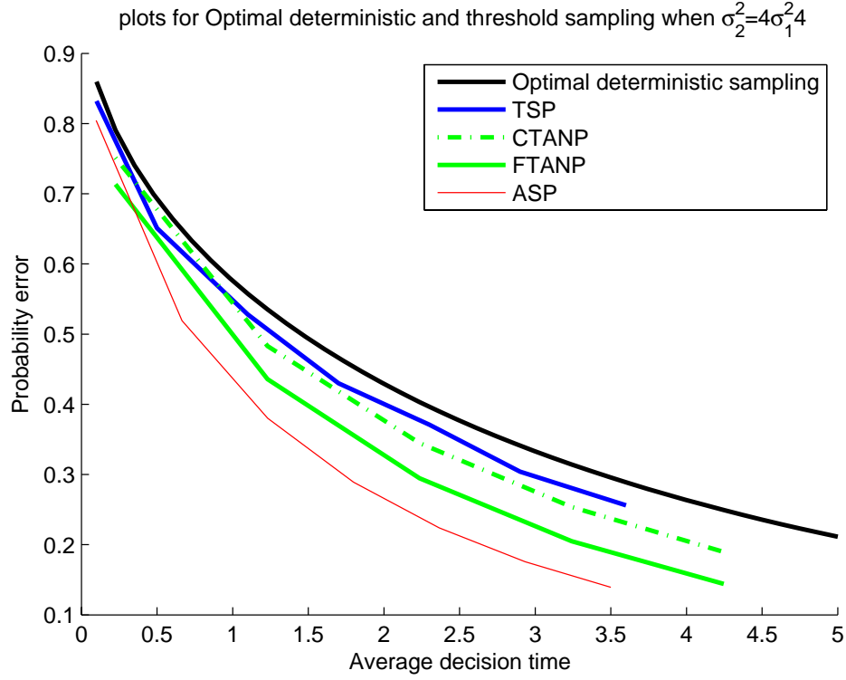
FIGURE 2. Plots of Probability of error vs. expected time taken to decide when the priors are equal. The asynchronous scheme performs well but the other threshold schemes are not clearly distinguishable.
