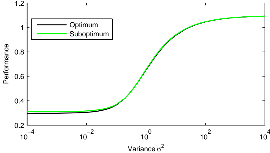
FIGURE 2. Relative performance of optimum (variable) threshold and suboptimum constant threshold sampling scheme, as a function of the variance ( \sigma^2 ) of the initial condition.
