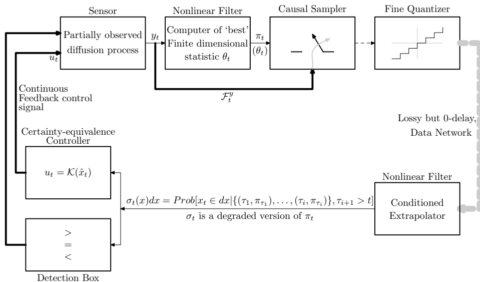
FIGURE 1. Schematic of a general Networked Control and Monitoring system with a single sensor.
