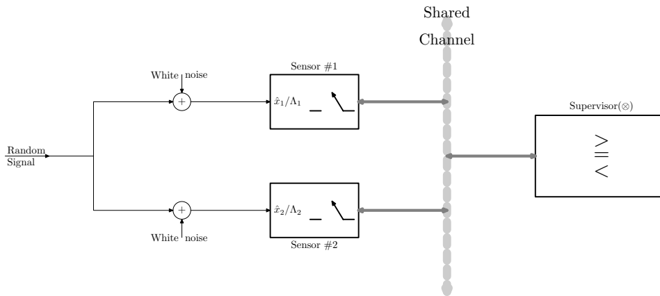
FIGURE 1. The two-sensor sequential detection set-up.
