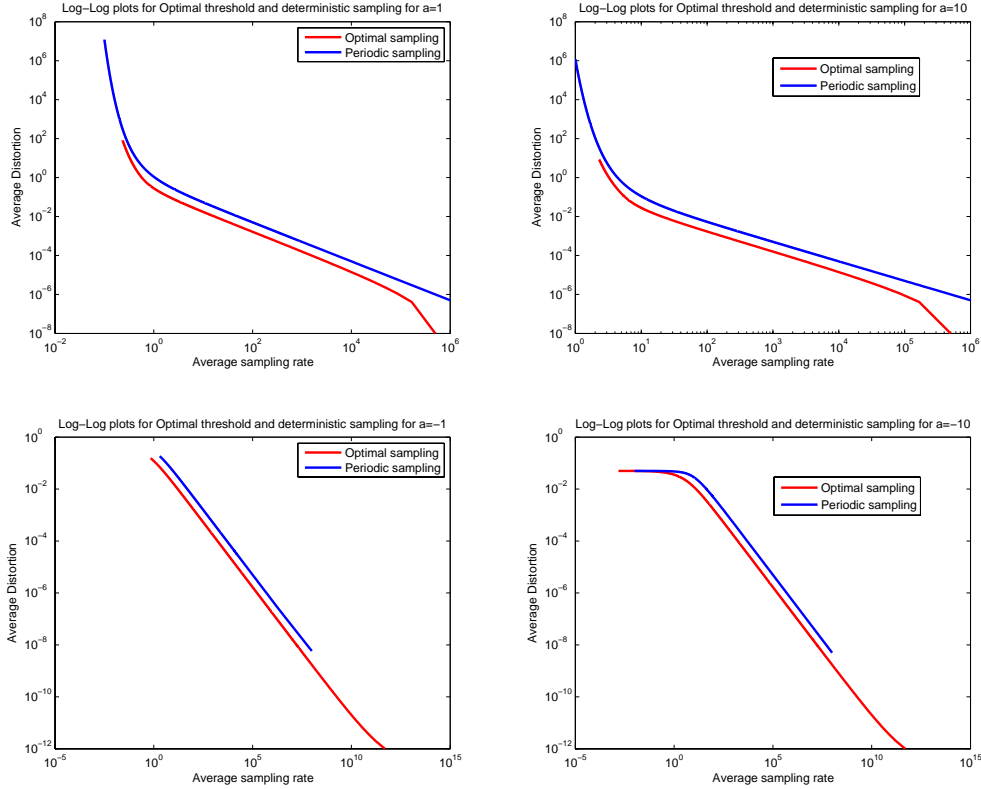
FIGURE 1. Relative performance of Optimal (Threshold) and Periodic samplers as a function of average sampling rate R_{av} and parameter values (a) a = 1 , (b) a = 10 , (c) a = -1 and (d) a = -10 .
