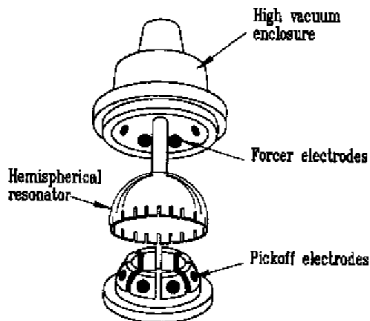
FIG. 1.2. Delco Hemispherical Resonator Gyroscope (Image from [14])
