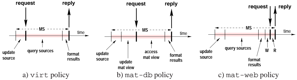
Figure 4: Staleness measurement
