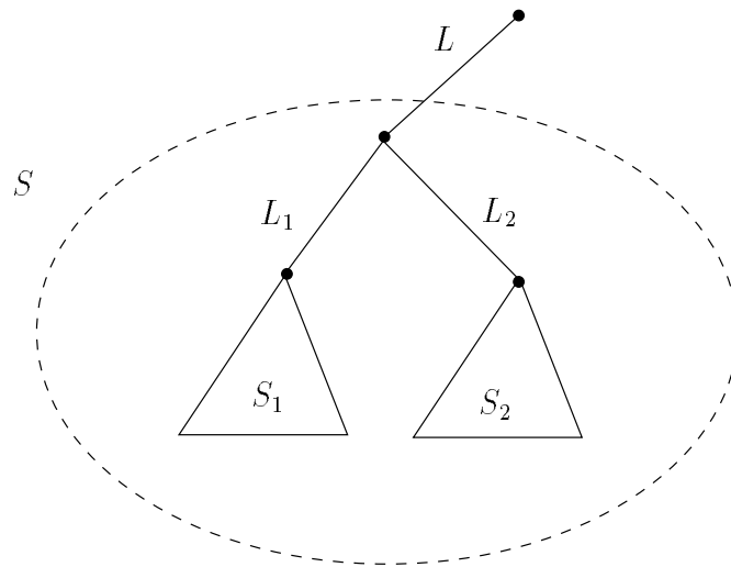
Figure 3: Inductive proof.
