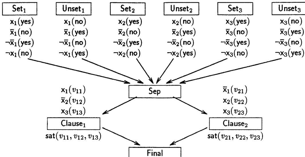
Figure 1: The plan P_X^* in the case where X = x_1\bar{x}_2x_3 + \bar{x}_1x_2x_3 . Each step's name is in a box, with its preconditions and postconditions above and below the box.
