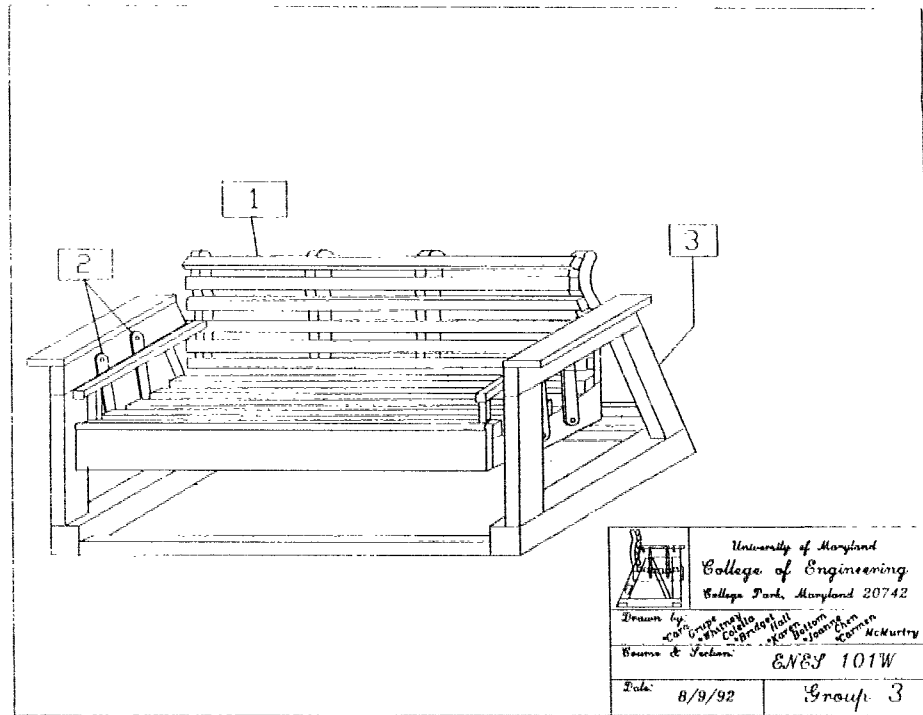
(a) Assembly Drawing of a Designed Porch Glider
