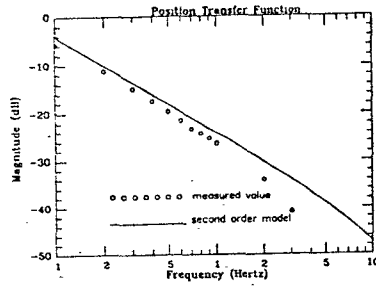
Figure 1: Theoretical vs. Actual Position Transfer Function
