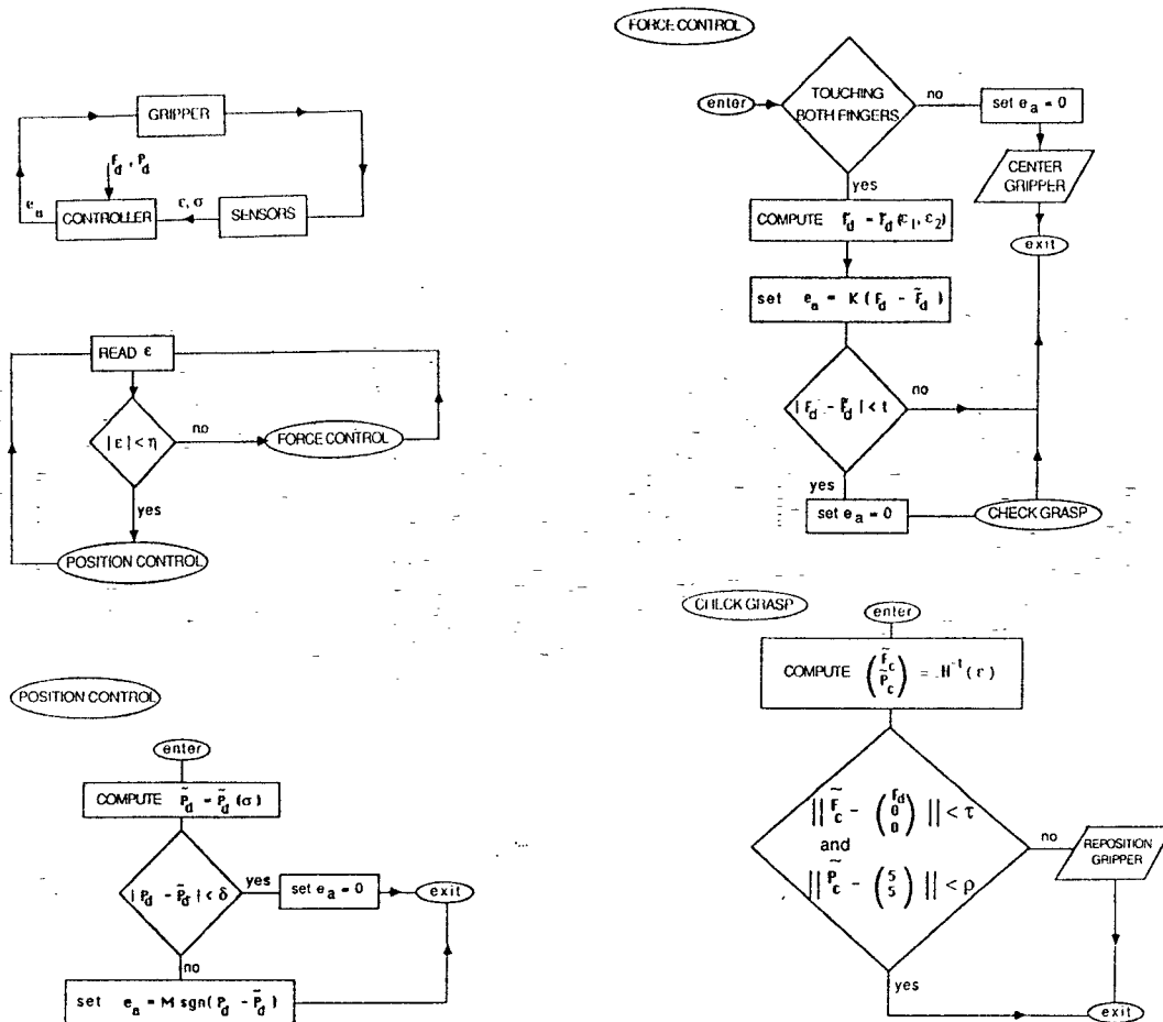
Figure 7: Control System Block Diagram
