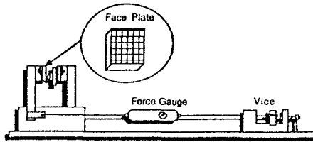
Figure 4: Experimental Setup for Accurate Force Measurements
