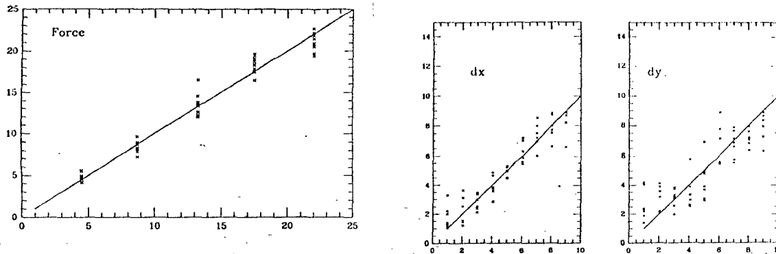
Figure 5: Actual vs Calculated Values for Holding Force and Position Offset
