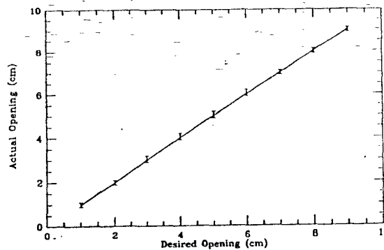
Figure 6: Positioning Accuracy
