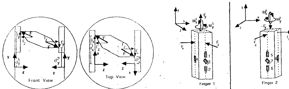
Figure 3: A. Contact Force Vectors B. Force and Moment Diagram
