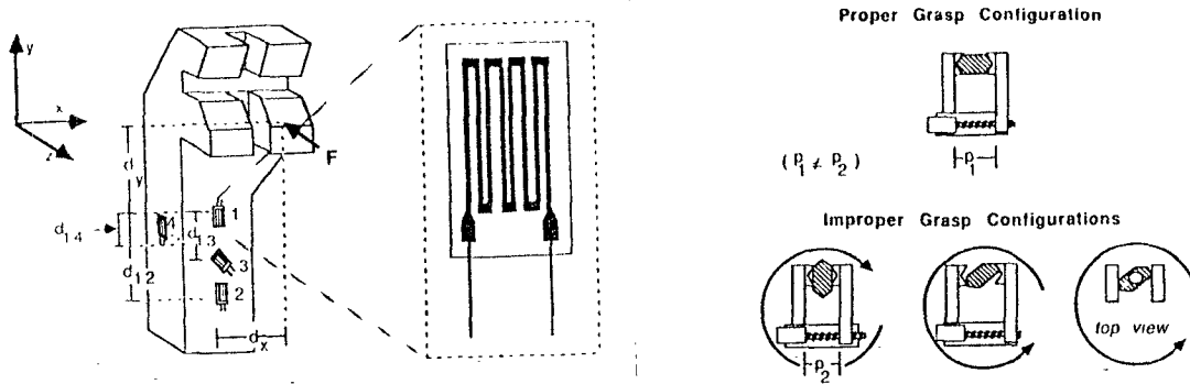
Figure 2: A. Strain Gauge Positions B. Grasp Configurations
