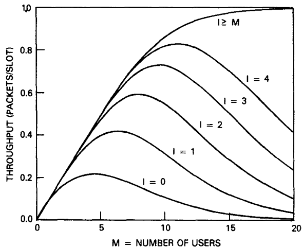
Fig. 7 Throughput performance of distributed reservation scheme for several levels of tolerable interference.
