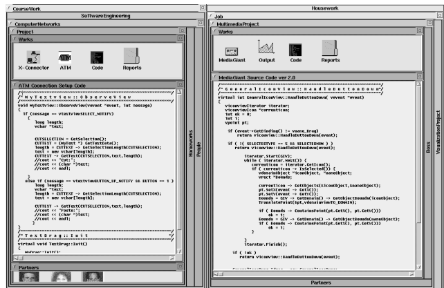
Figure 10: Layout customized to reference the code for Networks project at school, while working on the code for the Multimedia project at work.
