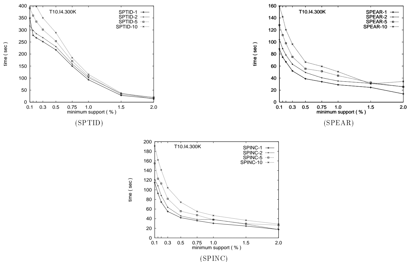
Figure 4.14: Times for different numbers of partitions
