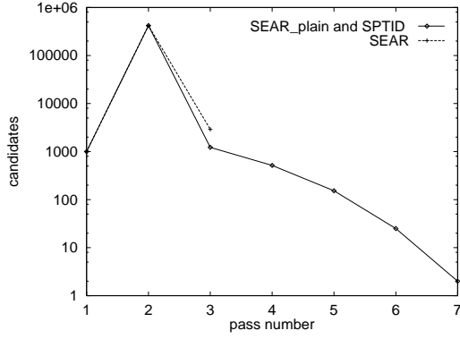
Figure 4.6: Candidates per pass s_{min} = 0.1\%
