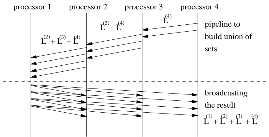
Figure 5.5: Union of sets of sets across processors
