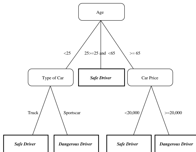
Figure 7.2: Example of Decision Trees Used in Classification
