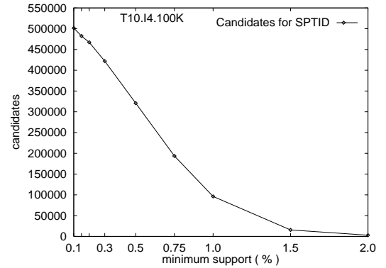
Figure 4.5: SPTID: Candidates depending on minimum support
