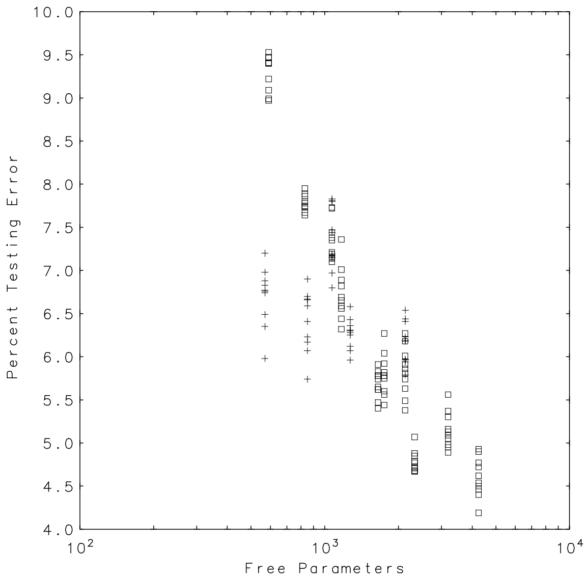
Figure 12: Testing error versus number of free parameters for MLP networks (+) and for RBF networks ( \square ).
