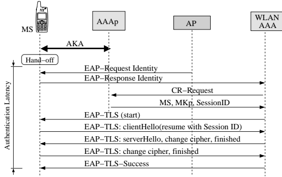
Fig. 9. Reactive Context Transfer To WLAN(EAP-TLS)
