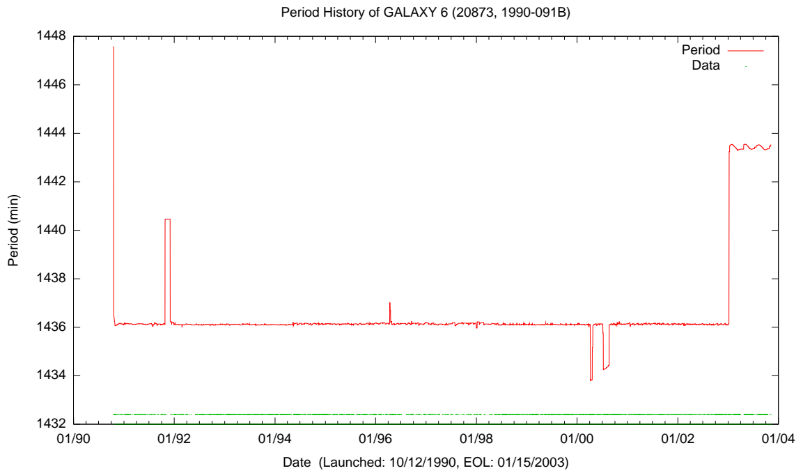
Figure E.5: Sample Satellite Period History Plot
