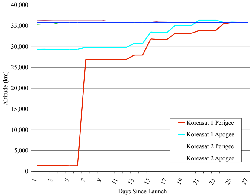
Figure D.5: KoreaSat 1 Altitude History
