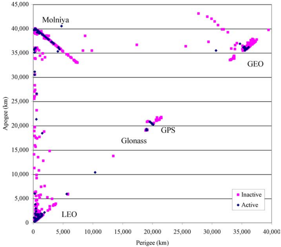
Figure A.13: Orbital Location Of All Spacecraft Near Earth
