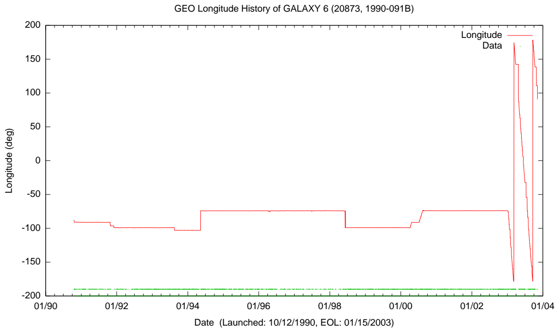
Figure E.3: Sample Satellite Geosynchronous Longitude History Plot
