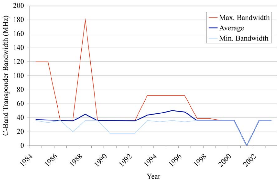
Figure 6.4: C-band Transponder Bandwidth By Year, 1994 To 2003
