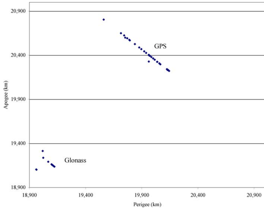
Figure A.15: Orbital Location Of Active Spacecraft In MEO
