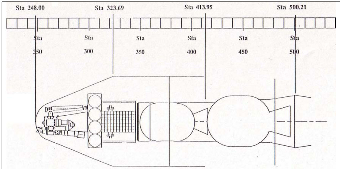
Ranger TFX On Delta II [77]
