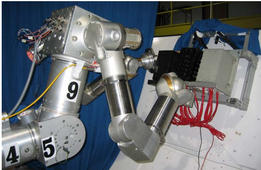
Figure 2.2: On-Orbit Servicing Robot Ground Demonstration, 2004 (RTSX) [34]
