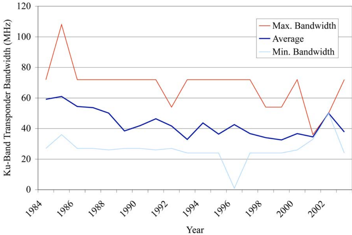
Figure 6.5: Ku-band Transponder Bandwidth By Year, 1994 To 2003
