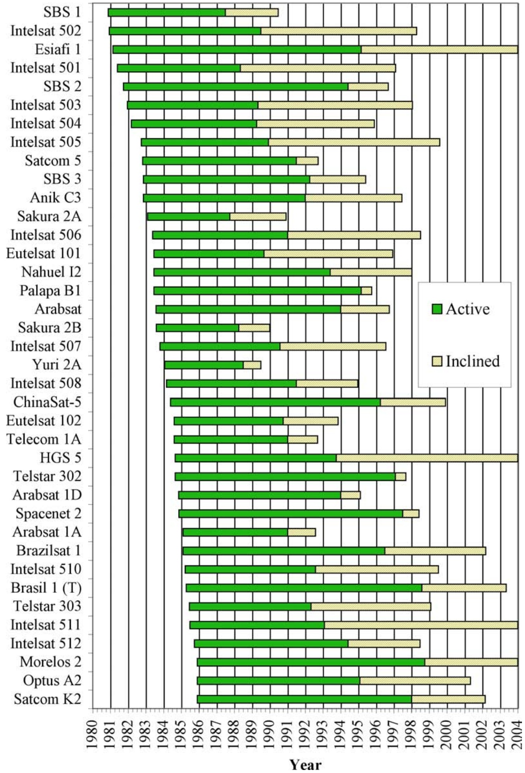
Figure A.18: Lifetimes Of Inclined Commercial Communications Satellites Launched Between 1980 And 1985
