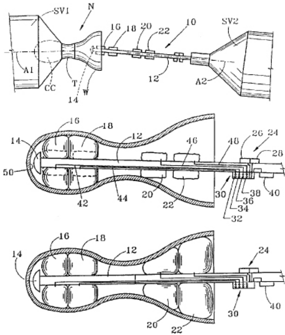
Figure 2.7: Apparatus for Attaching Two Spacecraft Under Remote Control [86], [87]
