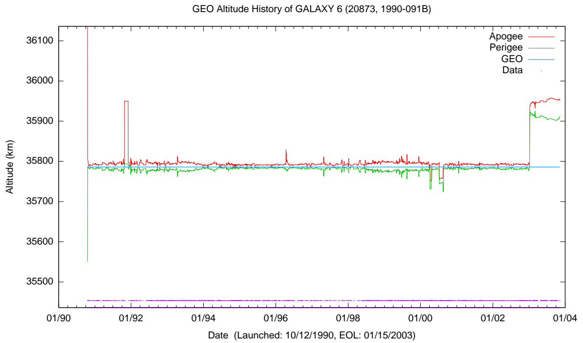
Figure E.1: Sample Satellite Geosynchronous Altitude History Plot
