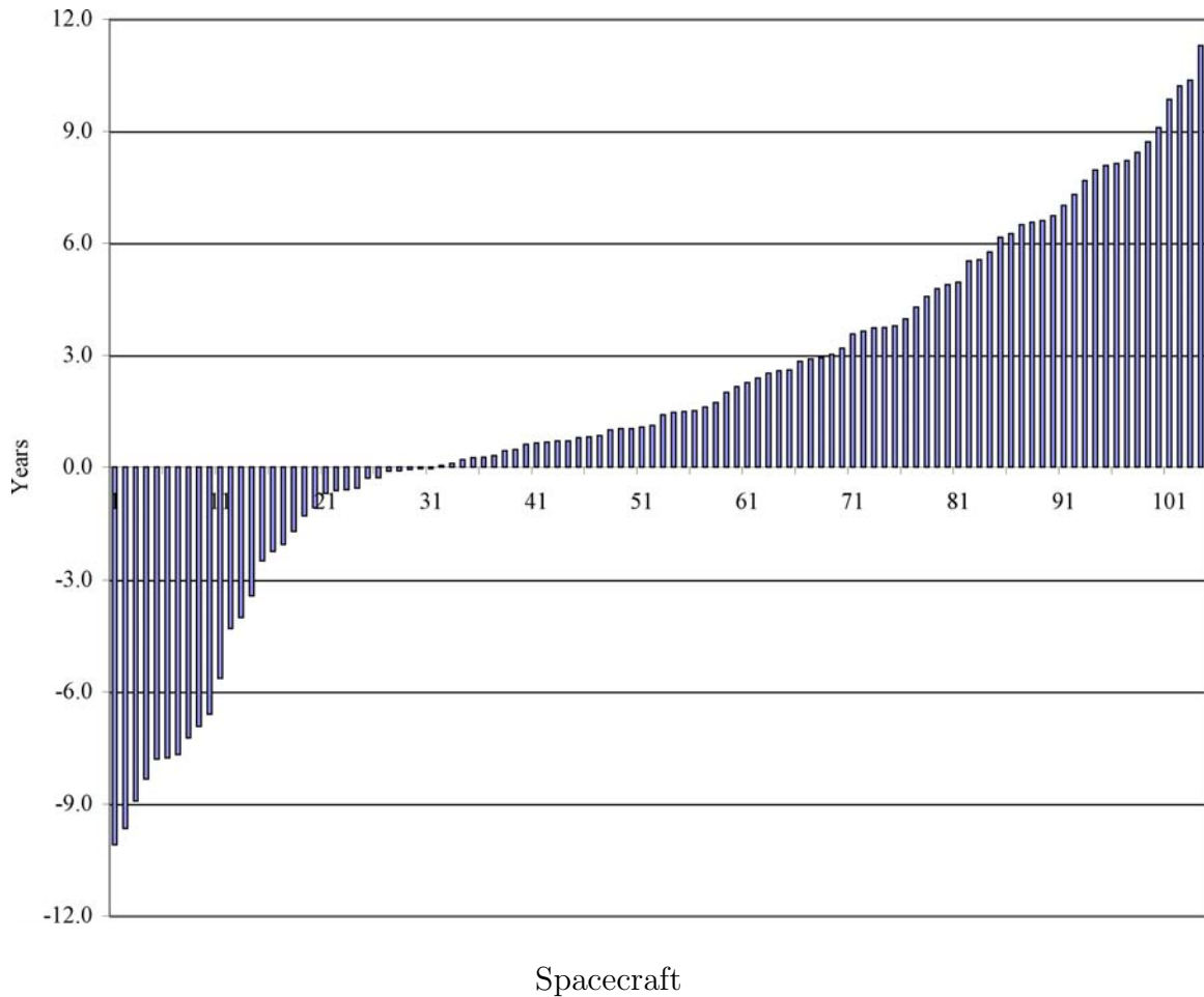
Figure 7.23: Years Actual Life Exceeded Design Life For Retired Geosynchronous Communications Satellites Launched Since 1980
