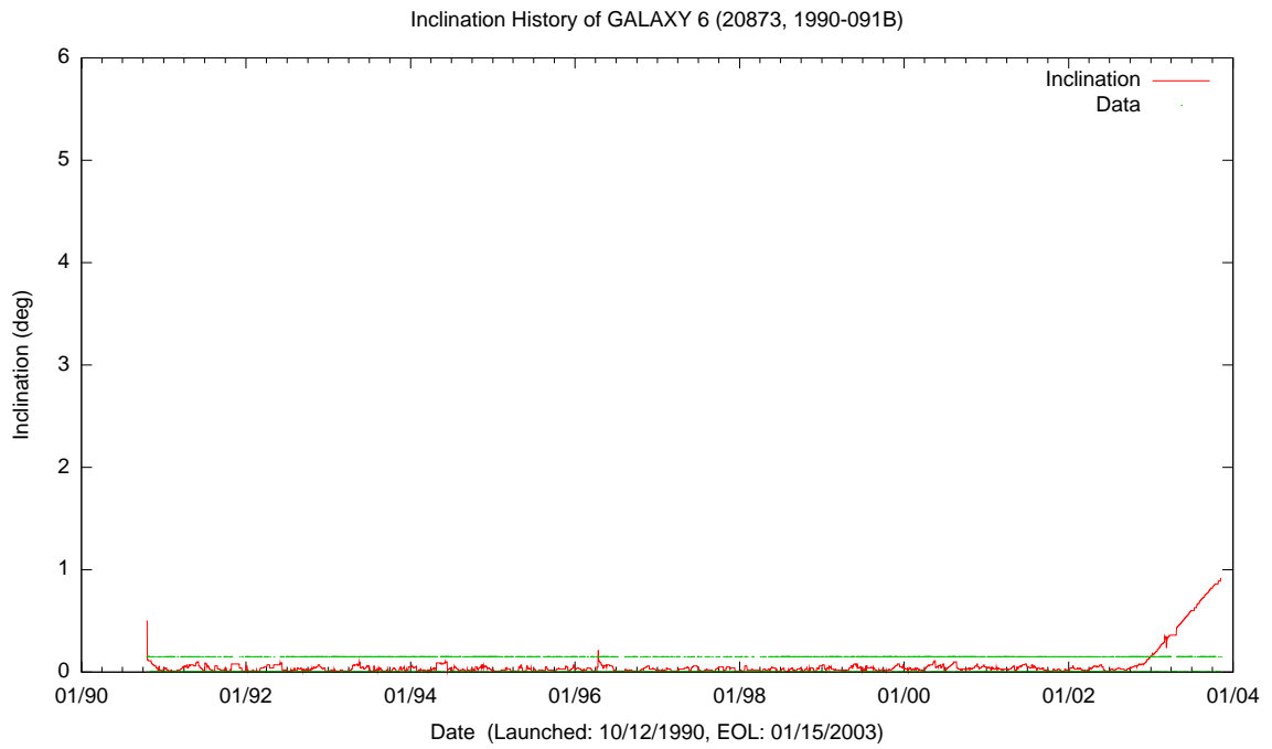
Figure E.2: Sample Satellite Inclination History Plot
