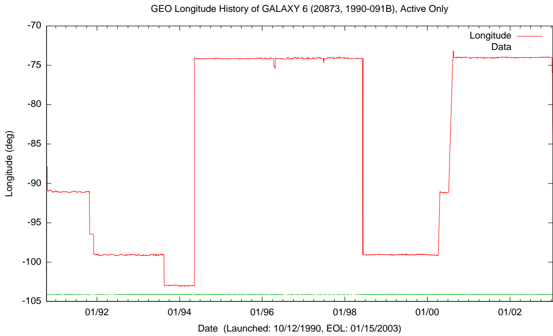
Figure E.4: Sample Satellite Geosynchronous Longitude History Plot, Active Life
