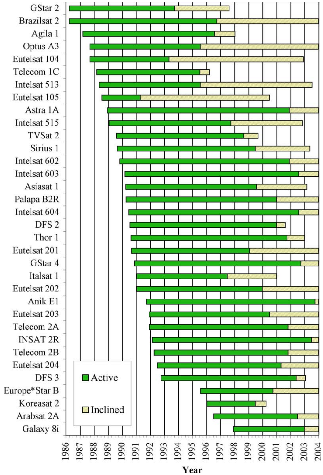
Figure A.19: Lifetimes Of Inclined Commercial Communications Satellites Launched From 1986 Onwards
