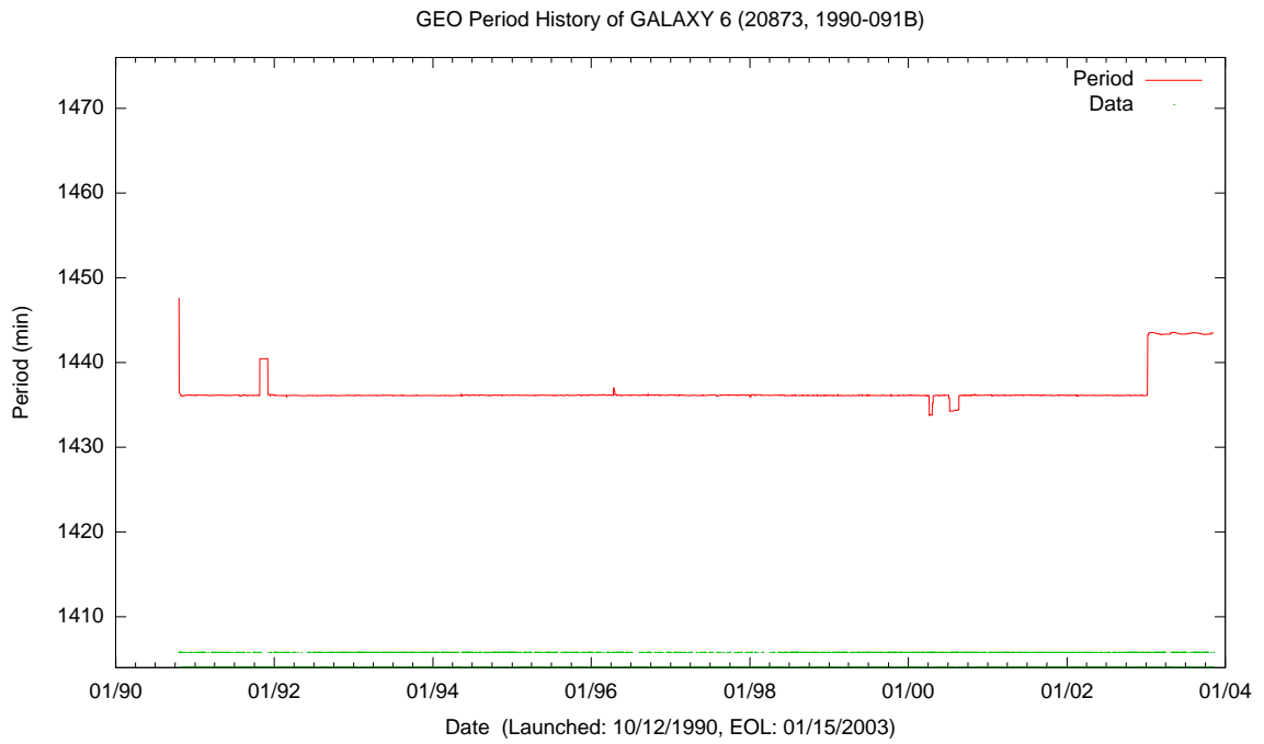
Figure E.6: Sample Satellite Geosynchronous Period History Plot
