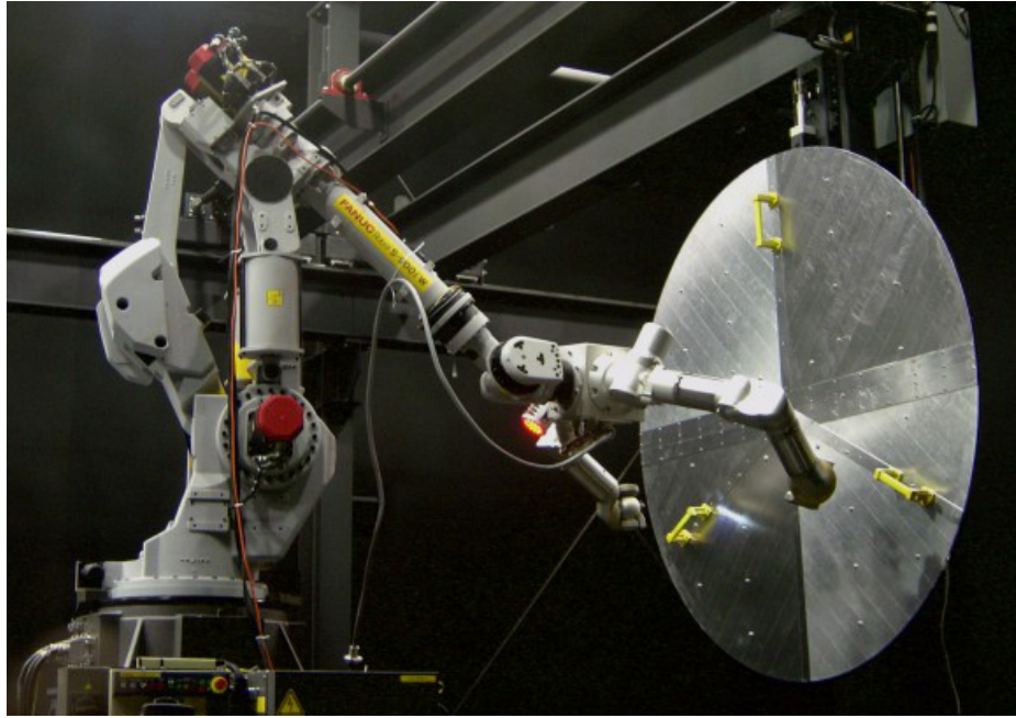
Figure 2.5: Ranger TSX Prepares To Dock With A Simulated Spacecraft [34]
