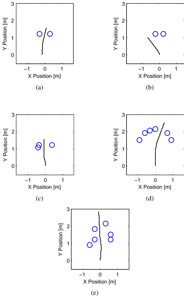
Fig. 7. Five experimental runs using the robotic platform. 7a: Robot can safely fit through obstacles. 7b: Robot correctly determines that the gap is too narrow and moves towards the outside. 7c: Additional obstacles do not affect Openspace . 7d: Robot finds and travels through the largest gap. 7e: Robot maneuvers random obstacle field
