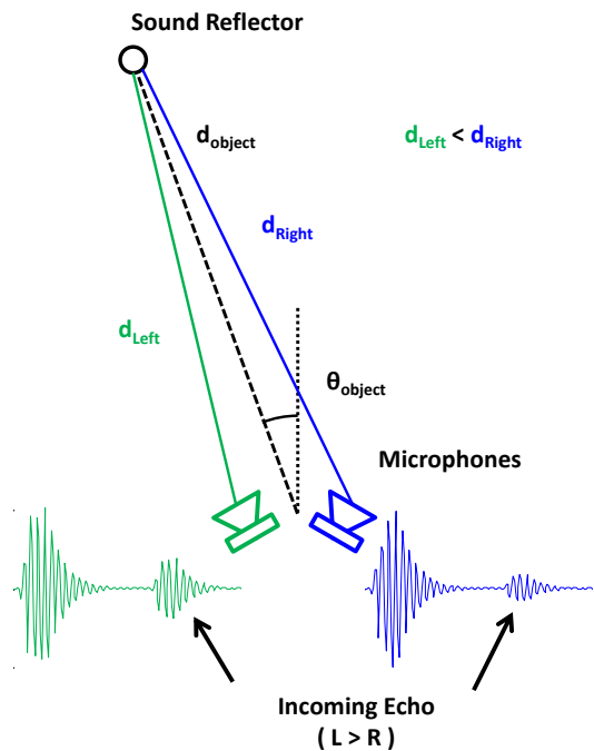
Fig. 1. Visualization of properties of the binaural sonar system which result in sound localization cues.
