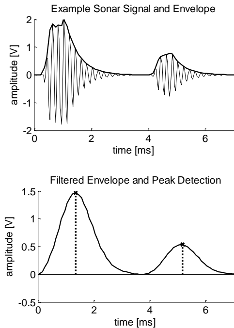
Fig. 2. Demonstration of signal processing on sample sonar signal. The sonar board detects the envelope of the signal using an Op-Amp based circuit. This is sent to MATLAB for filtering and peak detection for object detection.
