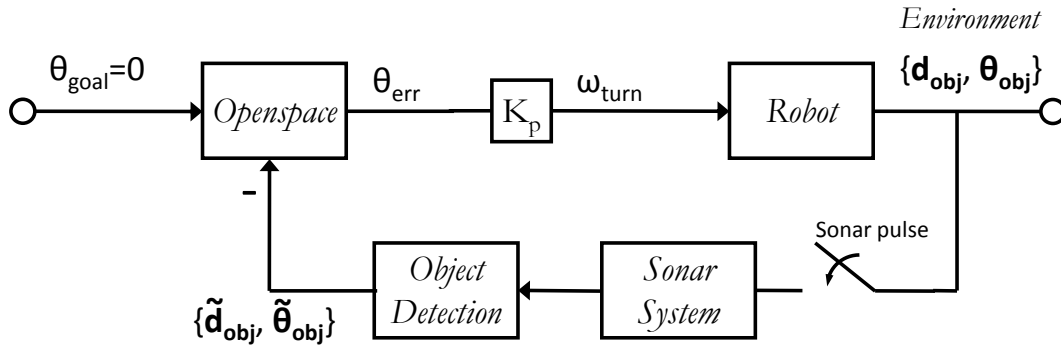
Fig. 6. System overview demonstrating the relation of the P Controller to the rest of the system. Note that the system is sampled due to active sonar, and an approximation of object locations is used in Openspace .
