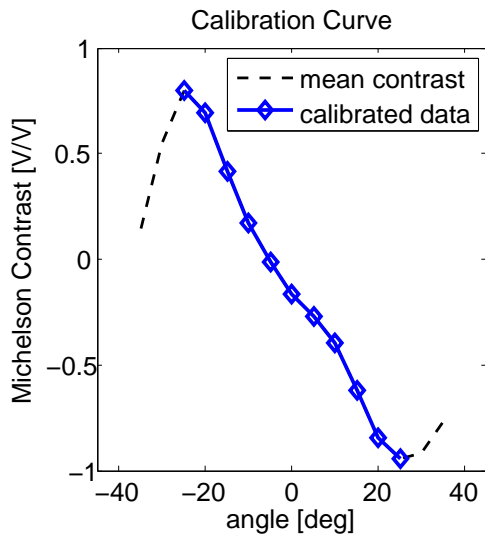
Fig. 3. Calibration data mapping Michelson Contrast values to angles. Only the region of monotonicity can be calibrated, so the dashed portion of the curve is truncated for calibration
