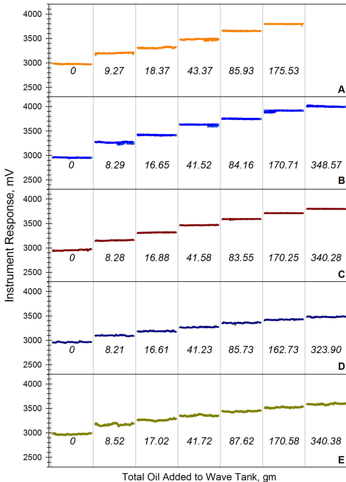
Figure 5. Time-series response of the CTG Aquatracka UV-HC to crude oil additions in the COOGER wave tank at the Bedford Institute of Oceanography, Bedford, NS. Instrument response reported over the 10 minute interval starting 40 minutes after addition of the indicated challenge compound level. Each tank trial was conducted as step-up oil additions to a fixed seawater parcel subject to mixing by breaking waves. Numeric legends indicate cumulative grams of corresponding crude oil added to test tank. (A) Arabian Light Crude (ALC, 7% weathered) + Corexit 9500 at a detergent to oil ratio (DOR) of 1:25. (B) Alaskan North Slope (ANS) DOR 1:25. (C) ALC, DOR 1:25. (D) ALC, DOR 0. (E) ANS, DOR 0.
