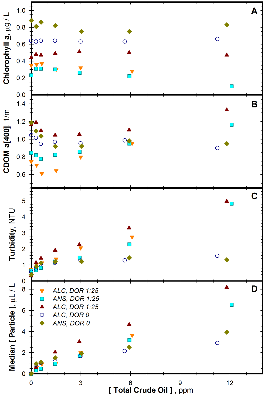
Figure 8. Variation of ancillary water quality parameters with crude oil additions during the COOGER trials. (A) Extracted chlorophyll a . (B) Absorbance at 400 nm as a proxy for CDOM. (C) Turbidity measured with a Hach 2100 AN. (D) Median particle concentration measured in situ using a LISST (Sequoia Inst).
