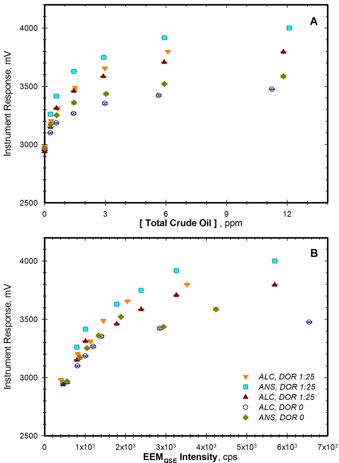
Figure 7. Response of CTG Aquatracka UV-HC to total crude oil concentration in presence/absence of the chemical dispersant Corexit 9500. All exposures experienced breaking waves. Reported measurements represent the average ( \pm S.D.) instrument response over 10 minute windows starting 40 minutes after addition of the challenge compound derived from data in Fig. 5. (A) Instrument response to total oil concentration (ppm) in Bedford Basin seawater (B) Relationship of instrument response to predicted EEM QSE based on instrument's optical window. EEMs not corrected for seawater background.
