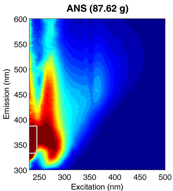
Figure 6. Representative EEMs for crude oil treatments during the COOGER trials. Grey boxes represent the CTG Aquatracka UV-HC optical window used for estimation of integrated fluorescent intensities.
