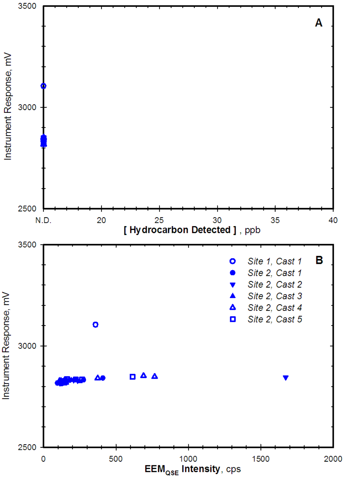
Figure 16. Response of the CTG Aquatracka UV-HC to ambient hydrocarbons and water fluorescence properties at the Gulf of Mexico hydrocast sites. (A) Instrument response to TPH detected by GC-FID, no TPH reported for this same batch. (B) Instrument response to predicted EEMs fluorescent intensity. Scale has been expanded relative to other figures to help reveal instrument response in this environment.
