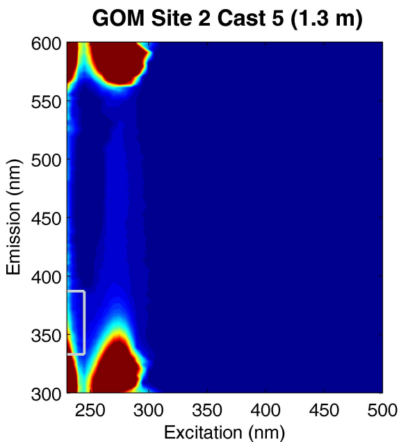
Figure 15. Representative EEMs for Gulf of Mexico hydrocast samples with the optical window for the CTG Aquatracka UV-HC represented by the grey outline box. No petroleum hydrocarbons were detected by GC-FID.
