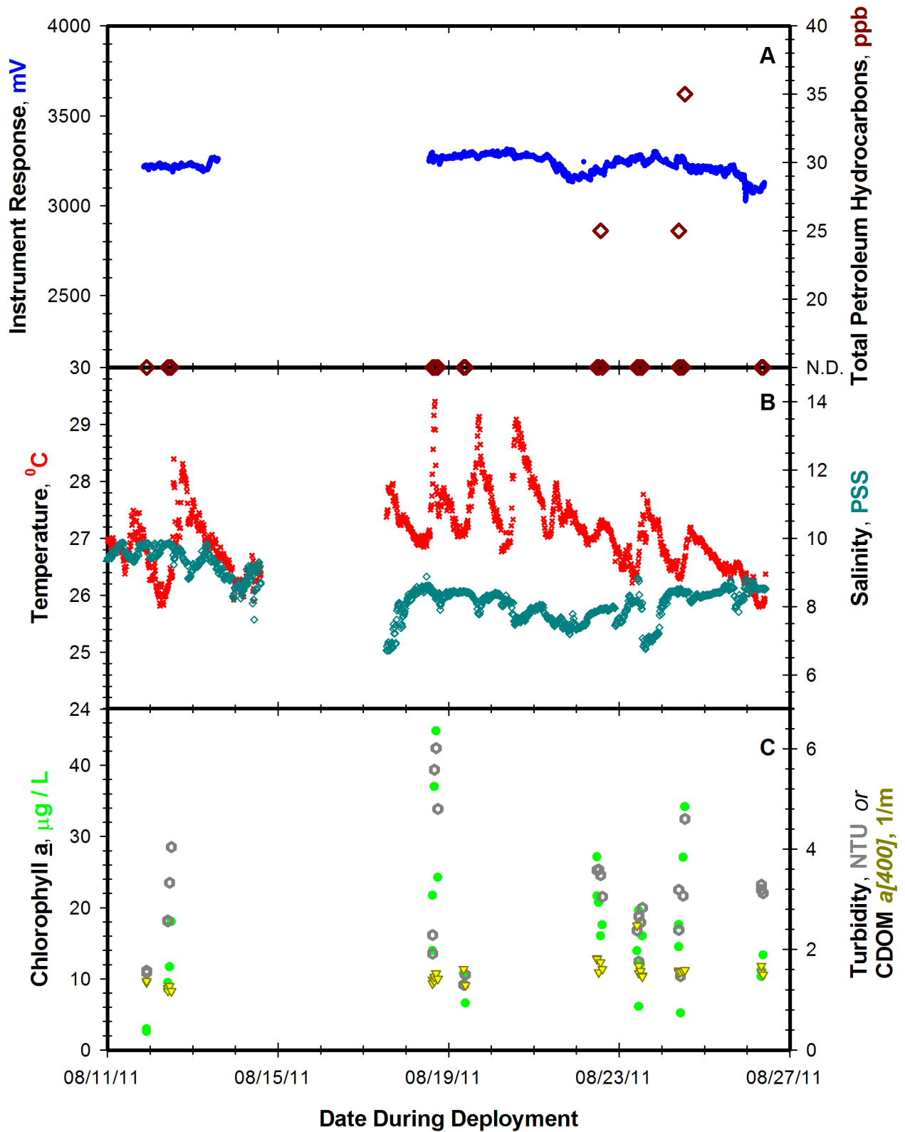
Figure 9. Summary of field deployment results for the CTG Aquatracka UV-HC at the MERC facility in Baltimore, MD. (A) Instrument time series response during deployment along with GC-FID measurements of total petroleum hydrocarbons (TPH, Test America- Sacramento) in grab samples taken at the time of instrument sampling. (B) Variation in temperature and salinity at the deployment site measured by a YSI 6600 sonde. (C) Variation in Chlorophyll a , turbidity and CDOM determined from grab samples taken adjacent to the instruments during deployment.
