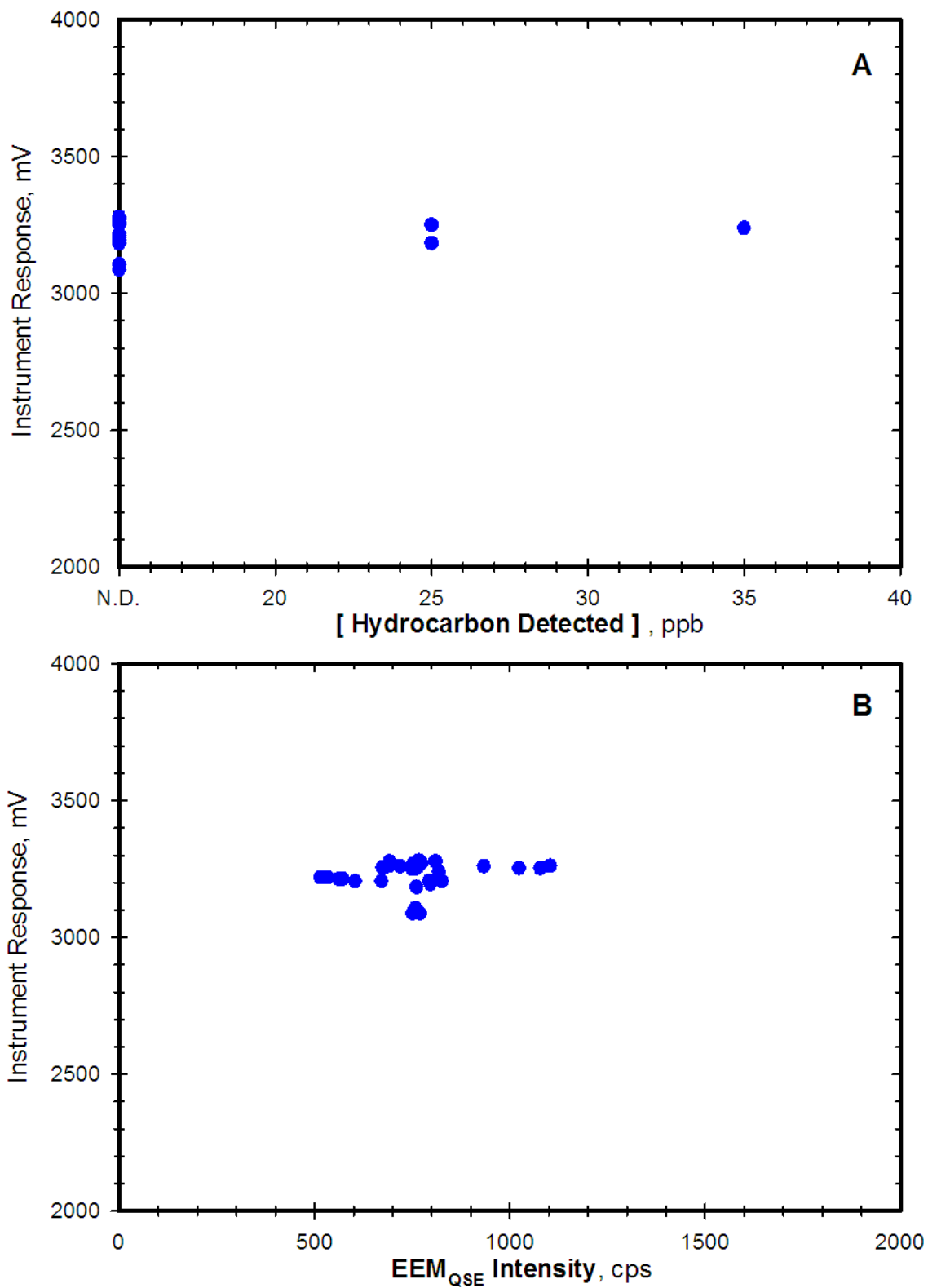
Figure 11. Response of CTG Aquatracka UV-HC to ambient hydrocarbons and water fluorescence properties during the Baltimore Harbor deployment. (A) Instrument response to TPH detected by GC-FID. (B) Instrument response to predicted EEMs fluorescent intensity.
