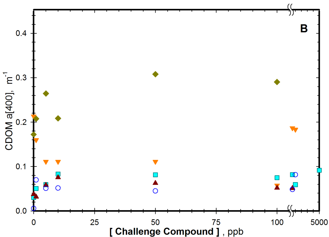
Figure 4. Variation in Turbidity and CDOM measurements with respect to challenge compound and challenge concentration during laboratory trials. (A) Turbidity (NTU) measured with a calibrated Hach 2100 AN. (B) Relative CDOM (chromophoric dissolved organic matter) concentration estimated as the absorbance at 400 nm, predicted from an exponential fit of sample absorbance spectra over 400-600 nm as described in text.
