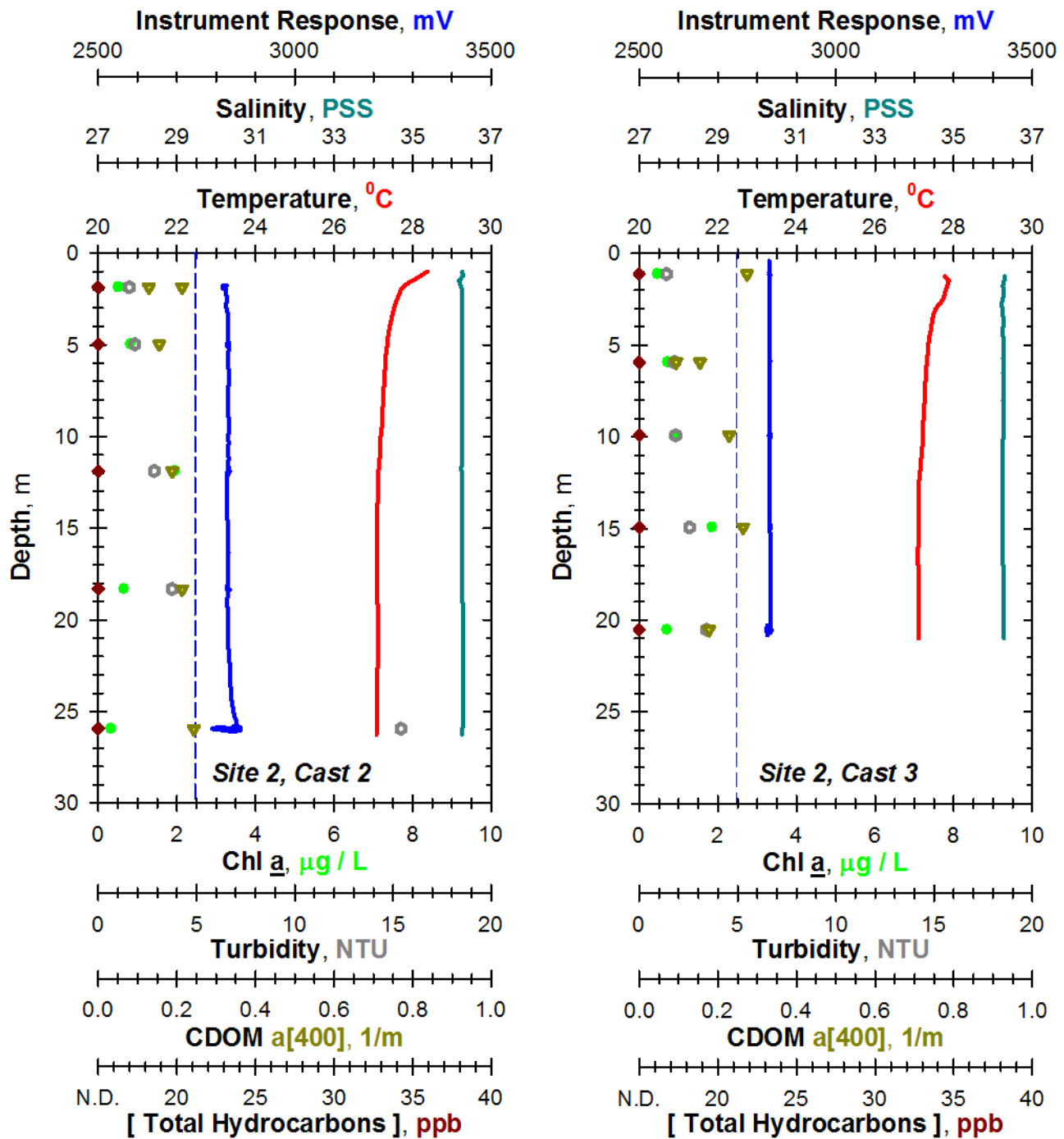
Figure 13. Gulf of Mexico hydrocast profiles from the CTG Aquatracka UV-HC, Site 2, Cast 2 and Cast 3. Left panel: Cast 2; Inside slick from oil barge (28.34.075N, 90.58.738W). Right panel: Cast 3; Inside plume near submerged barge (28.34.049N, 90.58.878W). Refer to Fig. 12 for details.
