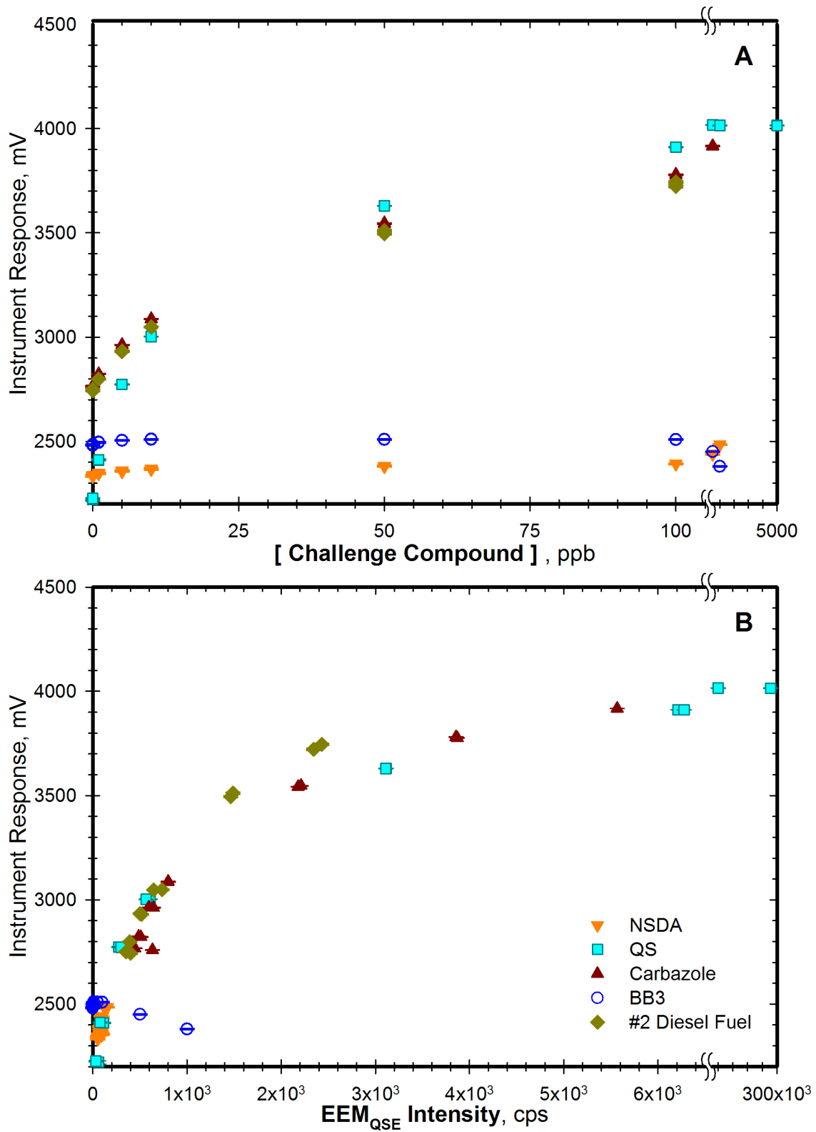
Figure 3. Response of CTG Aquatracka UV CDOM and HC to challenge compound additions. Reported measurements represent the average ( \pm S.D.) instrument response over 10 minute windows starting 30 minutes after addition of the challenge compound in de-ionized water. Scaling changes to 1000 ppb per tick after axis break. (A) Instrument response to concentration of challenge compound in de-ionized water. Scaling changes to 1000 ppb per tick after axis break. (B) Relationship of instrument response to predicted EEM QSE based on instruments specified optical window. Scaling changes to 50,000 cps per tick after axis break. Note also that the CTG Aquatracka UV-HC model used during #2 Diesel Fuel trial.
