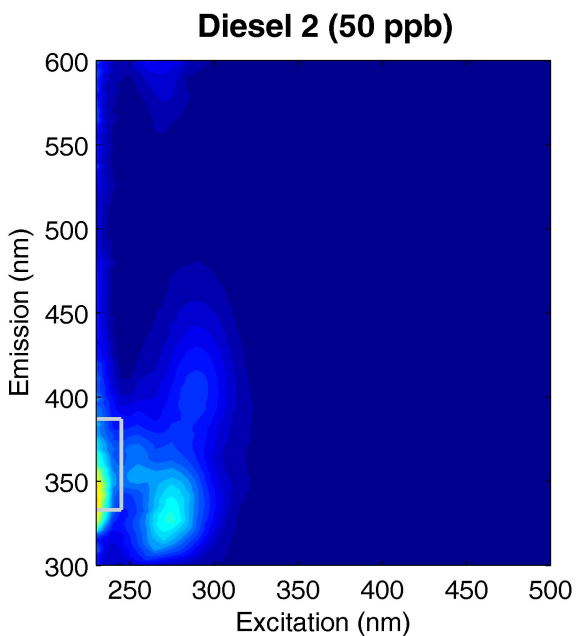
Figure 2. The CTG Aquatracka UV-HC optical window mapped onto EEMs of lab challenge compounds as in Fig. 1. This instrument was used during the diesel fuel challenge and in all subsequent evaluation trials.
