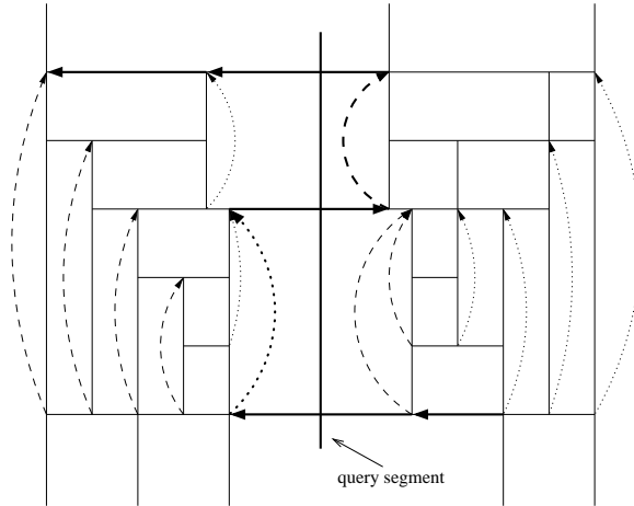
Figure 3: Modified hive graph.
