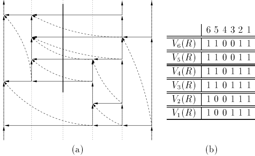
Figure 5: H(R) and M(R) .
