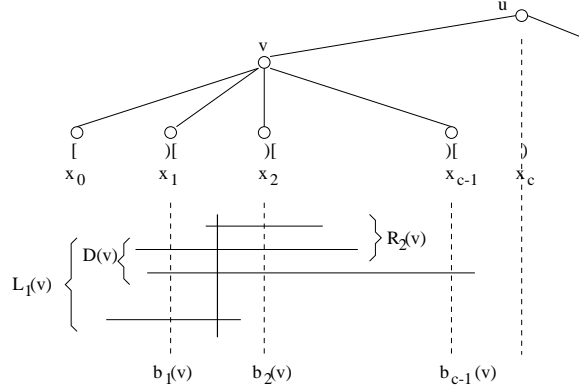
Figure 6: Data structures for the segments associated with node v .
