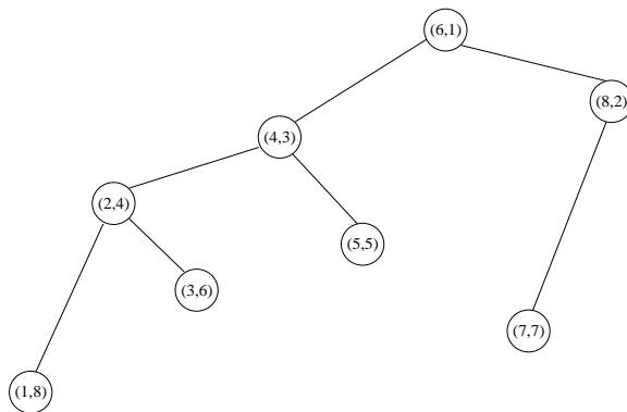
Figure 1: Cartesian tree.
