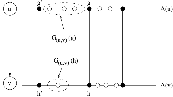
Figure 4: Fractional cascading.
