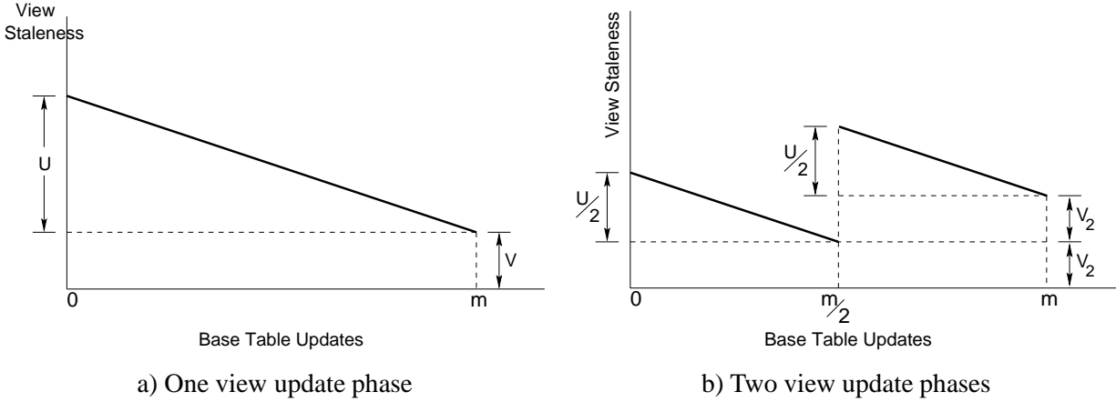
Figure 3: View staleness calculation
