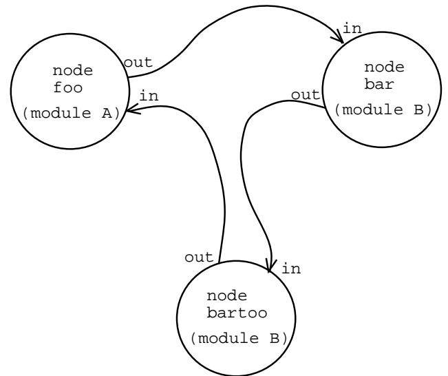
Figure 1.2: Information provided by the application's MIL program; module definitions (left); application definition (right).
