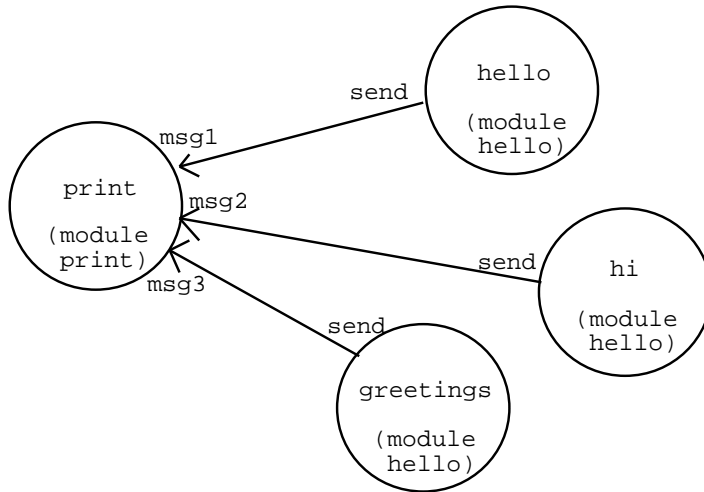
Figure 3.1: Basic application structure (used in first three examples).
