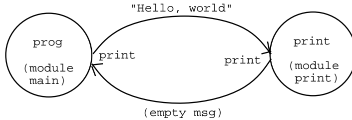
Figure 2.2: Hello1 , the POLYLITH version of simple Hello0 example.
